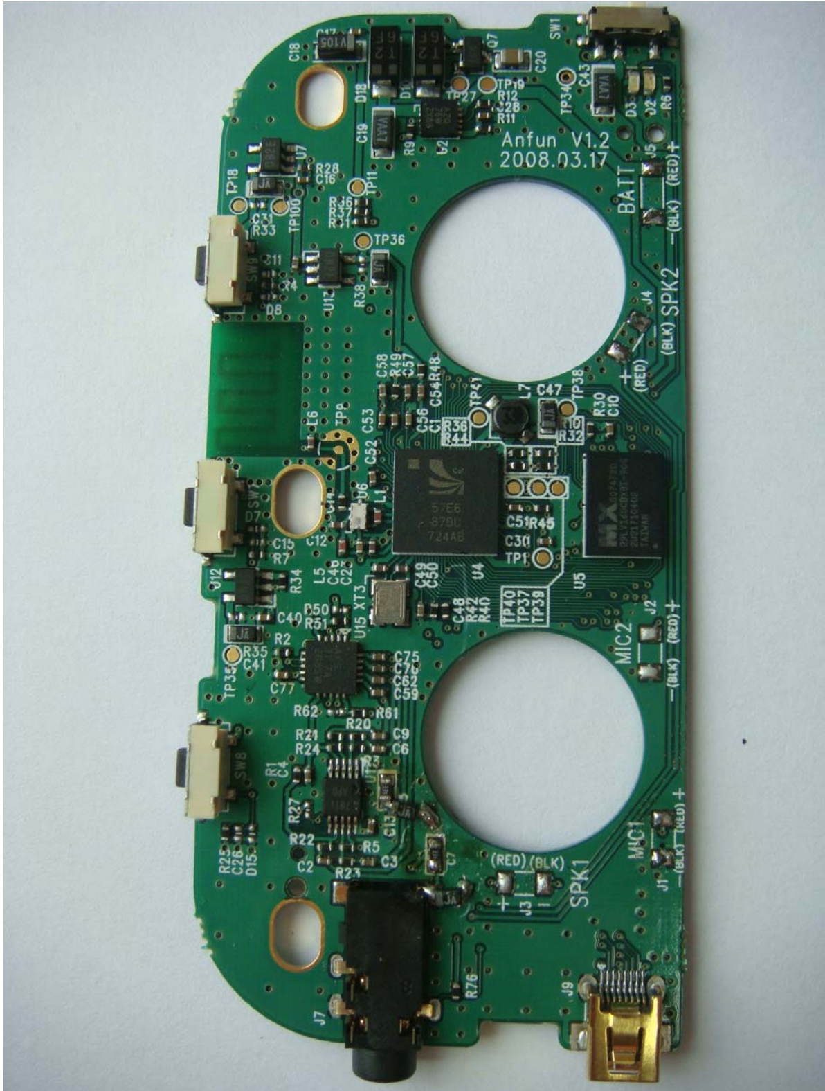
<Photograph 2: Internal Board_Front>
