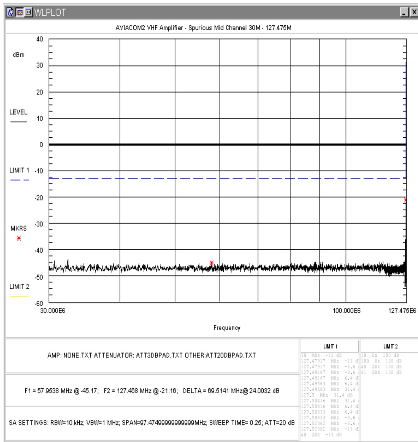
Figure 8. Conducted Spurious Emissions, Mid Channel Plot 1
