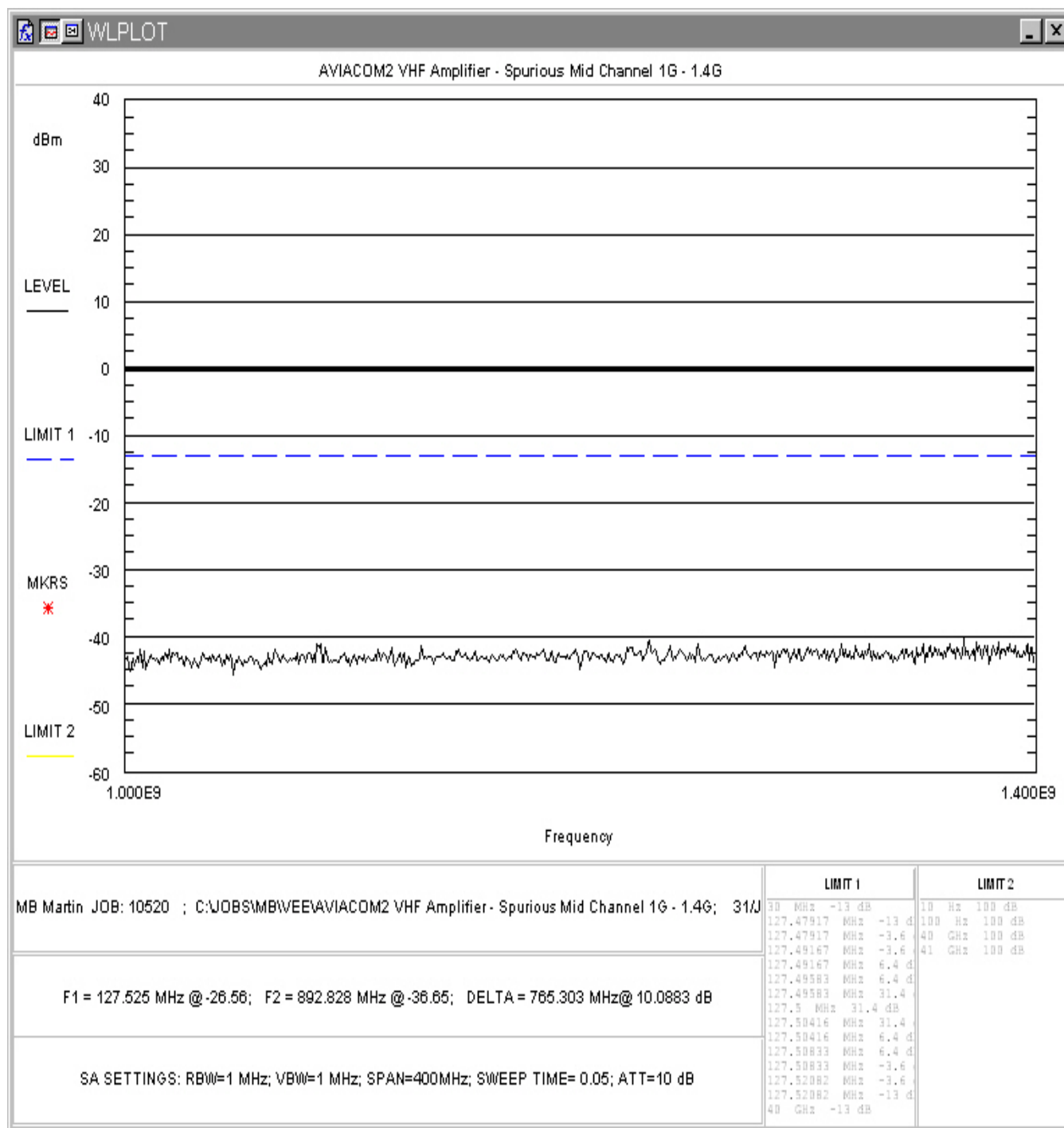
Figure 10. Conducted Spurious Emissions, Mid Channel Plot 3
