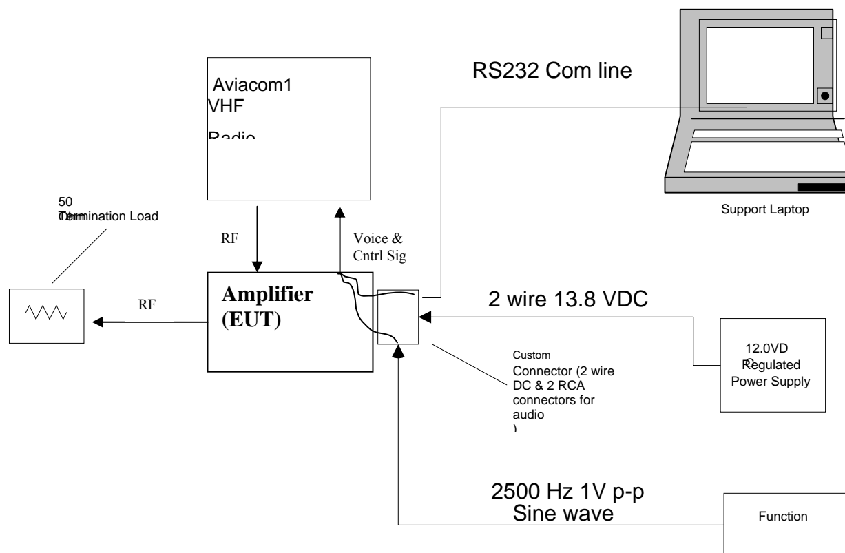
Figure 1. Test Configuration
