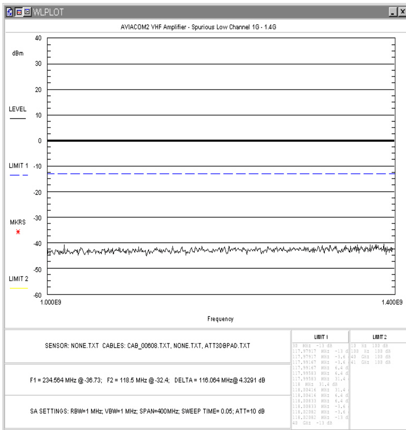
Figure 7. Conducted Spurious Emissions, Low Channel Plot 3
