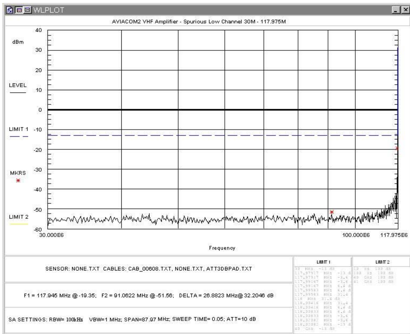
Figure 5. Conducted Spurious Emissions, Low Channel Plot 1
