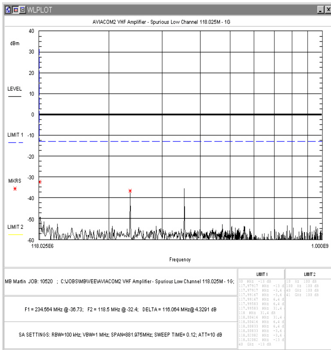
Figure 6. Conducted Spurious Emissions, Low Channel Plot 2
