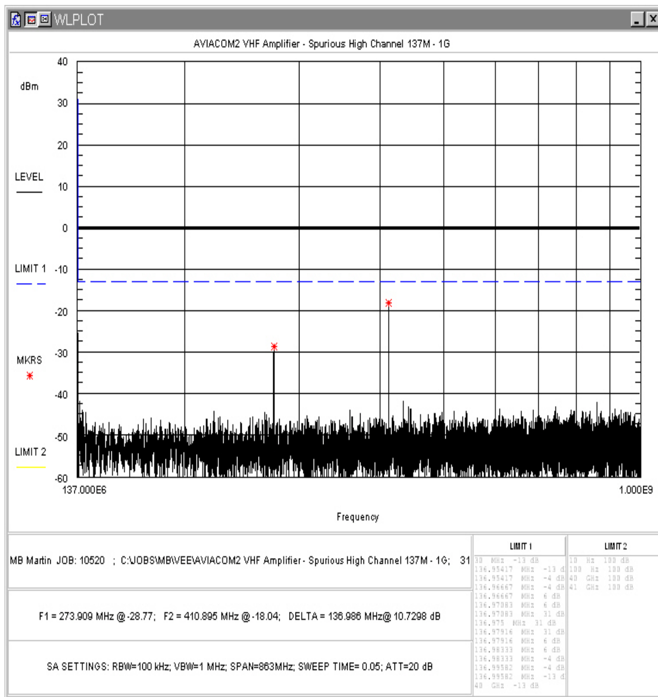
Figure 12. Conducted Spurious Emissions, High Channel Plot 2
