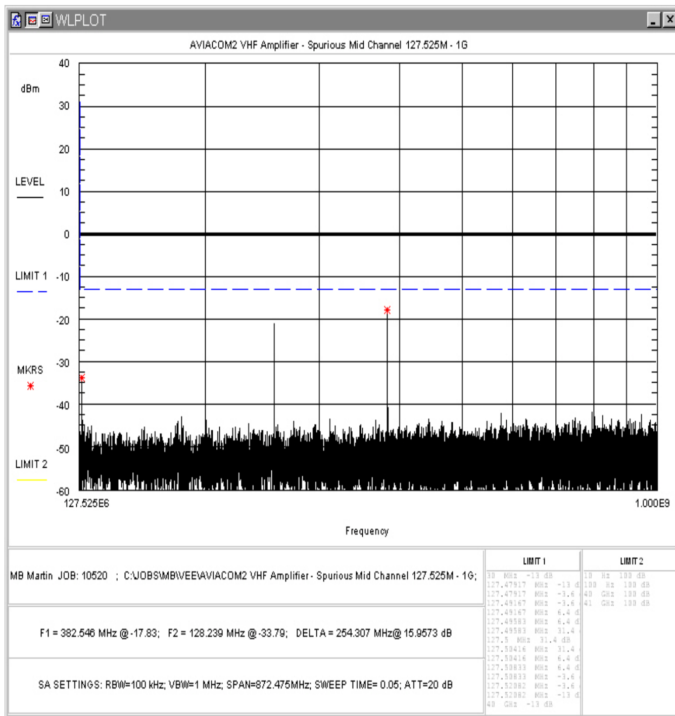
Figure 9. Conducted Spurious Emissions, Mid Channel Plot 2
