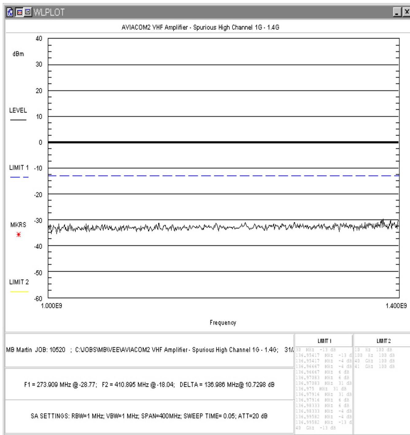
Figure 13. Conducted Spurious Emissions, High Channel Plot 3
