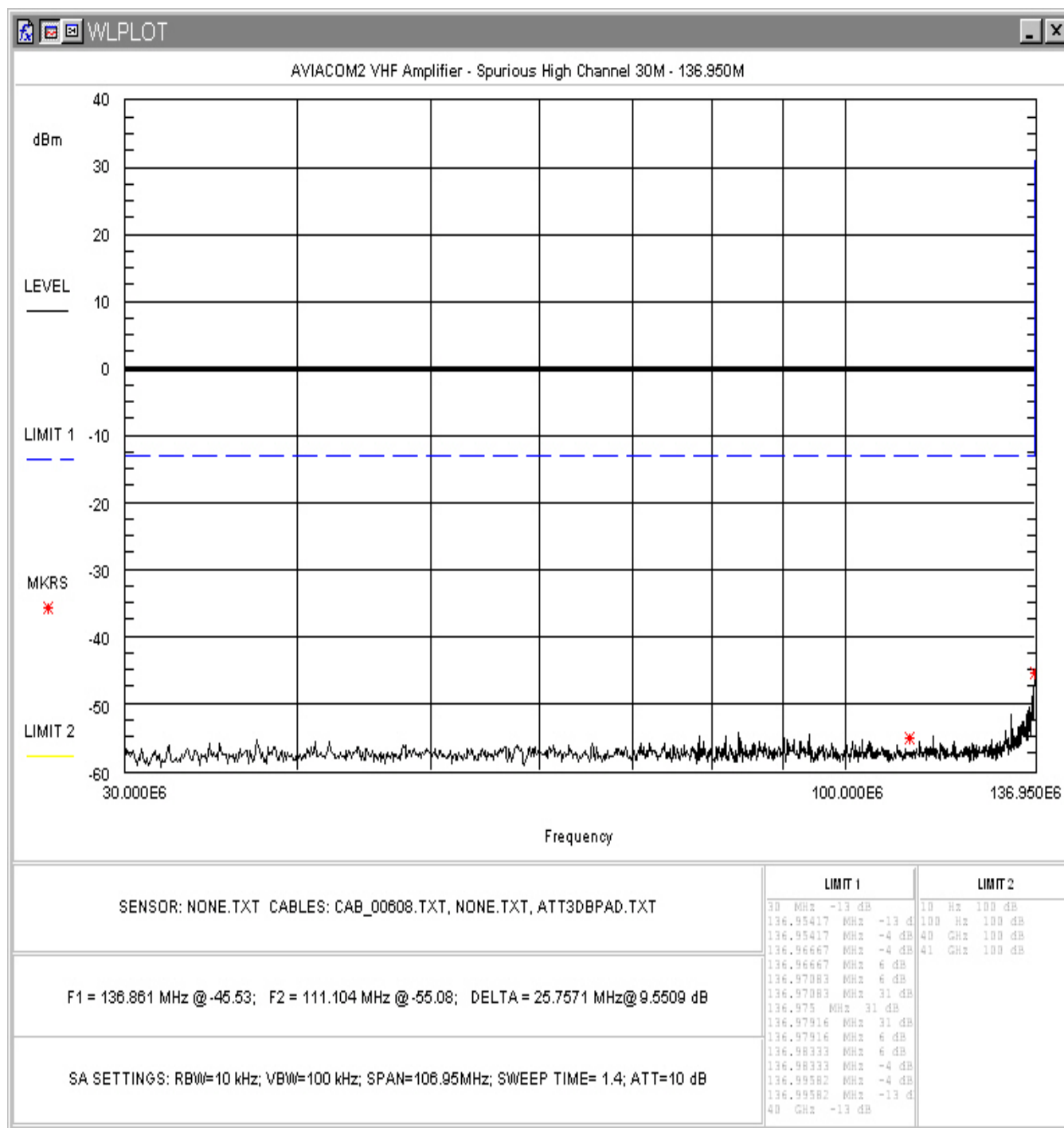
Figure 11. Conducted Spurious Emissions, High Channel Plot 1
