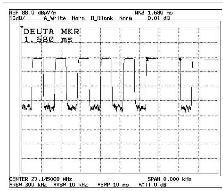
Duty Cycle 1
