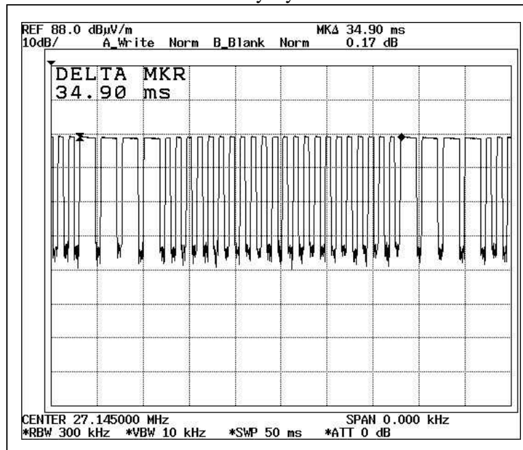
Duty Cycle
