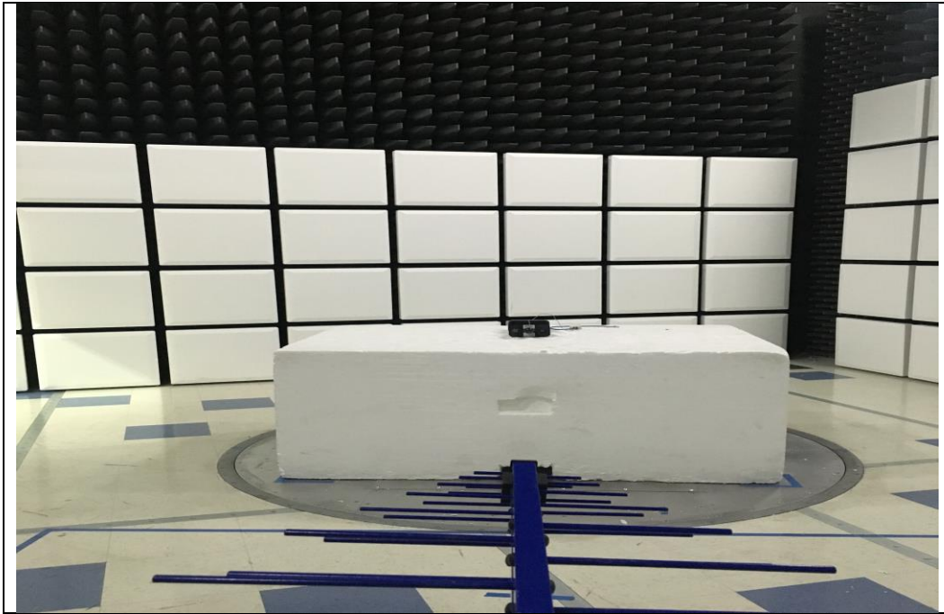
Radiated measurements 30 MHz- 1GHz
