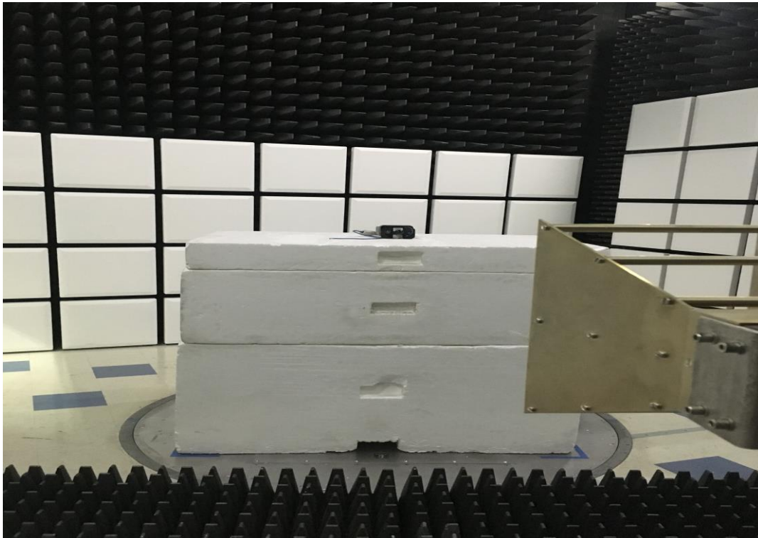
Radiated measurements 1-18GHz
