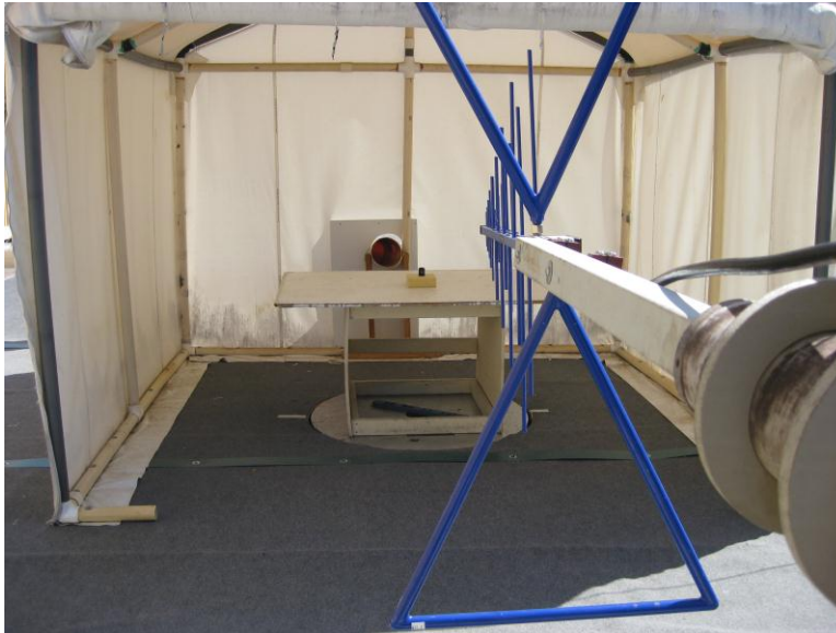
Radiated Emissions below 1 GHz - #2
