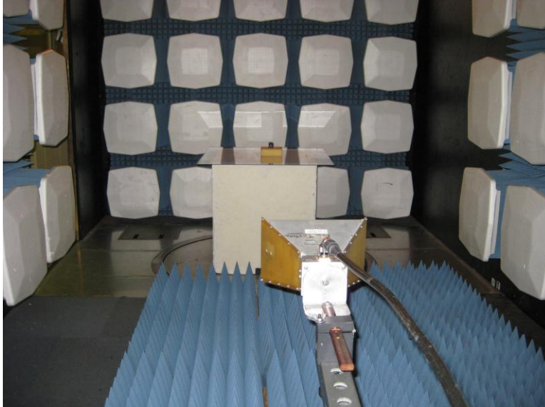
Radiated Emissions above 1 GHz - #1
