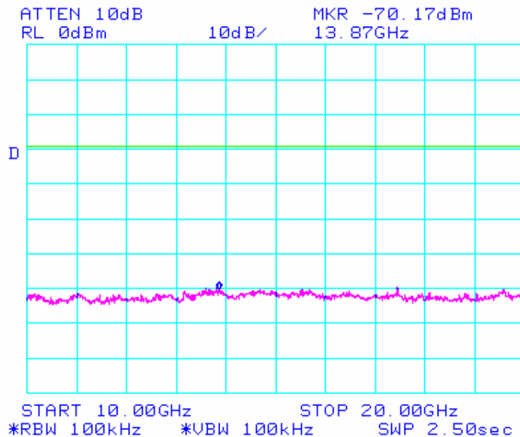
Plot 5: Conducted Spurious 3 of 3
