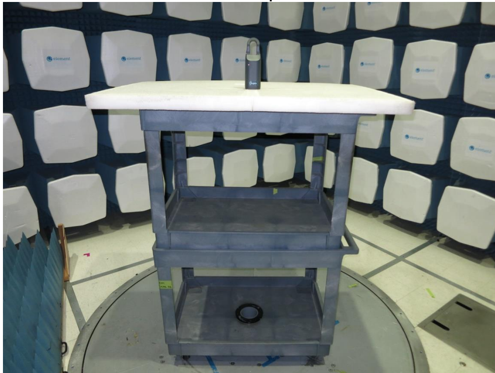
Radiated Spurious
