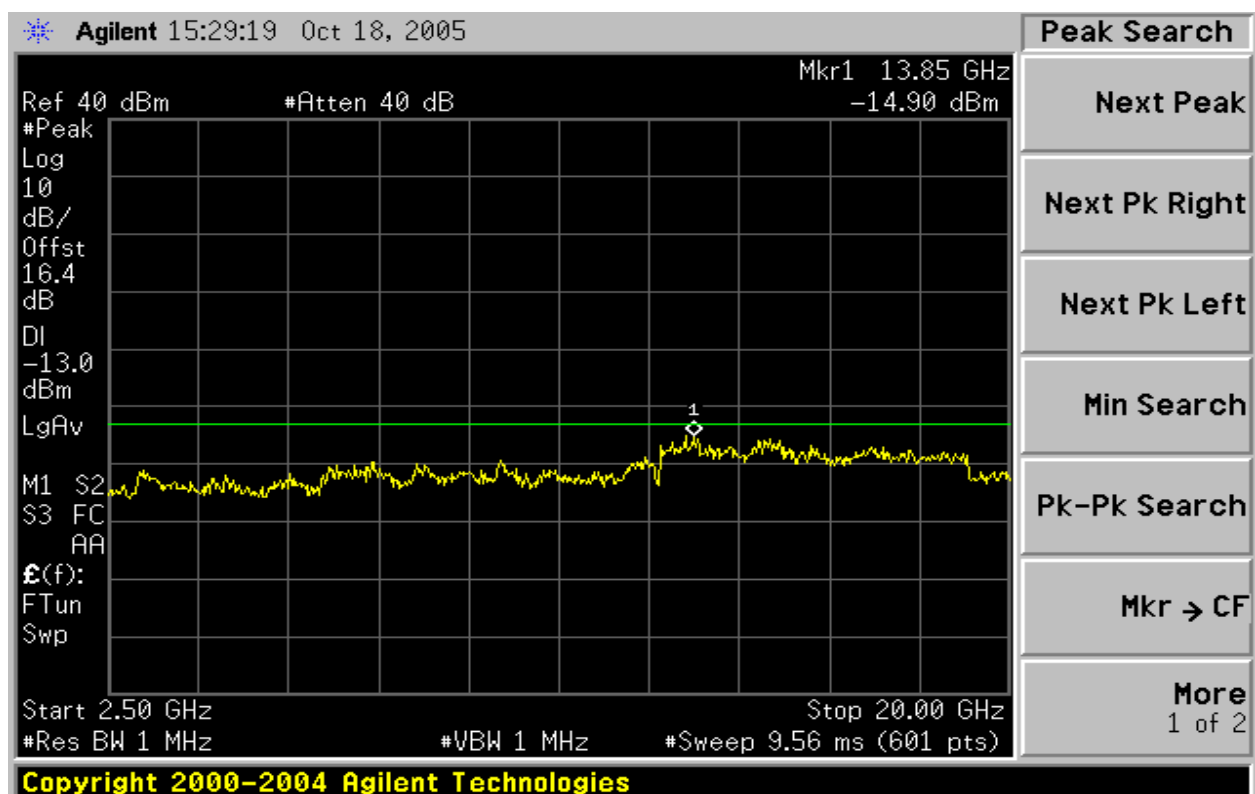
Figure2: Out of Band emission at antenna terminals – GSM CH Low
