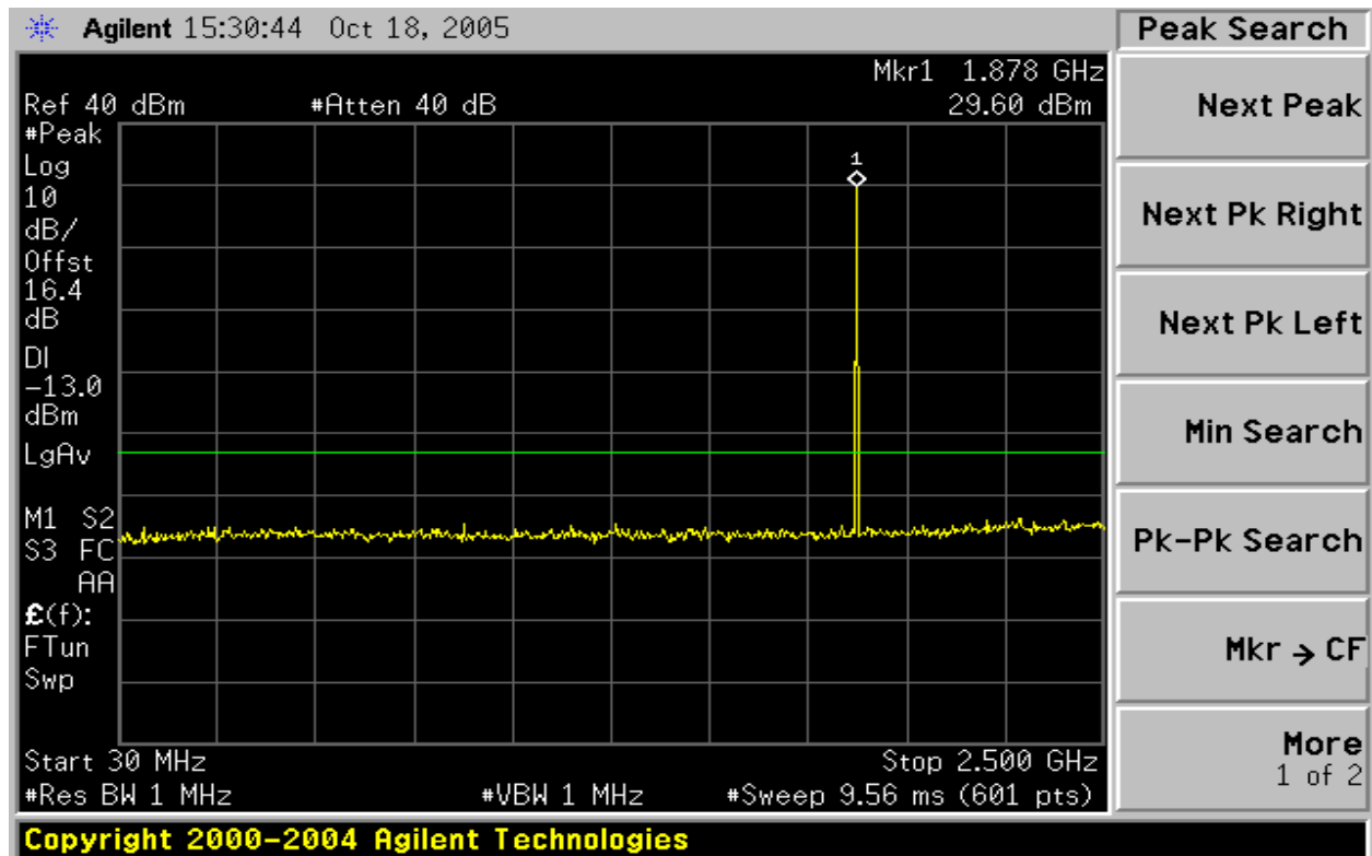
Figure3: Out of Band emission at antenna terminals – GSM CH Mid
