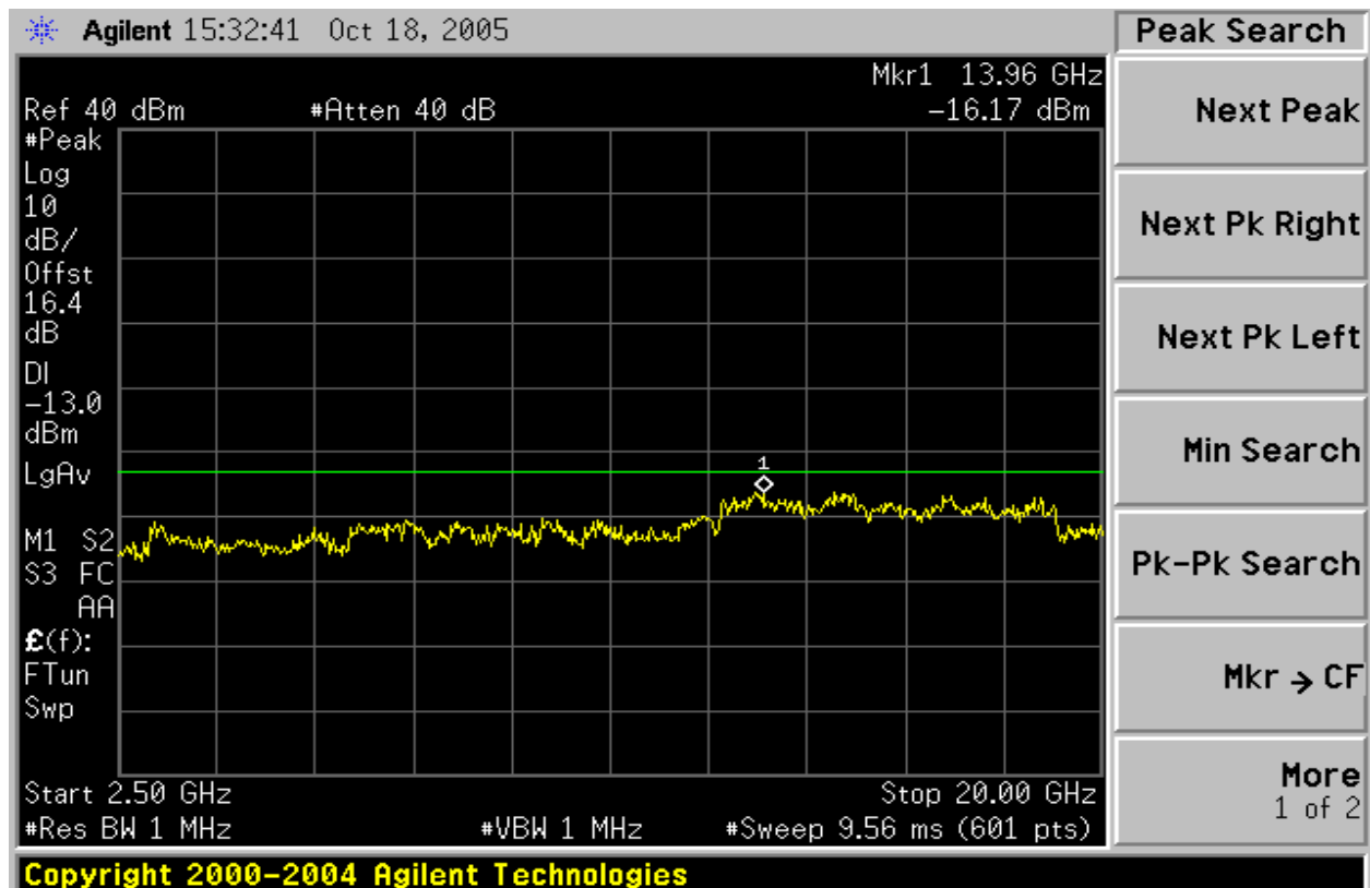
Figure 6: Out of Band emission at antenna terminals – GSM CH High
