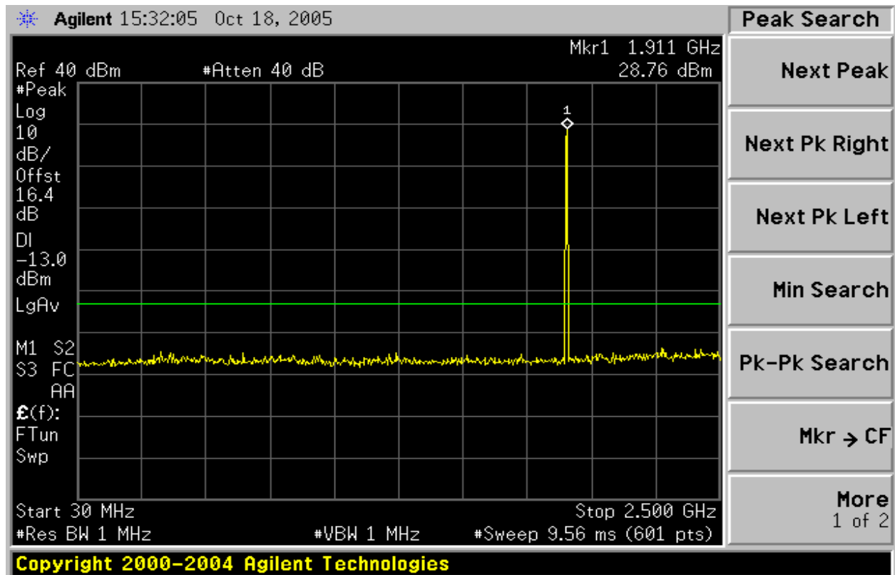
Figure5: Out of Band emission at antenna terminals – GSM CH High
