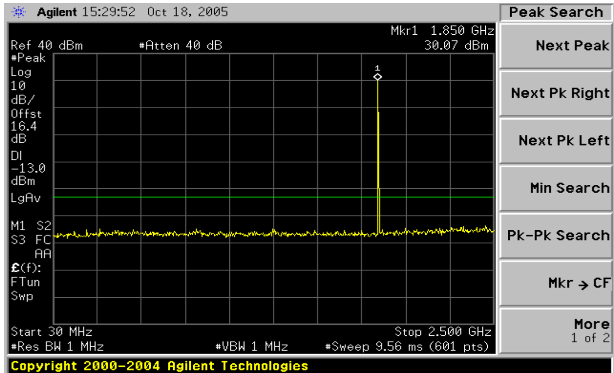
Figure 1: Out of Band emission at antenna terminals – GSM CH Low
