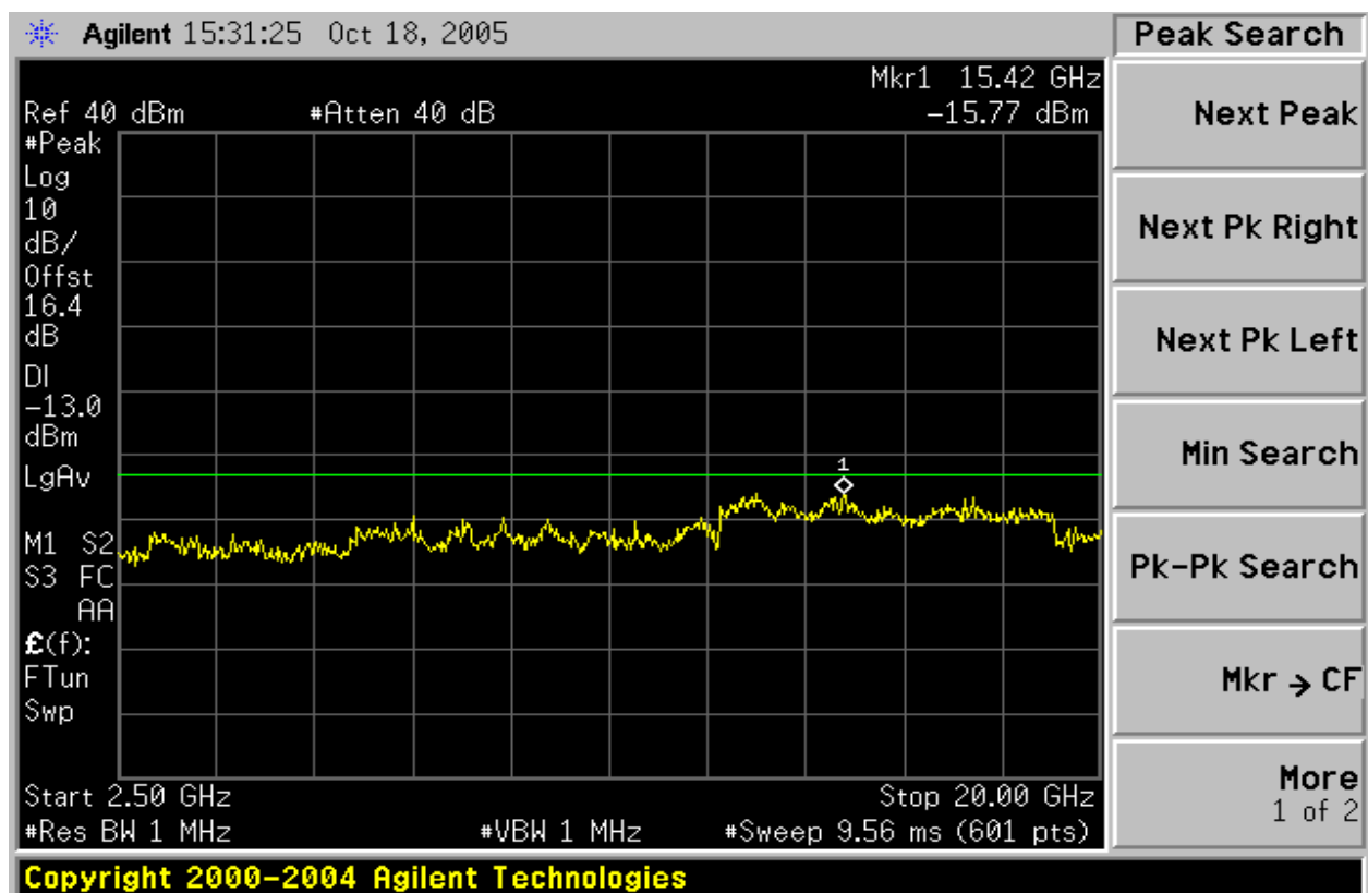
Figure4: Out of Band emission at antenna terminals – GSM CH Mid
