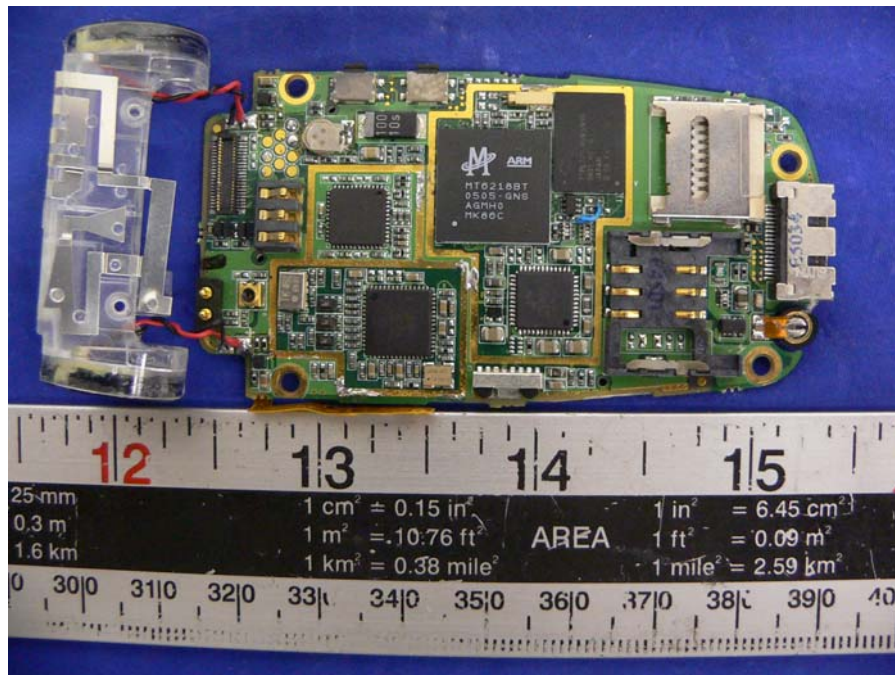
Main Board – Without Shielding View
