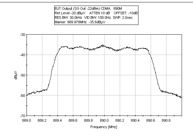
CDMA 890 MHz Output signal
