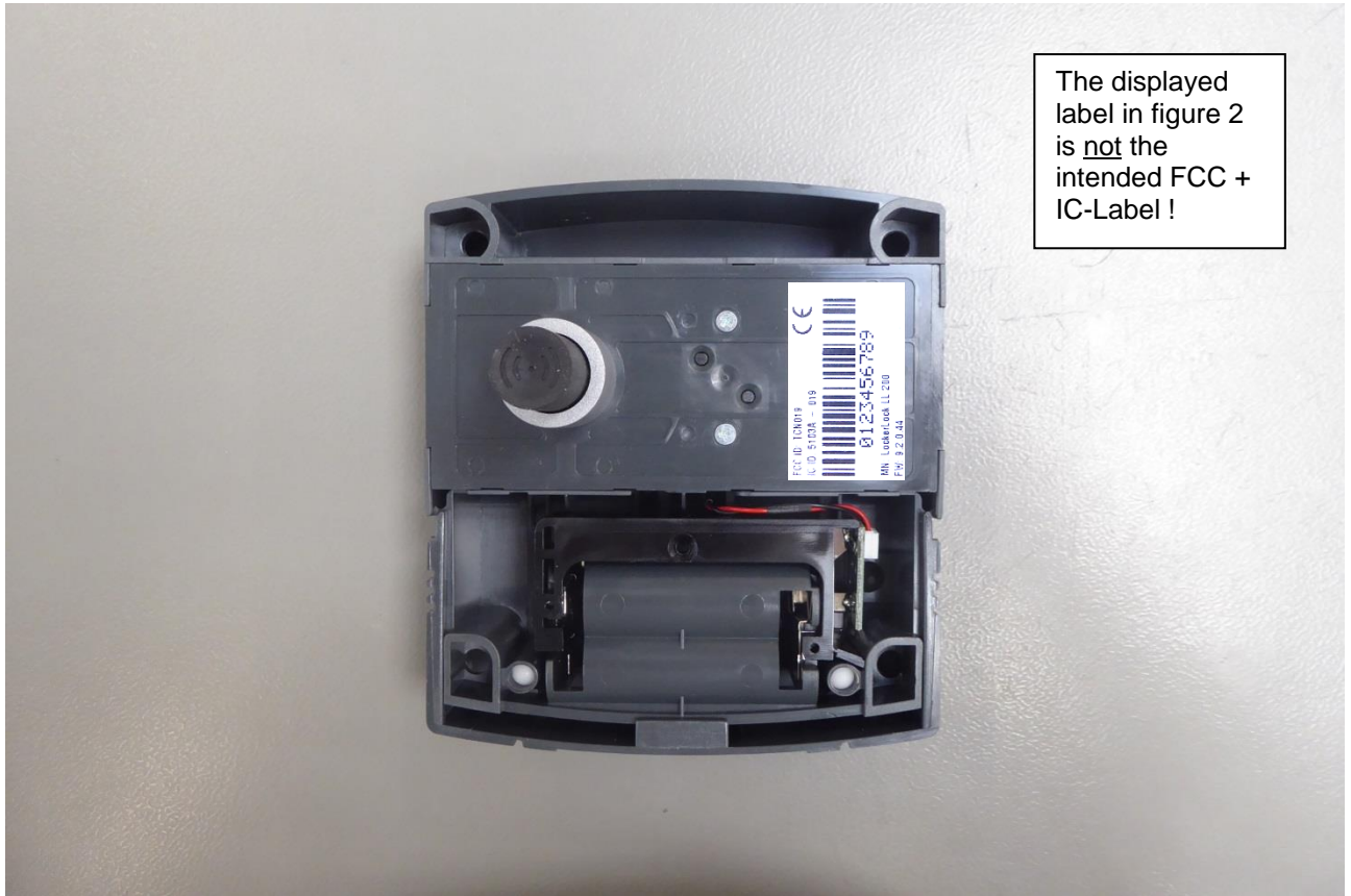
Figure 2 - Rear View
