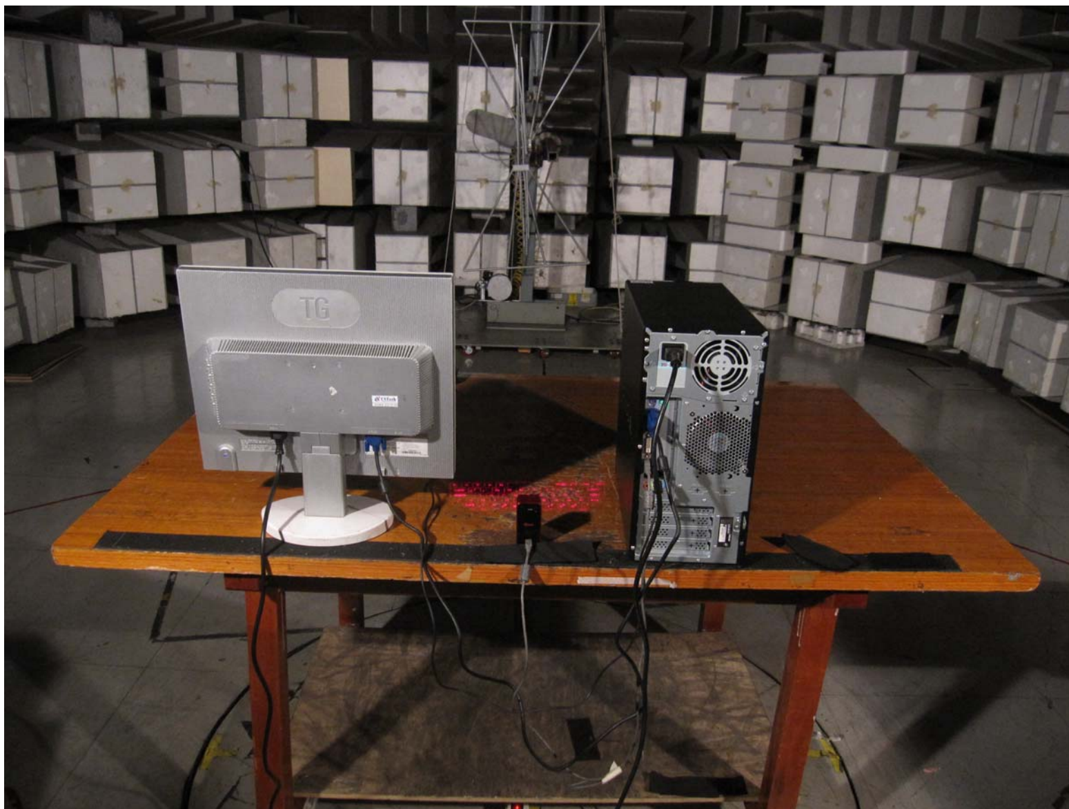
Magic Cube_Radiated Emission 30 MHz to 1 GHz (PC) Rear
