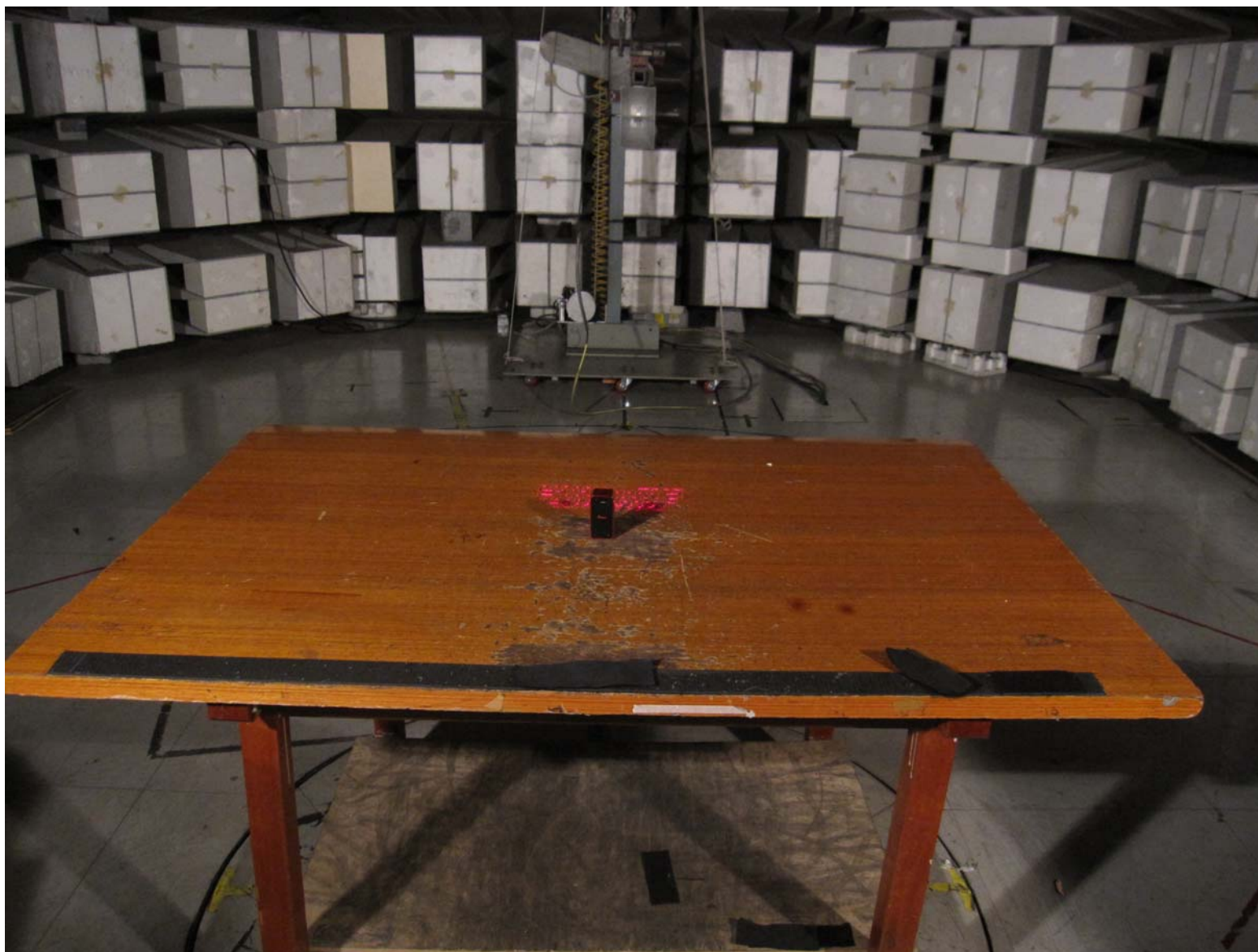
Magic Cube_Radiated Emission 1 GHz to 12.75 GHz Rear
