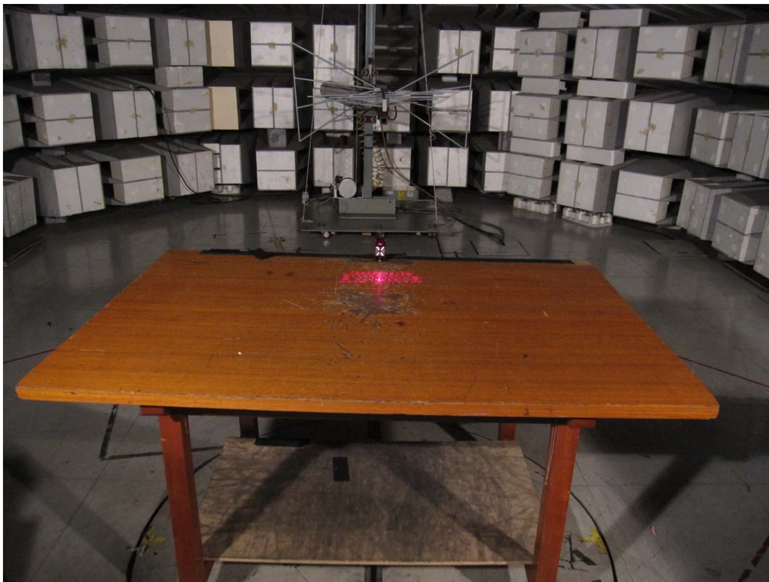
Magic Cube_Radiated Emission 30 MHz to 1 GHz (Portable) Front
