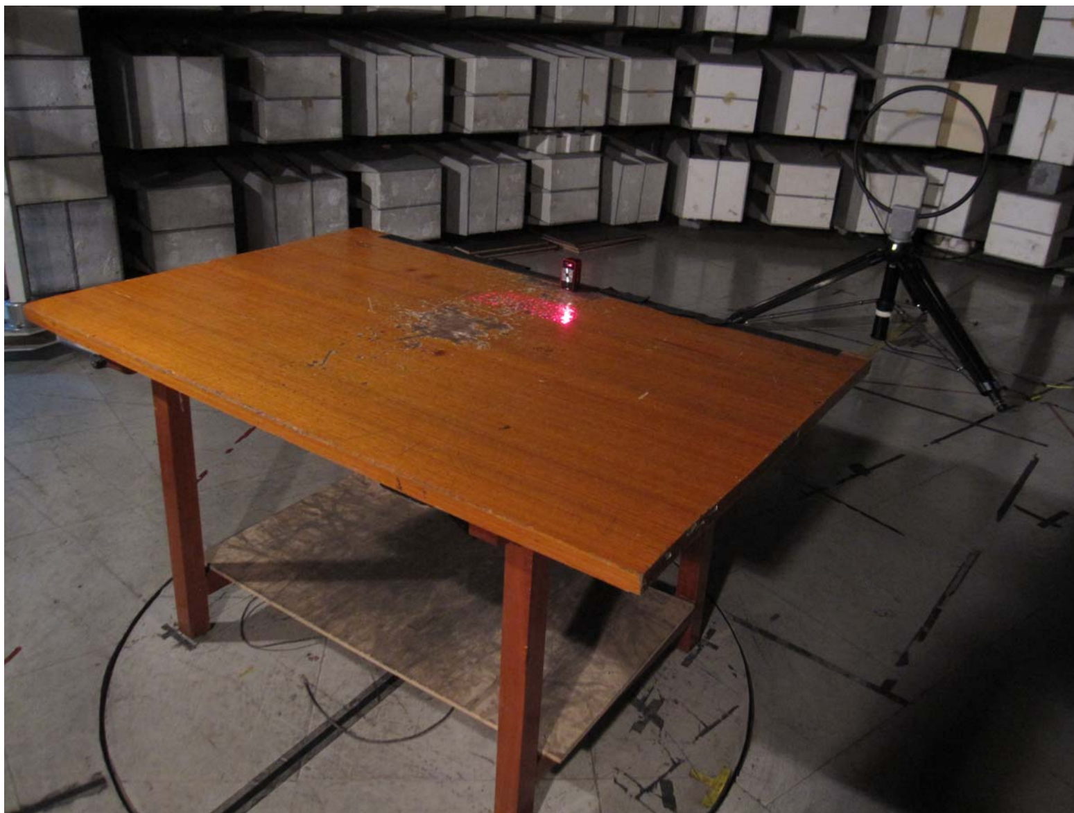
Magic Cube_Radiated Emission 9 kHz to 30 MHz (Portable)
