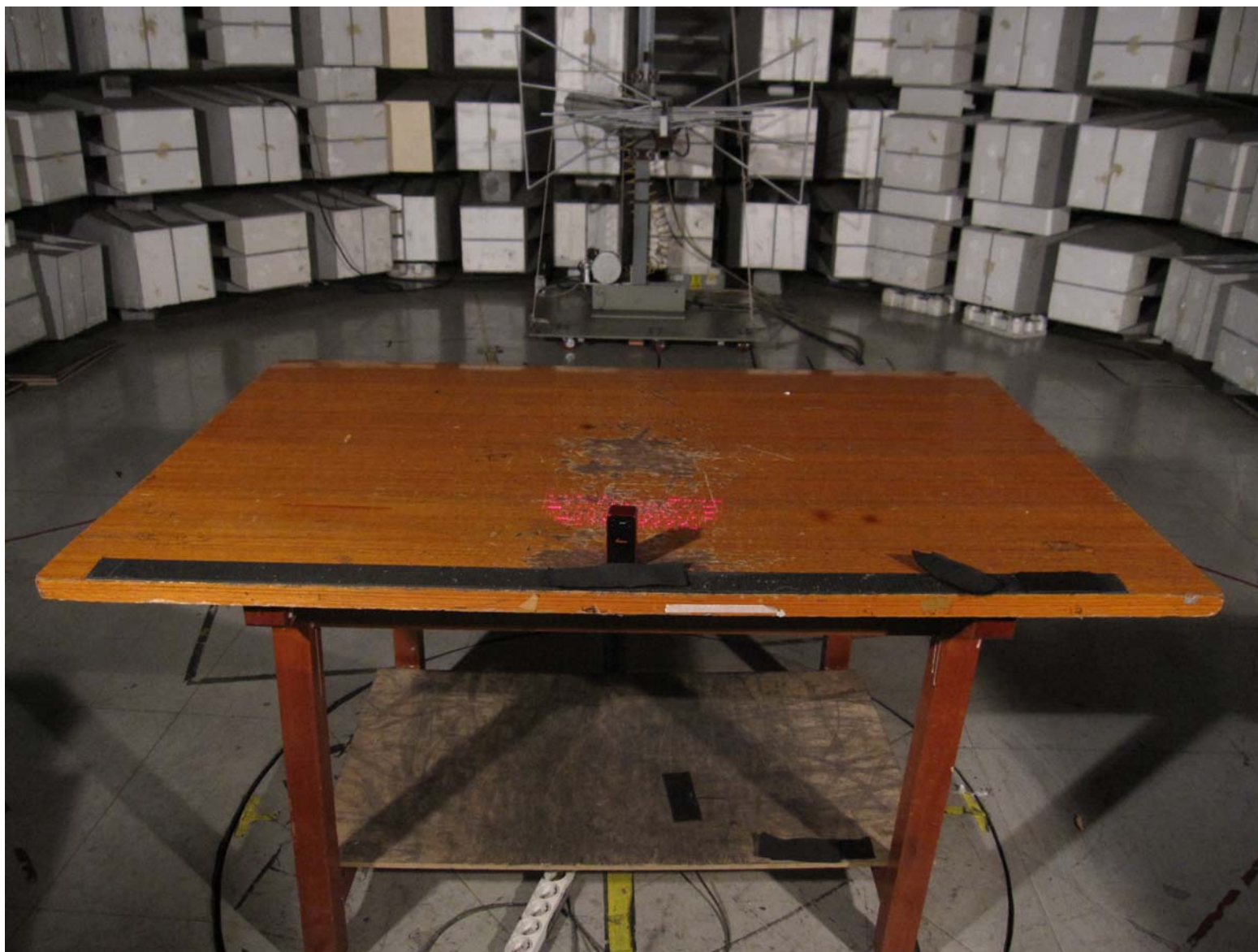
Magic Cube_Radiated Emission 30 MHz to 1 GHz (Portable) Rear
