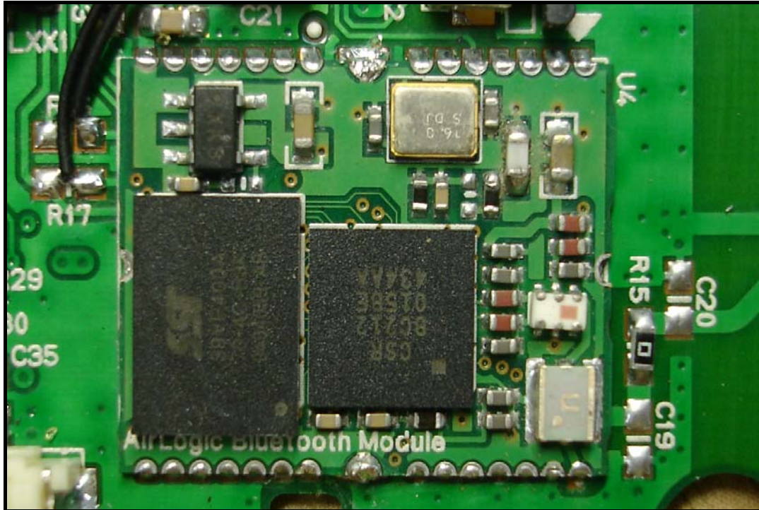
<Photograph 8: RF Module – Shielding can removed>
