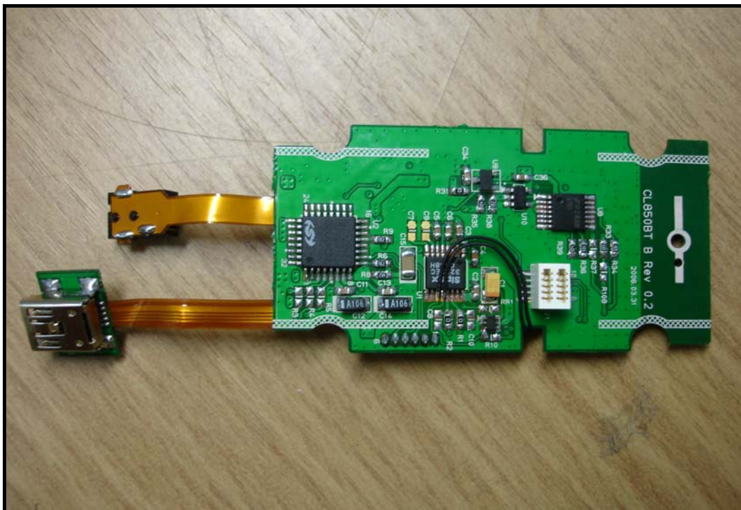
<Photograph 5: Rear Side – Main board>
