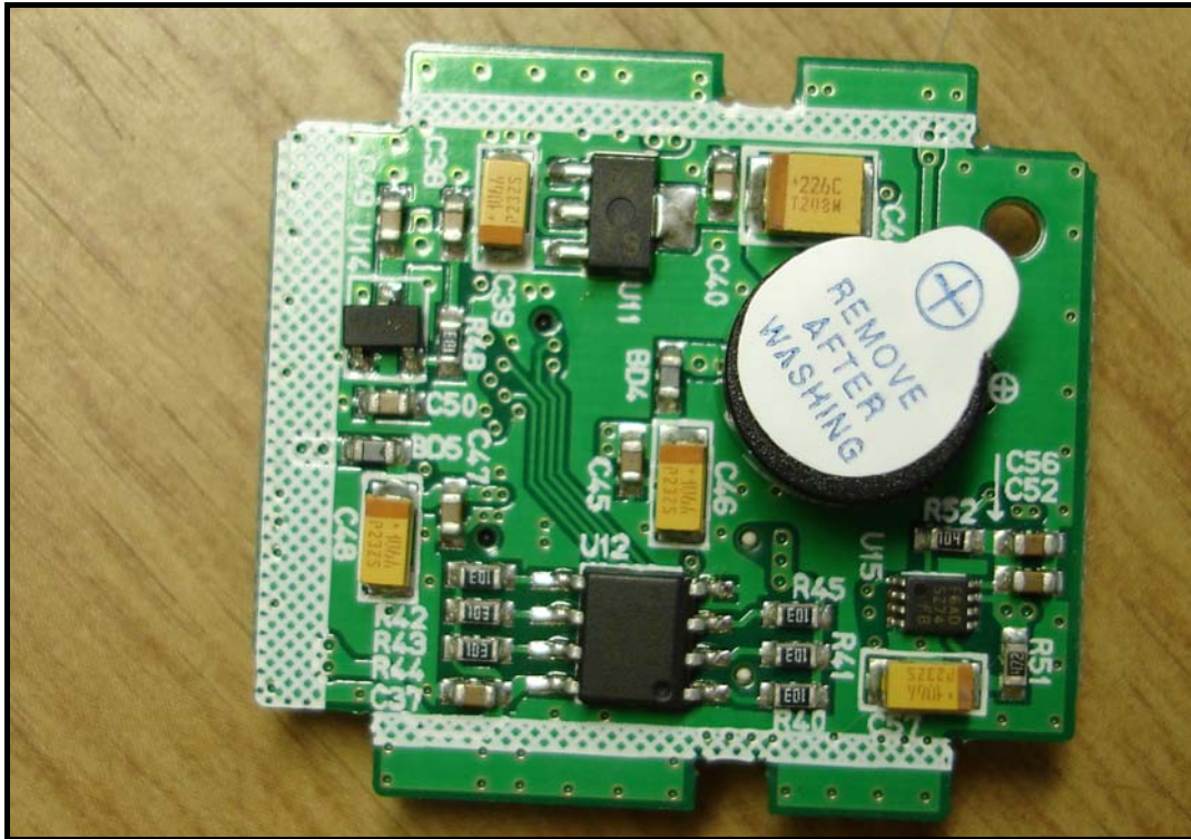
<Photograph 6: Front Side – Sub-board>
