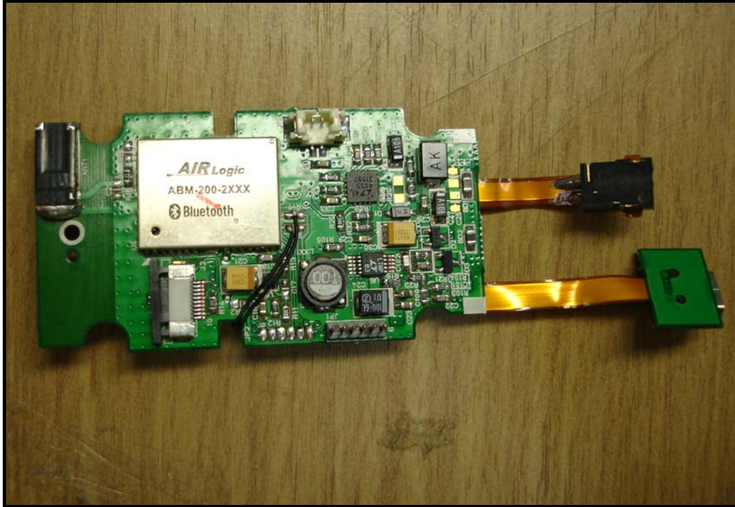
<Photograph 4: Front Side – Main board>
