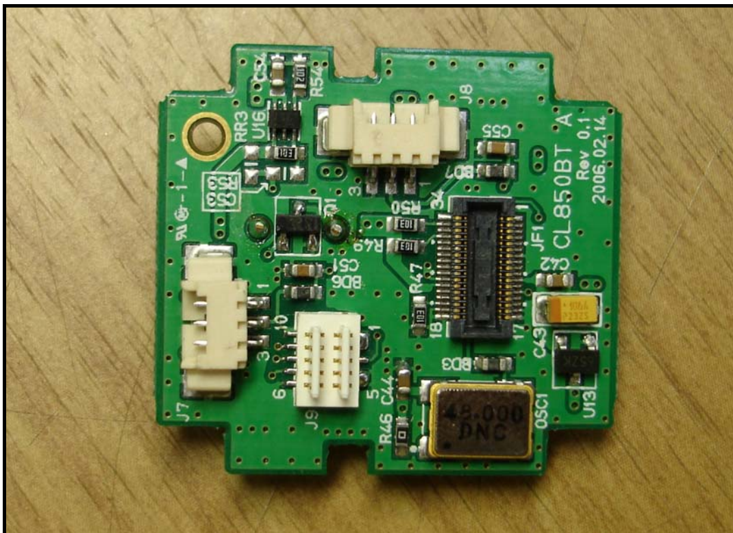
<Photograph 7: Rear Side – Sub-board>
