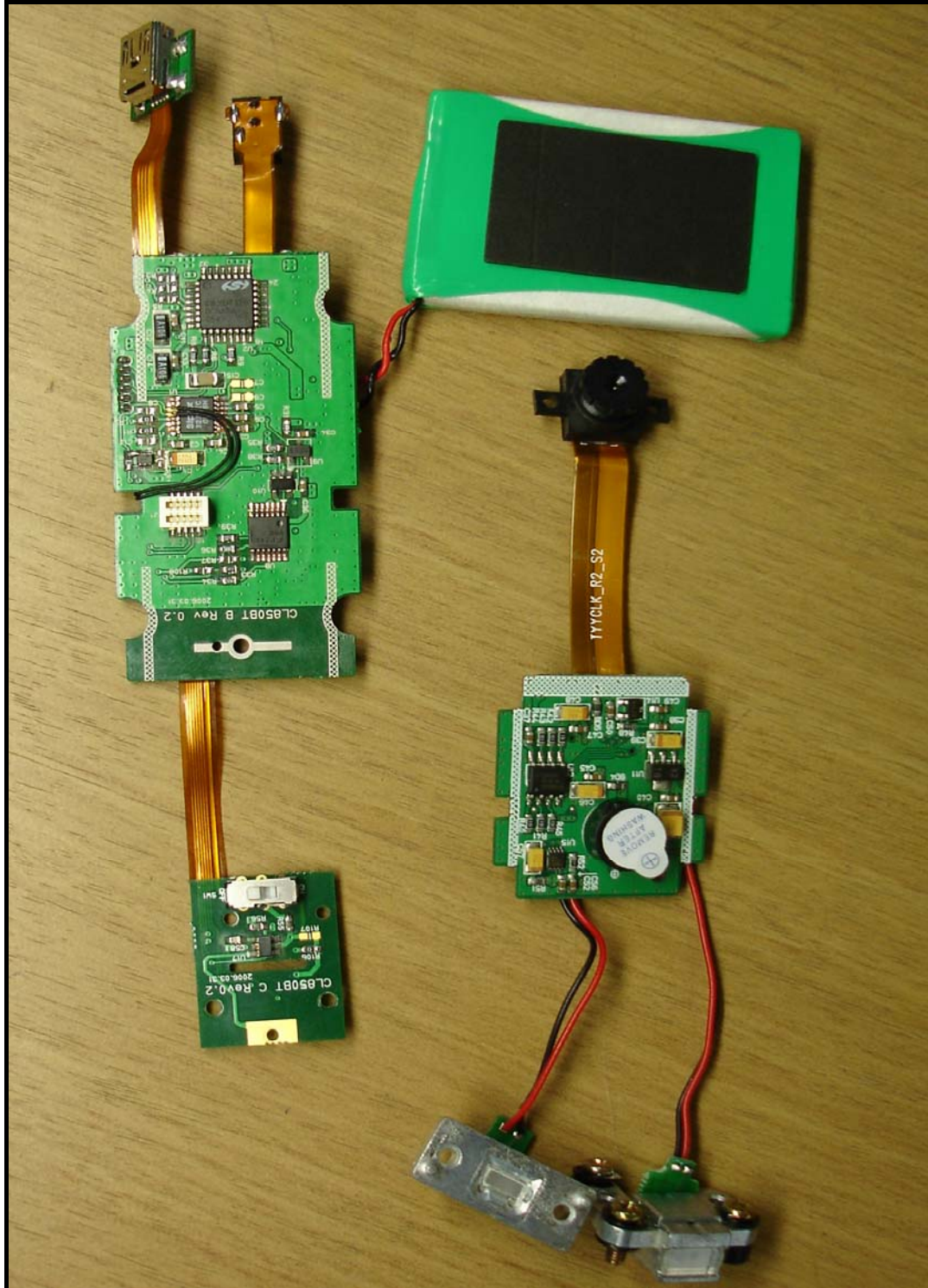
&lt;Photograph 3: Rear Side &gt;
