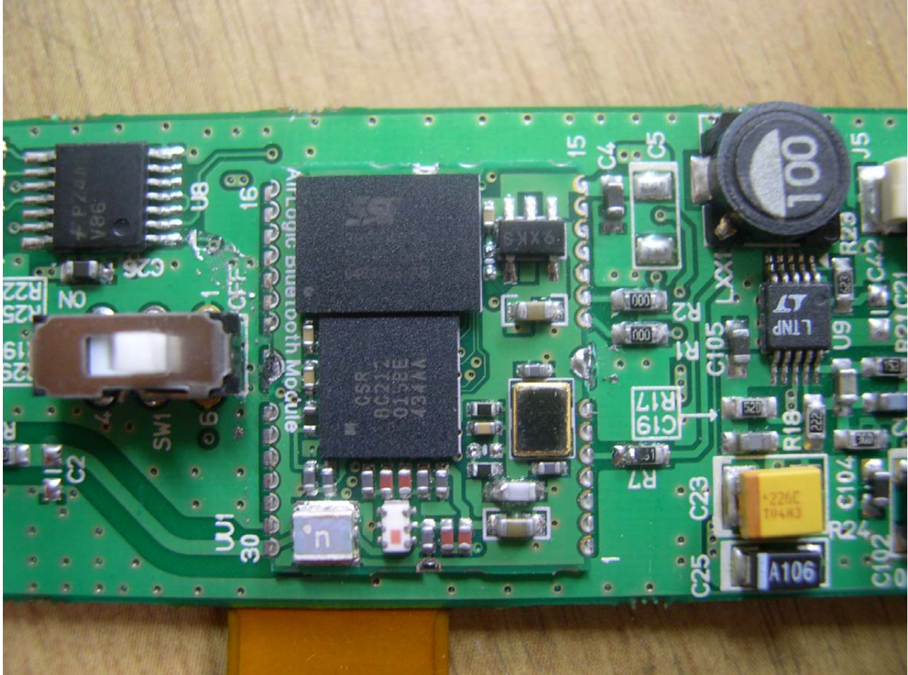
<Photograph 8: RF Module – Shielding can be removed>
