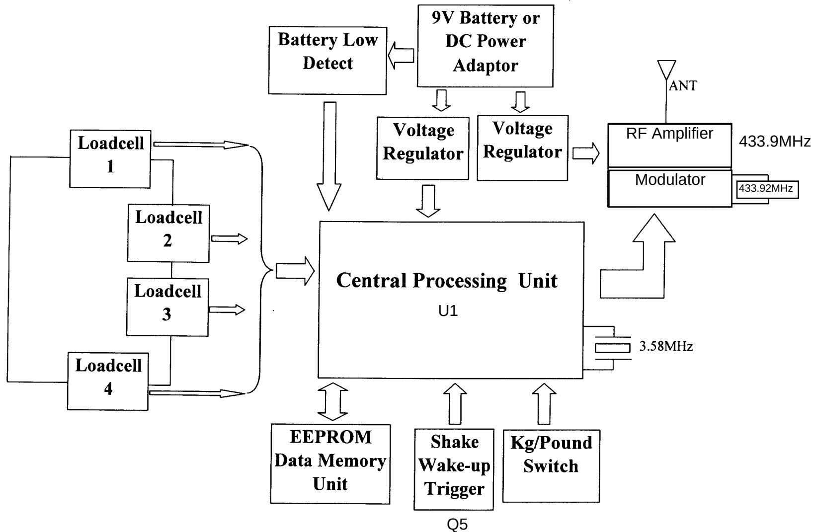
DS-300 Tx Block Diagram
