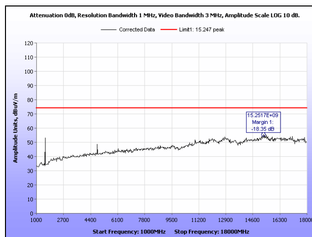
Plot 9. Radiated Spurious Emissions, Low Channel, 802.11g, 1 GHz – 18 GHz, Peak
