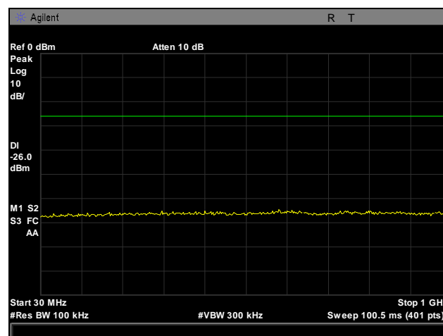
Plot 22. Conducted Spurious Emissions, Mid Channel, 802.11g, 30 MHz – 1 GHz
