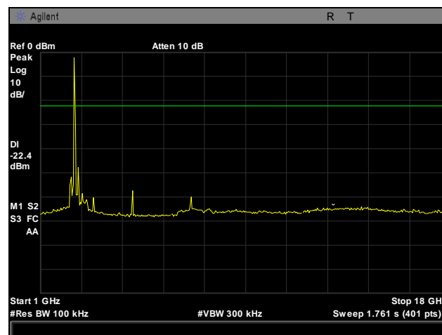
Plot 21. Conducted Spurious Emissions, Low Channel, 802.11g, 1 GHz – 18 GHz
