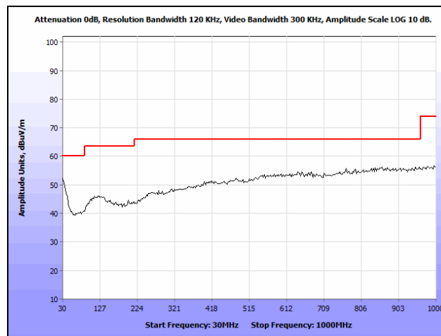
Plot 26. Radiated Spurious Emissions, Low Channel, 2412 MHz, 802.11g, 30 MHz – 1 GHz, Peak
