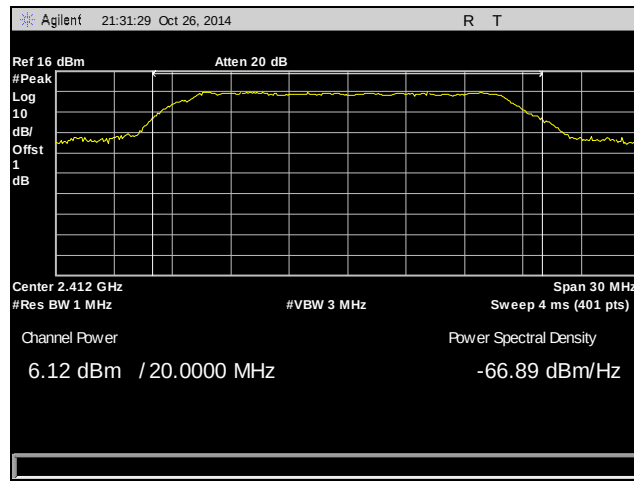
Plot 10. Peak Power Output, Low Channel, 2412 MHz, 802.11g
