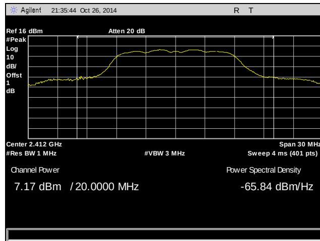
Plot 7. Peak Power Output, Low Channel, 2412 MHz, 802.11b
