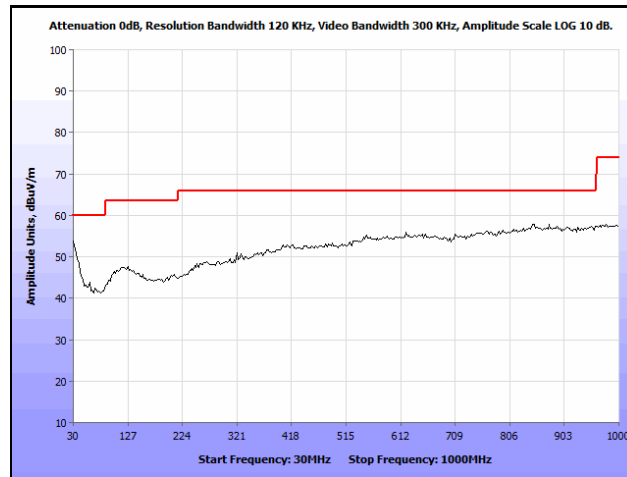
Plot 22. Radiated Spurious Emissions, High Channel, 2462 MHz, 802.11b, 30 MHz – 1 GHz, Peak
