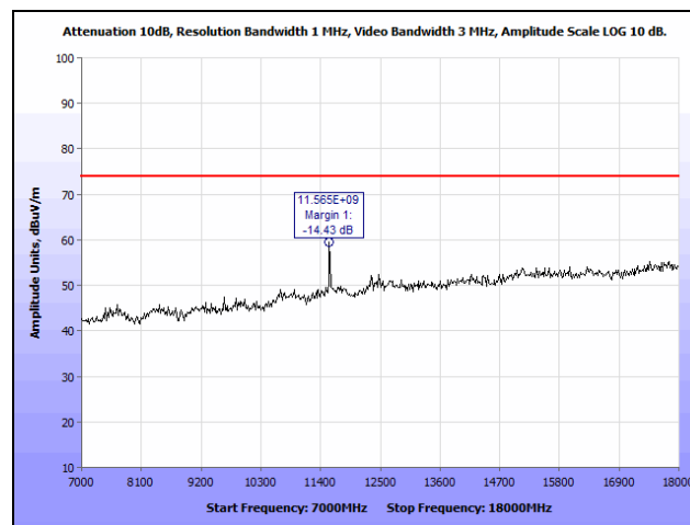
Plot 17. Radiated Spurious Emissions, Mid Channel, 5785 MHz, 802.11a, 7 GHz – 18 GHz, Peak
