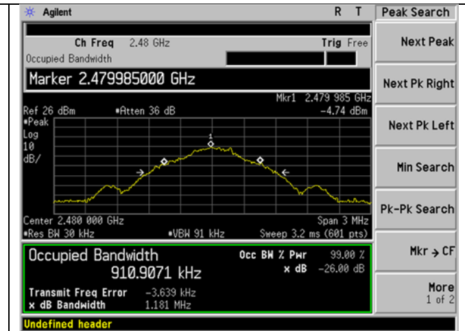
DH1 2480 MHz 99 Percent Occupied Bandwidth
