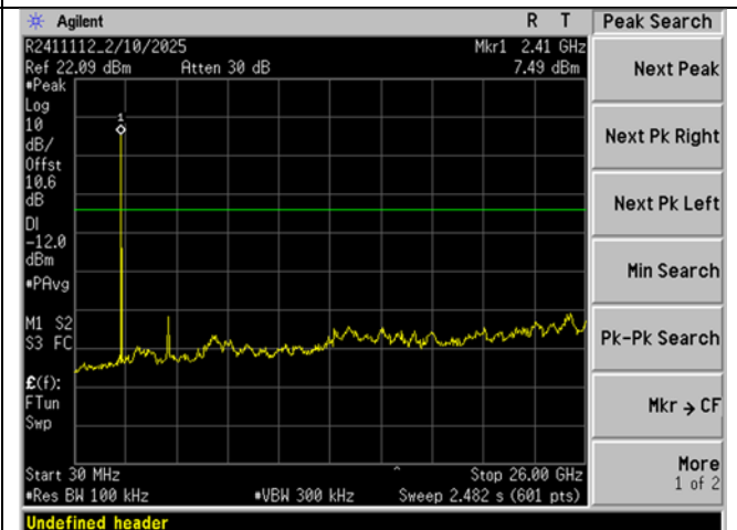
BLE_Low Ch_2402MHz_2MBit_-20dBc_30MHz-26GHz
