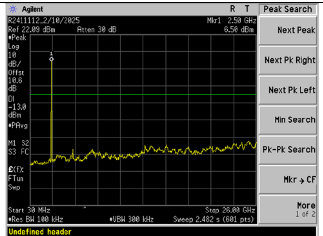
BLE_High Ch_2480MHz_1MBit_-20dBc_30MHz-26GHz
