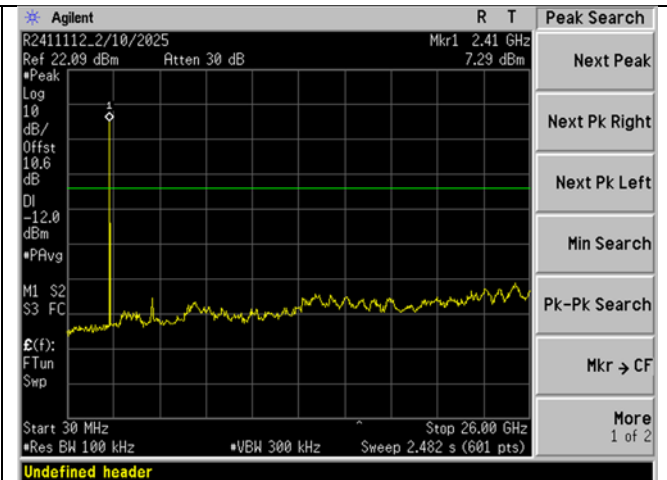
BLE_Low Ch_2402MHz_1MBit_-20dBc_30MHz-26GHz
