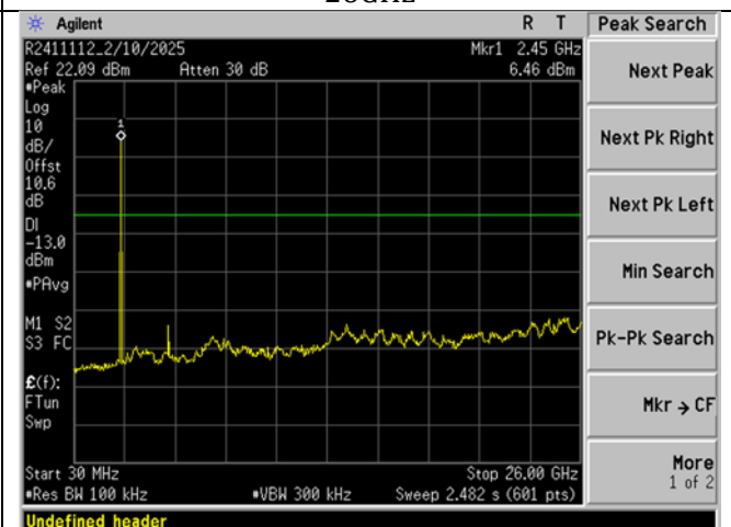
BLE_Mid Ch_2442MHz_1MBit_-20dBc_30MHz-26GHz
