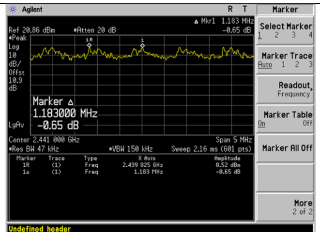
8DPSK hopping channel separation
