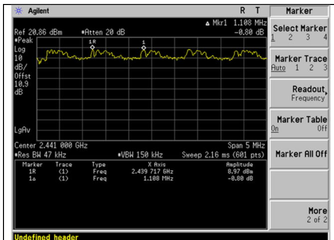
\pi/4 -DQPSK hopping channel separation
