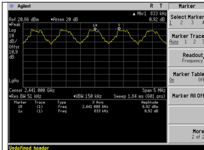
GFSK hopping channel separation
