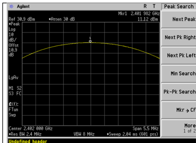
OUTPUT POWER 8DPSK low
