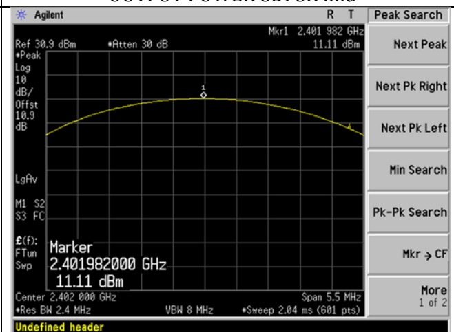
OUTPUT POWER GFSK low
