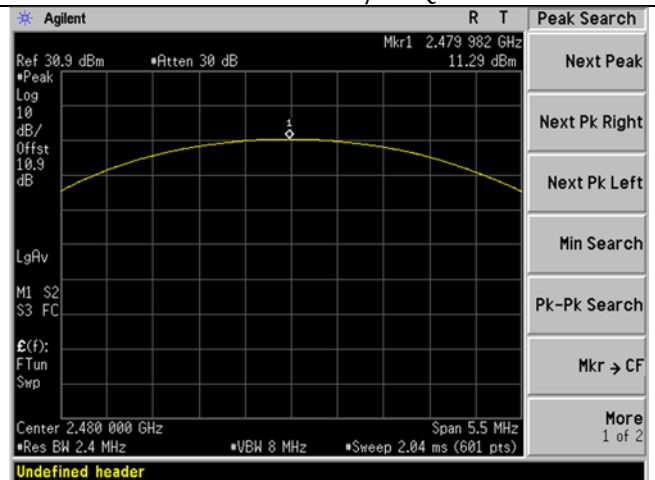
OUTPUT POWER 8DPSK high
