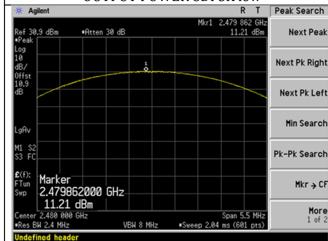
OUTPUT POWER GFSK high
