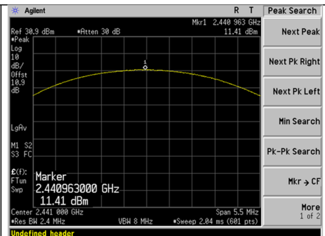
OUTPUT POWER 8DPSK mid
