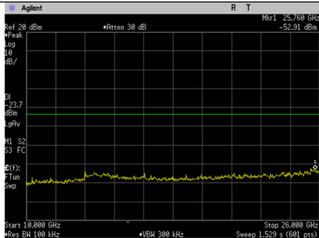
BLE_High CH_2480MHz_1MHz BW_Mbit_20dBc_10-26GHz
