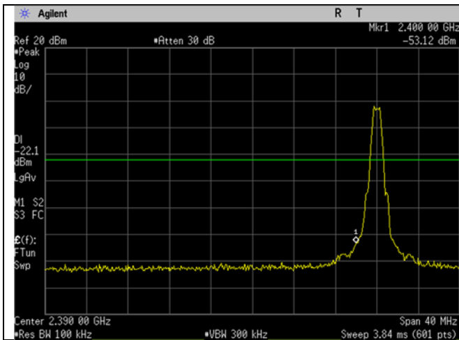
BLE_Low CH_2402MHz_1MHz BW_Mbit_20dBc Lower Band Edge
