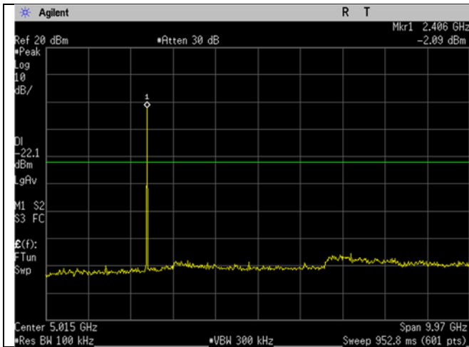
BLE_Low CH_2402MHz_1MHz BW_Mbit_20dBc_30MHz-10GHz
