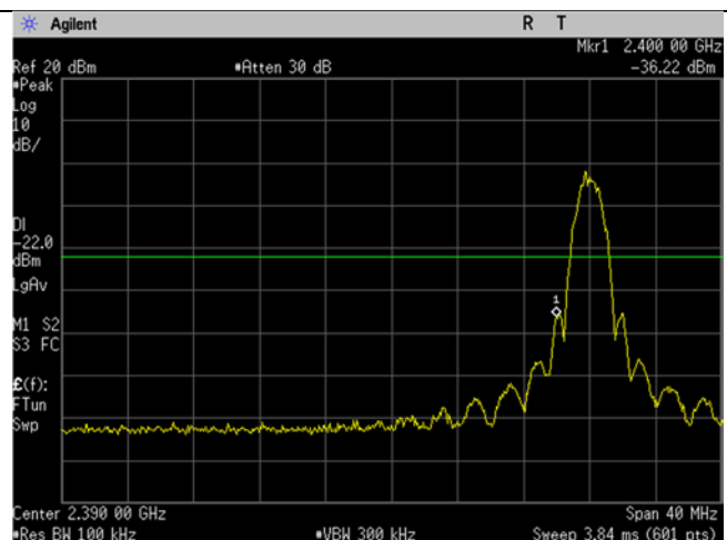
BLE_Low CH_2402MHz_2MHz BW_Mbit_20dBc Lower Band Edge
