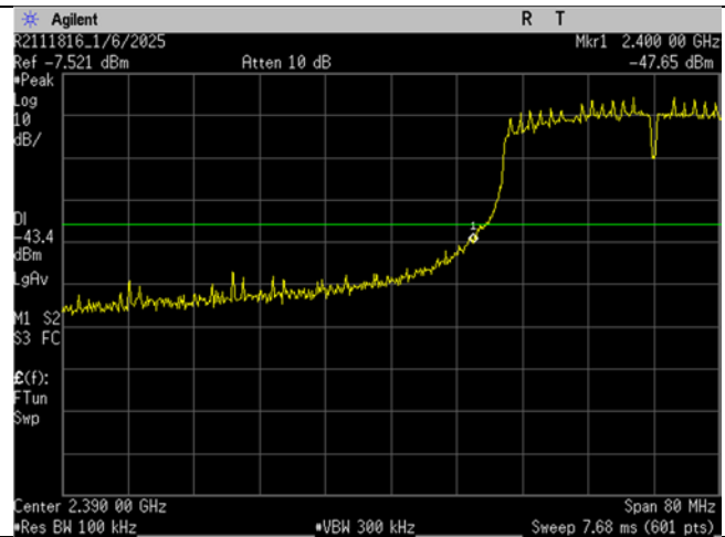
WIFI_Low Ch_2422MHz_40MHz BW_n-mode_- 30dBc_Lower Band Edge
