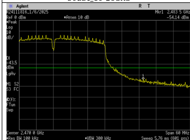
WIFI_High Ch_2452MHz_40MHz BW_n-mode_-30dBc_Upper Band Edge
