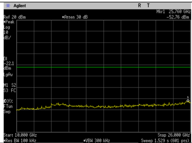
BLE_Low CH_2402MHz_1MHz BW_Mbit_20dBc_10- 26GHz
