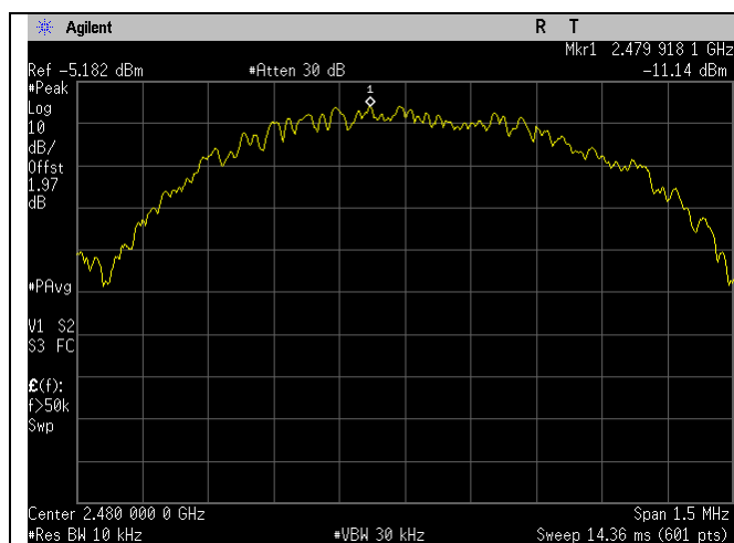
BLE_High Ch_2480MHz_1MBit_Spectral Density_Port 1
