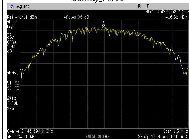
BLE_Mid Ch_2440MHz_1MBit_Spectral Density_Port 1
