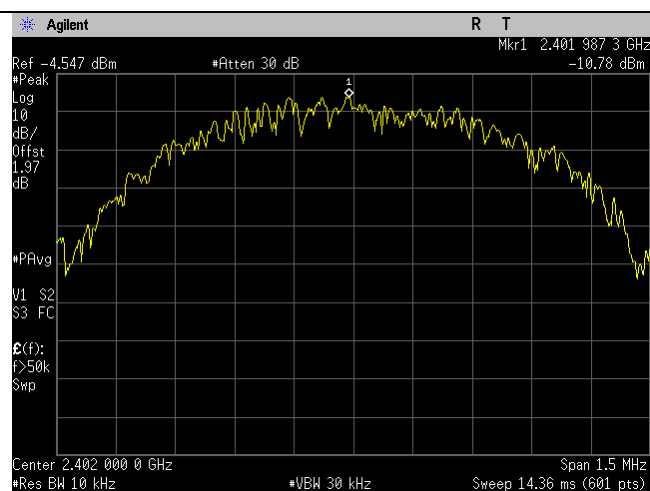
BLE_Low Ch_2402MHz_1MBit_Spectral Density_Port 1
