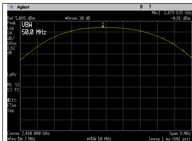
BLE_High Ch_2480MHz_1MBit_Output Power_Port 1
