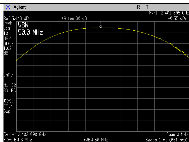
BLE_Low Ch_2402MHz_1MBit_Output Power_Port 1
