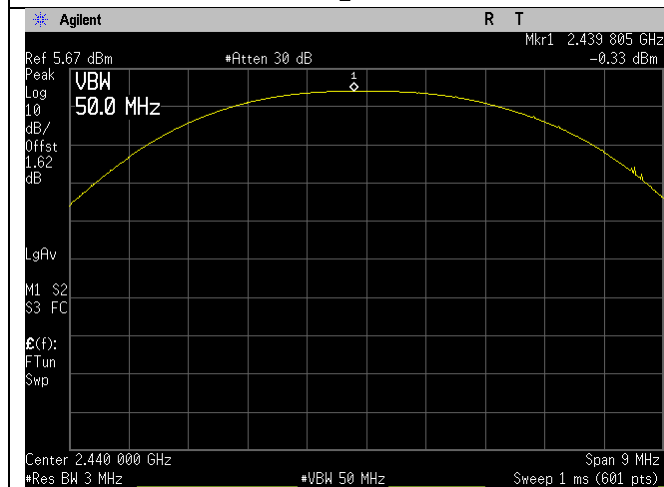
BLE_Mid Ch_2440MHz_1MBit_Output Power_Port 1
