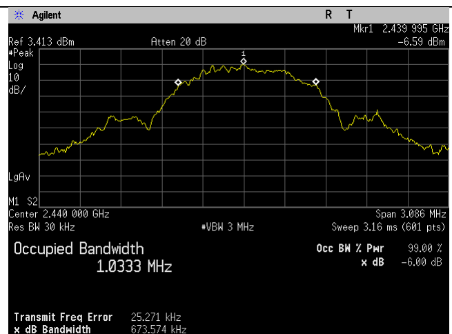
BLE_Mid Ch_2440MHz_1MBit_Occupied Bandwidth_99 percent_Port 1
