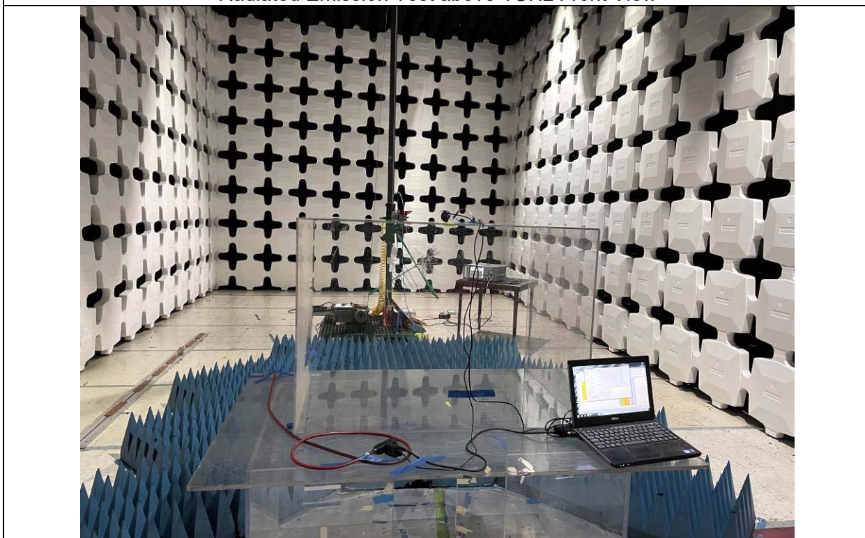
Radiated Emission Test above 1GHz Rear View
