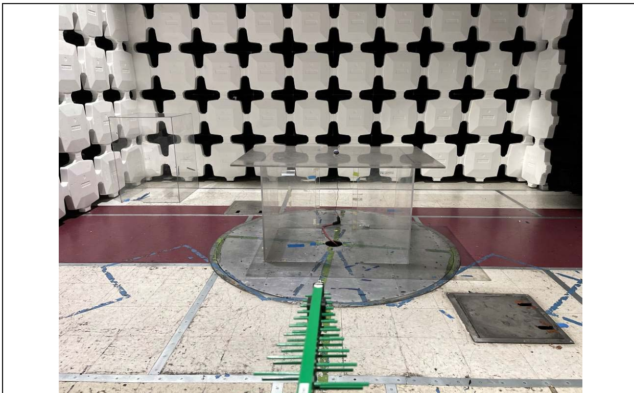
Radiated Emission Test below 1GHz Front View
