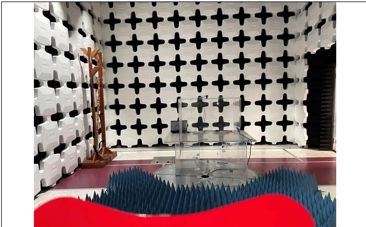
Radiated Emission Test above 1GHz Front View
