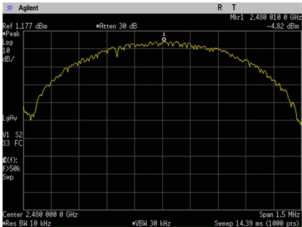
BLE_High Ch_2480MHz_1MBit_Spectral Density_Port 1
