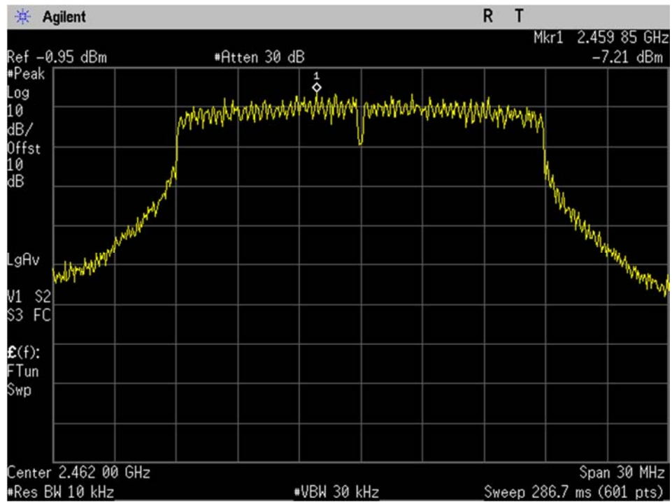
WIFI_High Ch_2462MHz_20MHz BW_n-mode_Spectral Density_Port 1
