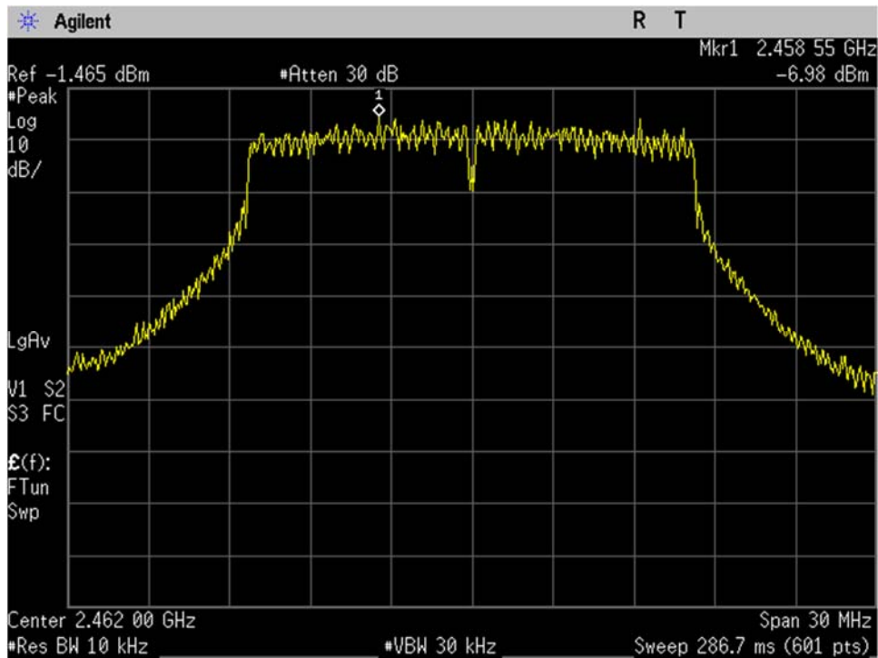
WIFI_High Ch_2462MHz_20MHz BW_g-mode_Spectral Density_Port 2
