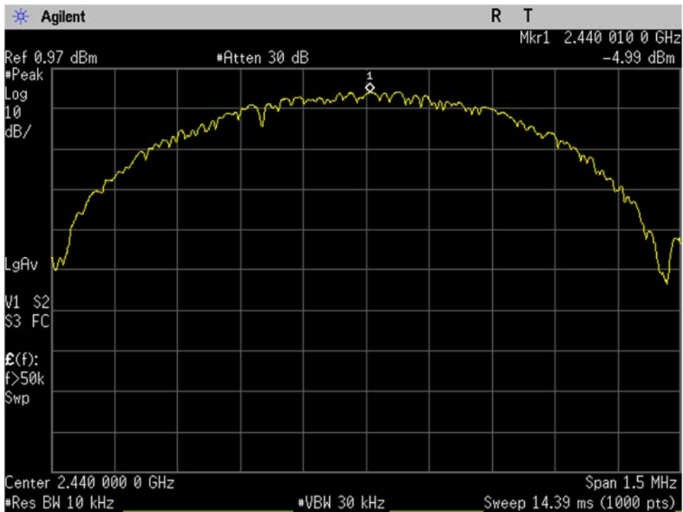
BLE_Mid Ch_2440MHz_1MBit_Spectral Density_Port 1
