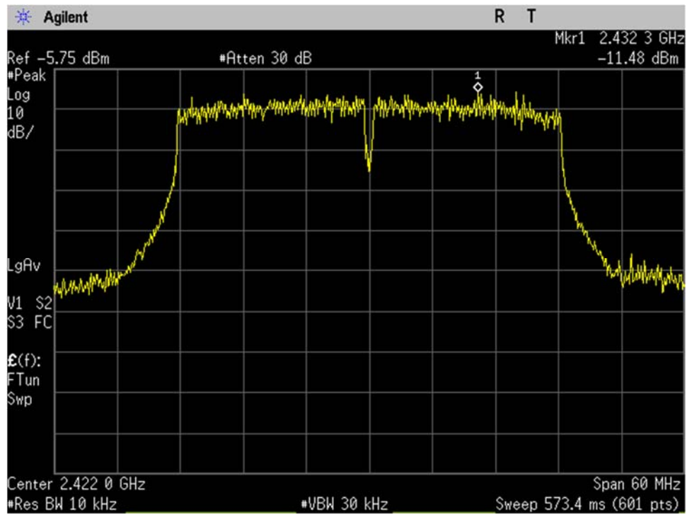
WIFI_Low Ch_2422MHz_40MHz BW_n-mode_Spectral Density_Port 1
