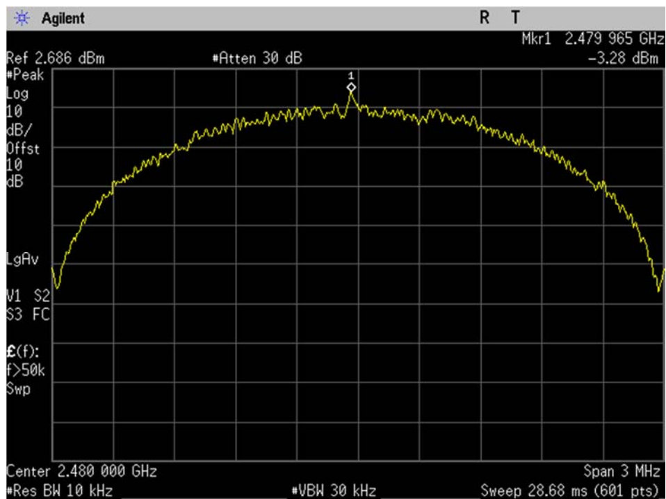
BLE_Mid Ch_2480MHz_2MBit_Spectral Density_Port 1
