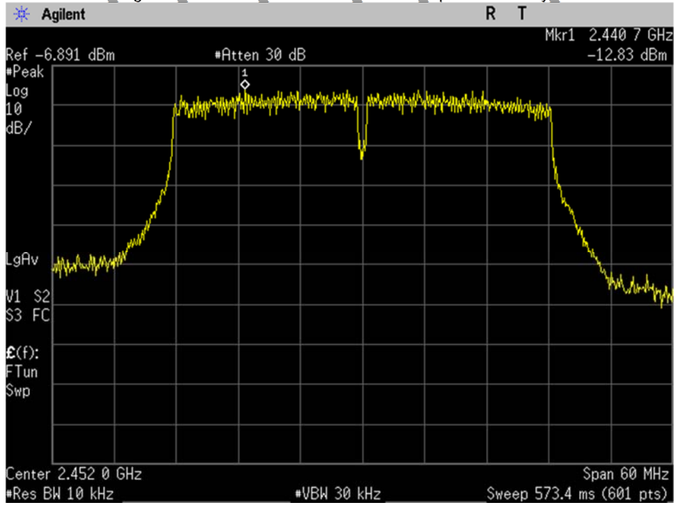
WIFI_High Ch_2452MHz_40MHz BW_n-mode_Spectral Density_Port 1
