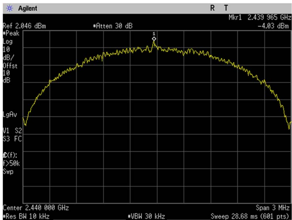
BLE_High Ch_2440MHz_2MBit_Spectral Density_Port 1
