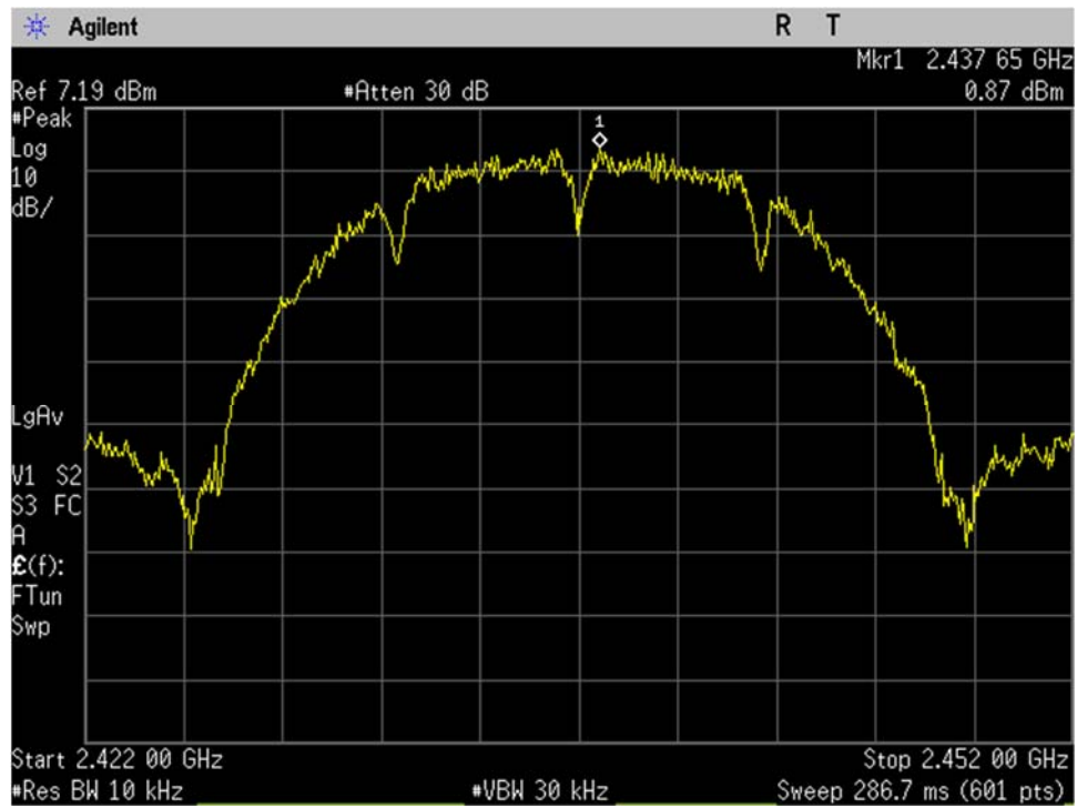
WIFI_Mid Ch_2437MHz_20MHz BW_b-mode_Spectral Density_Port 1
