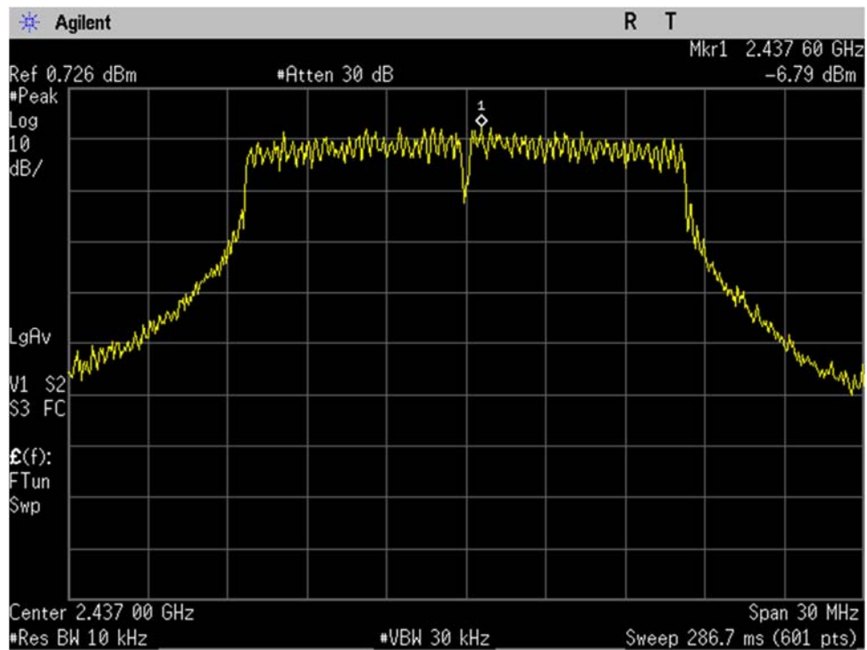
WIFI_Mid Ch_2437MHz_20MHz BW_g-mode_Spectral Density_Port 2
