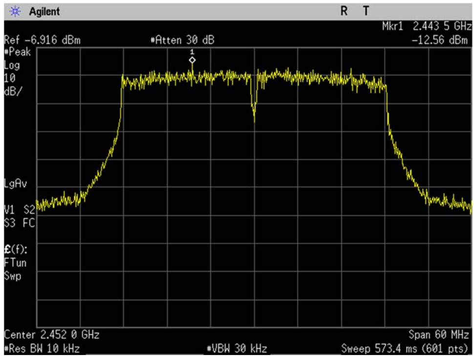
WIFI_High Ch_2452MHz_40MHz BW_n-mode_Spectral Density_Port 2
