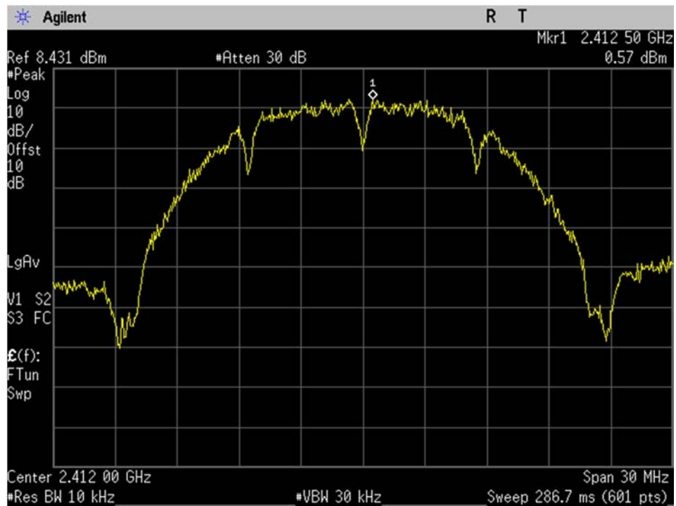
WIFI_Low Ch_2412MHz_20MHz BW_b-mode_Spectral Density_Port 1
