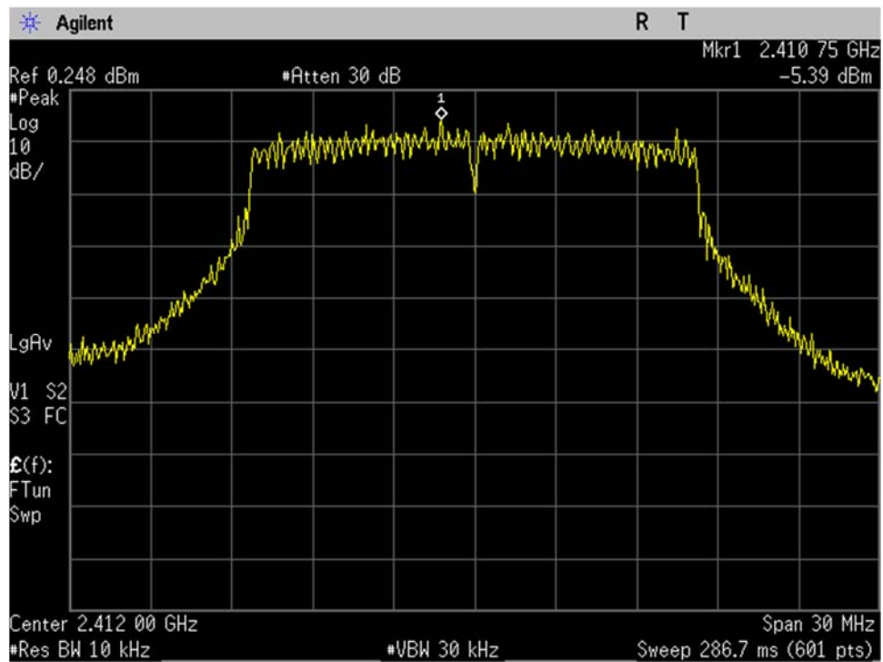
WIFI_Low Ch_2412MHz_20MHz BW_g-mode_Spectral Density_Port 2
