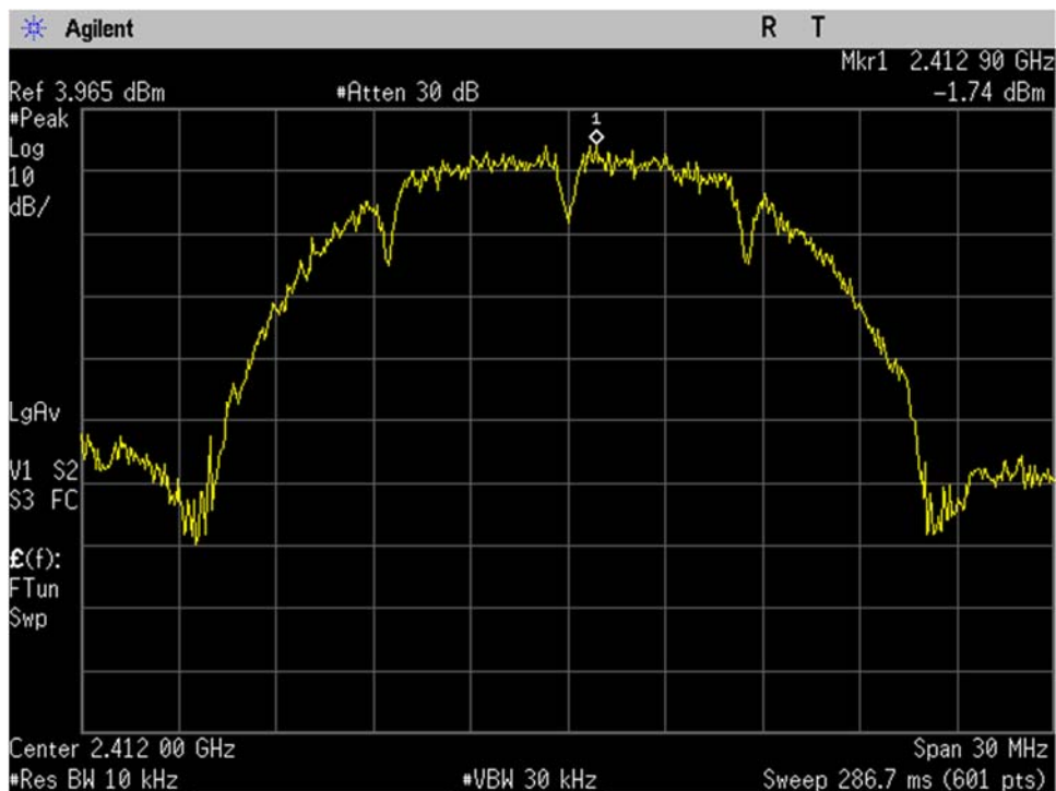
WIFI_Low Ch_2412MHz_20MHz BW_b-mode_Spectral Density_Port 2
