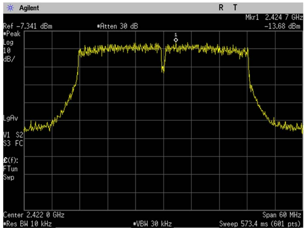
WIFI_Low Ch_2422MHz_40MHz BW_n-mode_Spectral Density_Port 2
