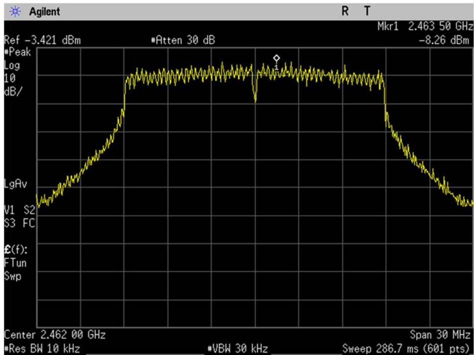
WIFI_High Ch_2462MHz_20MHz BW_n-mode_Spectral Density_Port 2
