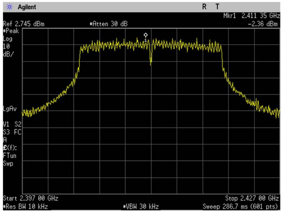
WIFI_Low Ch_2412MHz_20MHz BW_g-mode_Spectral Density_Port 1
