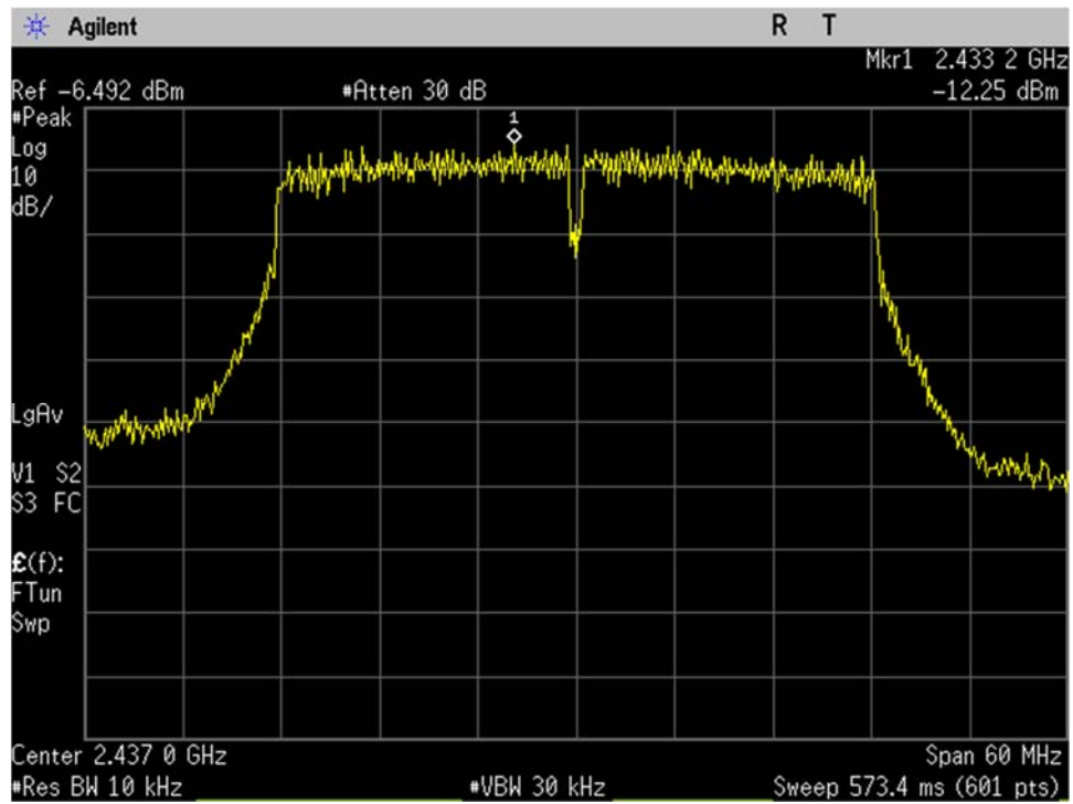
WIFI_Mid Ch_2437MHz_40MHz BW_n-mode_Spectral Density_Port 1
