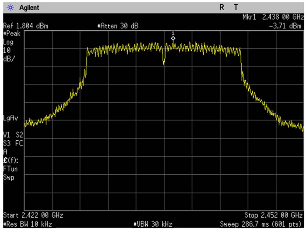
WIFI_Mid Ch_2437MHz_20MHz BW_g-mode_Spectral Density_Port 1
