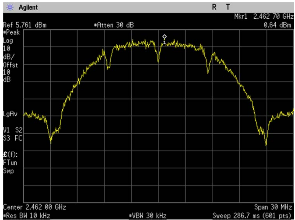
WIFI_High Ch_2462MHz_20MHz BW_b-mode_Spectral Density_Port 1
