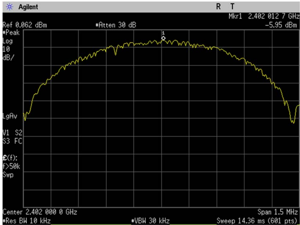
BLE_Low Ch_2402MHz_1MBit_Spectral Density_Port 1
