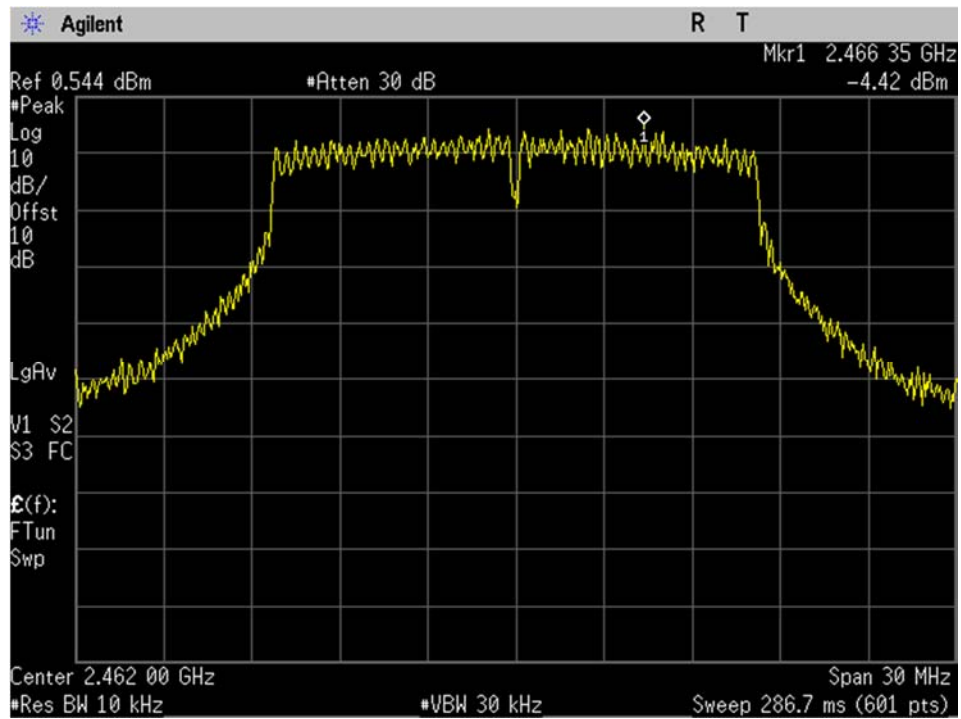
WIFI_High Ch_2462MHz_20MHz BW_g-mode_Spectral Density_Port 1
