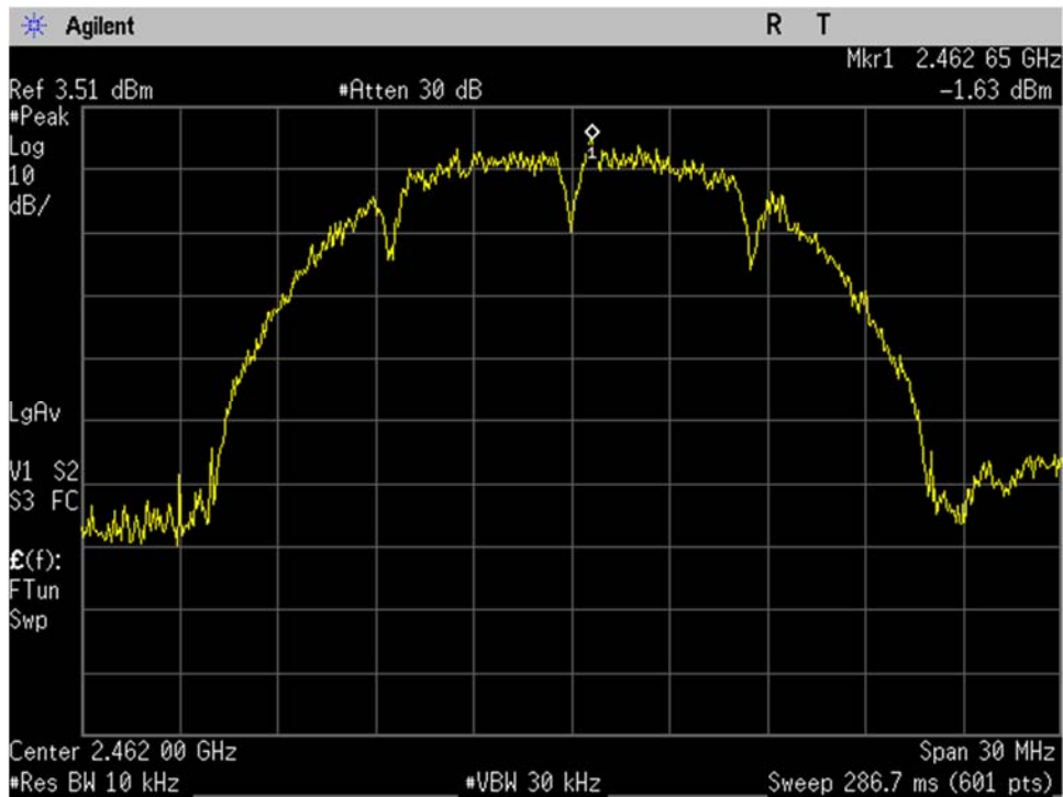
WIFI_High Ch_2462MHz_20MHz BW_b-mode_Spectral Density_Port 2
