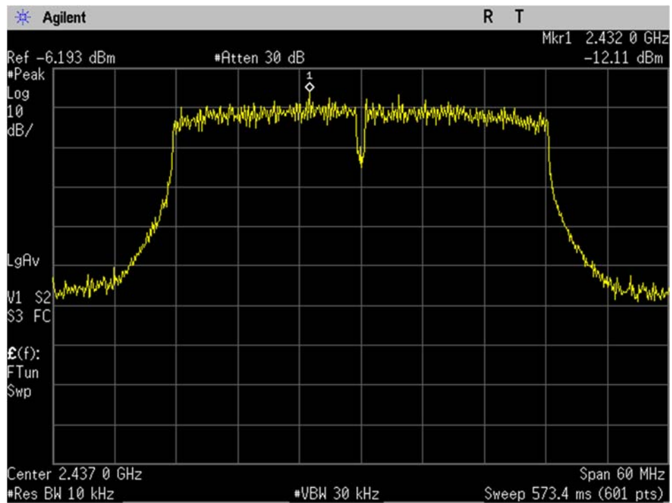
WIFI_Mid Ch_2437MHz_40MHz BW_n-mode_Spectral Density_Port 2
