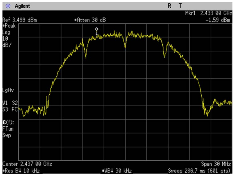
WIFI_Mid Ch_2437MHz_20MHz BW_b-mode_Spectral Density_Port 2
