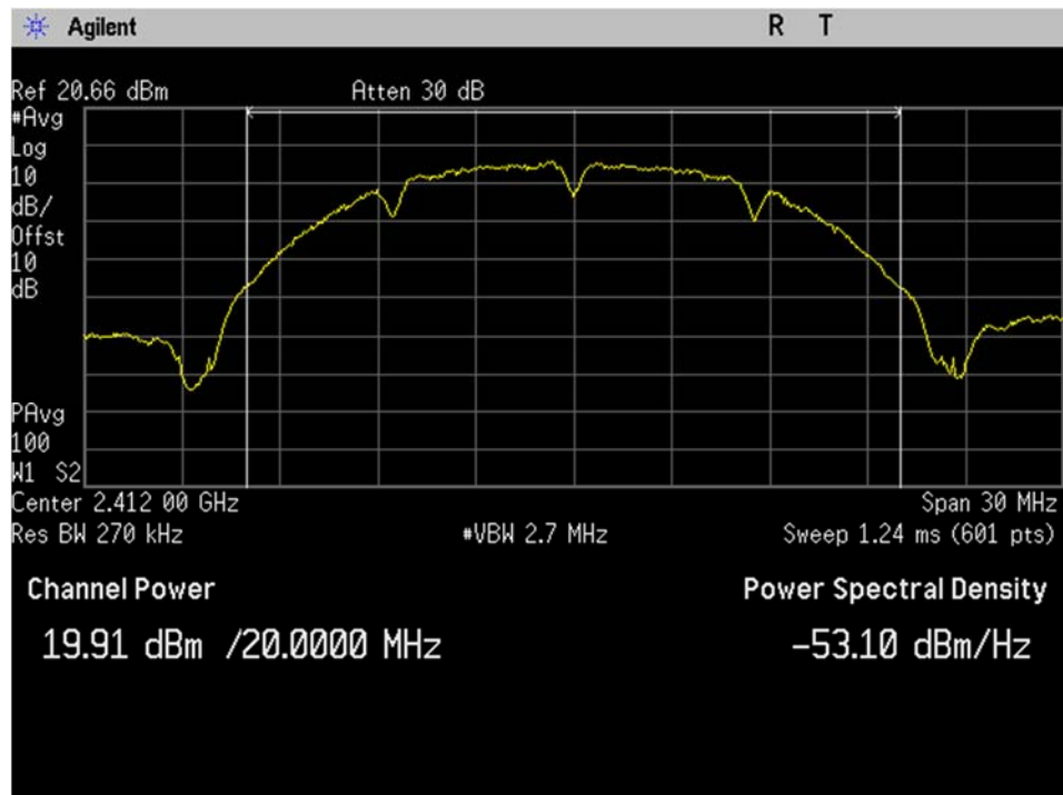
WIFI_Low Ch_2412MHz_20MHz BW_b-mode_Output Power_Port 1
