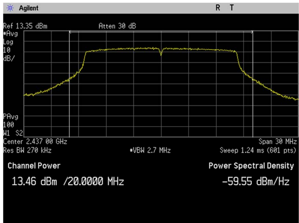
WIFI_Mid Ch_2437MHz_20MHz BW_g-mode_Output Power_Port 2
