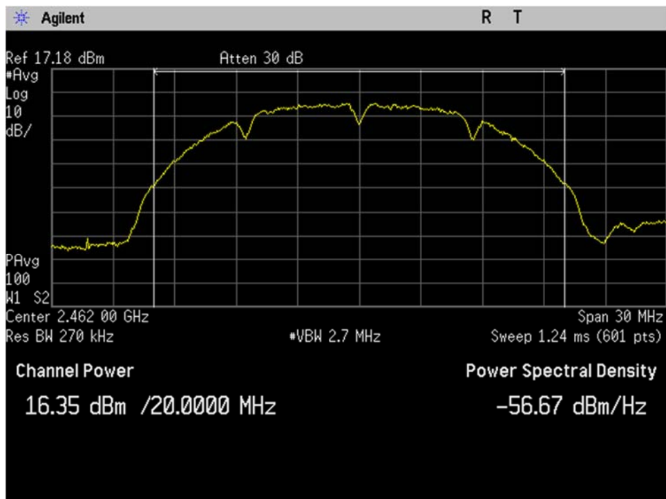
WIFI_High Ch_2462MHz_20MHz BW_b-mode_Output Power_Port 2
