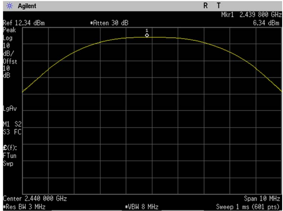
BLE_High Ch_2440MHz_2MBit_Output Power_Port 1
