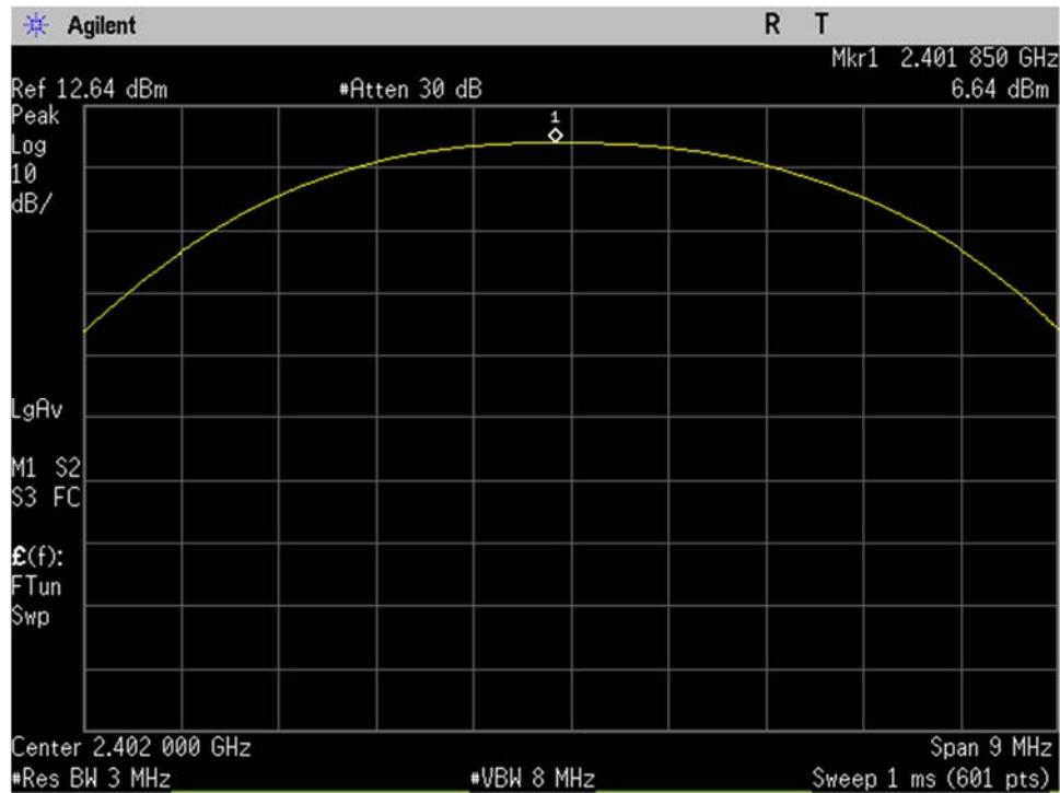
BLE_Low Ch_2402MHz_1MBit_Output Power_Port 1
