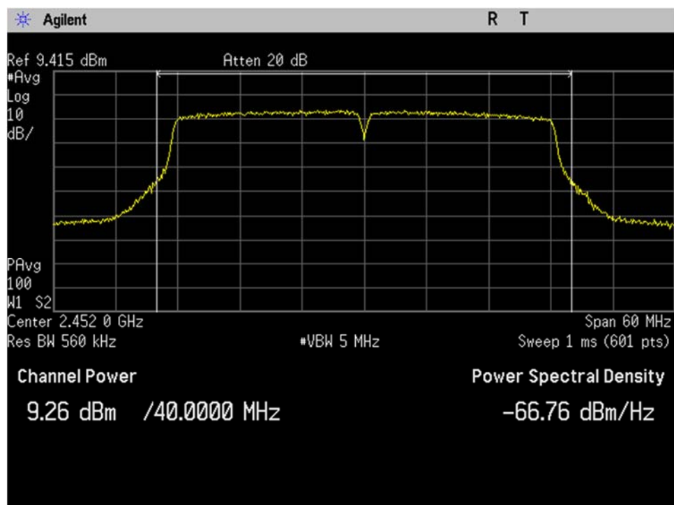
WIFI_High Ch_2452MHz_40MHz BW_n-mode_Output Power_Port 2
