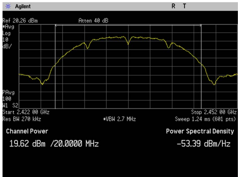
WIFI_Mid Ch_2437MHz_20MHz BW_b-mode_Output Power_Port 1
