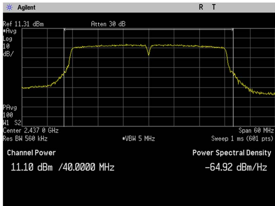
WIFI_Mid Ch_2437MHz_40MHz BW_n-mode_Output Power_Port 1
