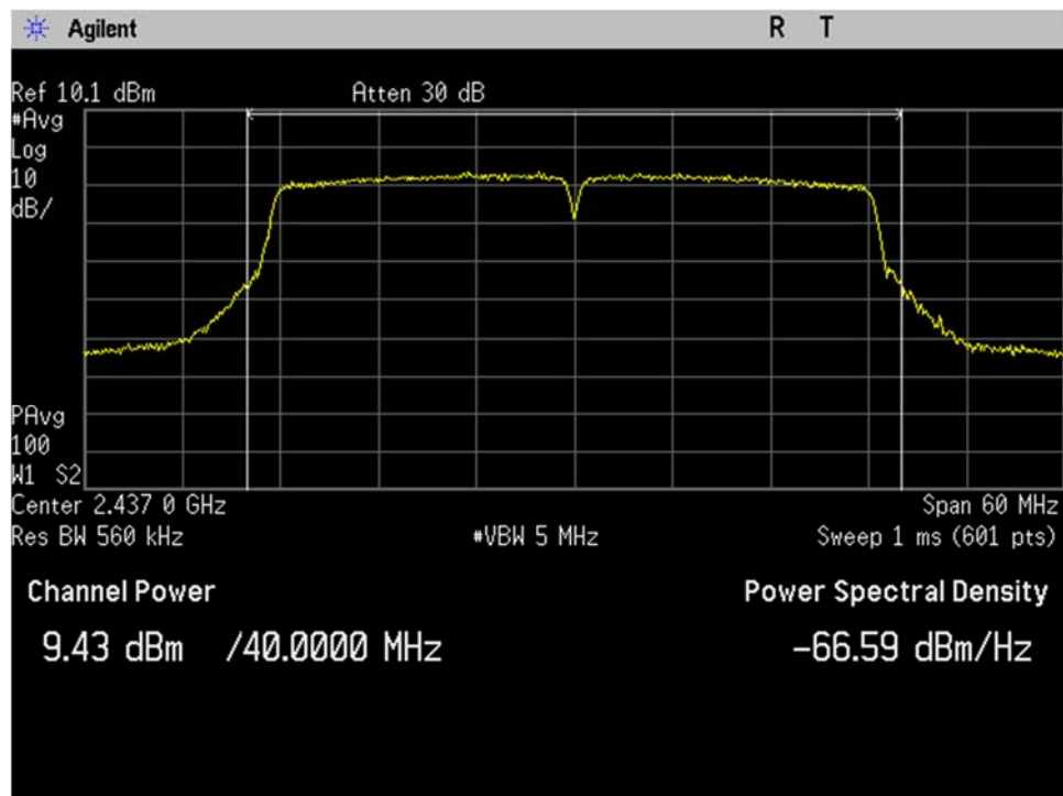
WIFI_Mid Ch_2437MHz_40MHz BW_n-mode_Output Power_Port 2
