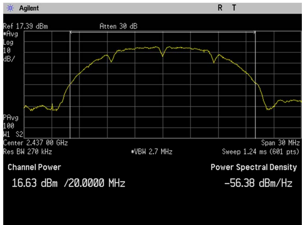
WIFI_Mid Ch_2437MHz_20MHz BW_b-mode_Output Power_Port 2
