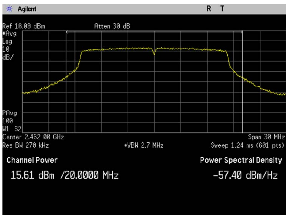
WIFI_High Ch_2462MHz_20MHz BW_g-mode_Output Power_Port 1
