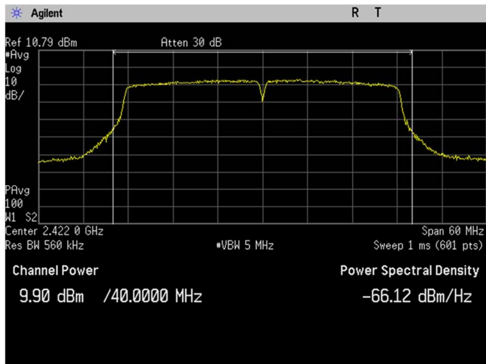
WIFI_Low Ch_2422MHz_40MHz BW_n-mode_Output Power_Port 2
