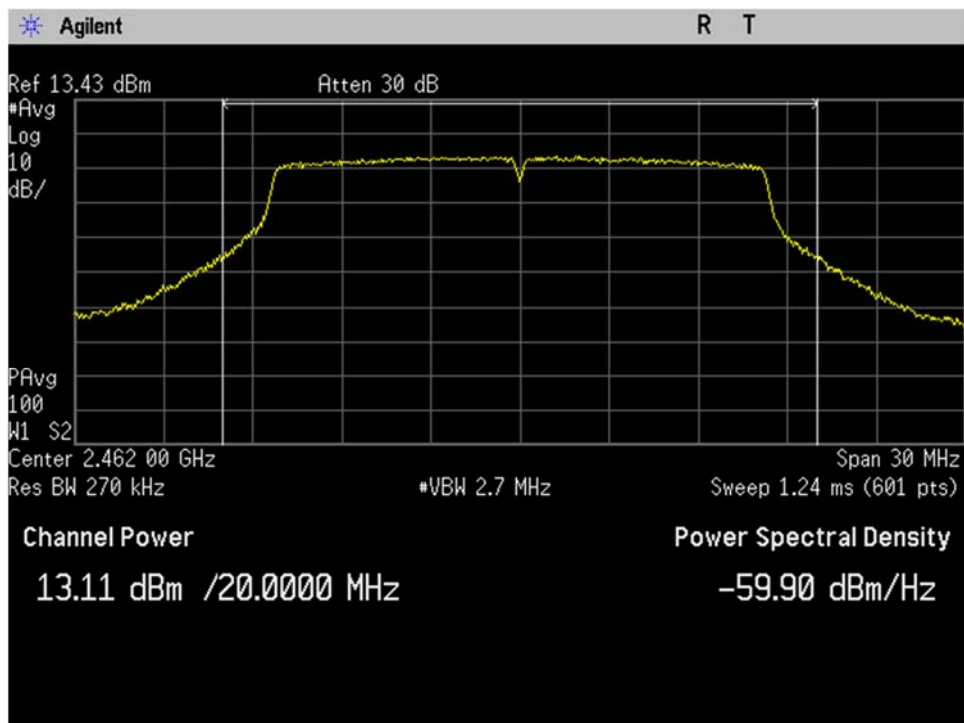
WIFI_High Ch_2462MHz_20MHz BW_g-mode_Output Power_Port 2
