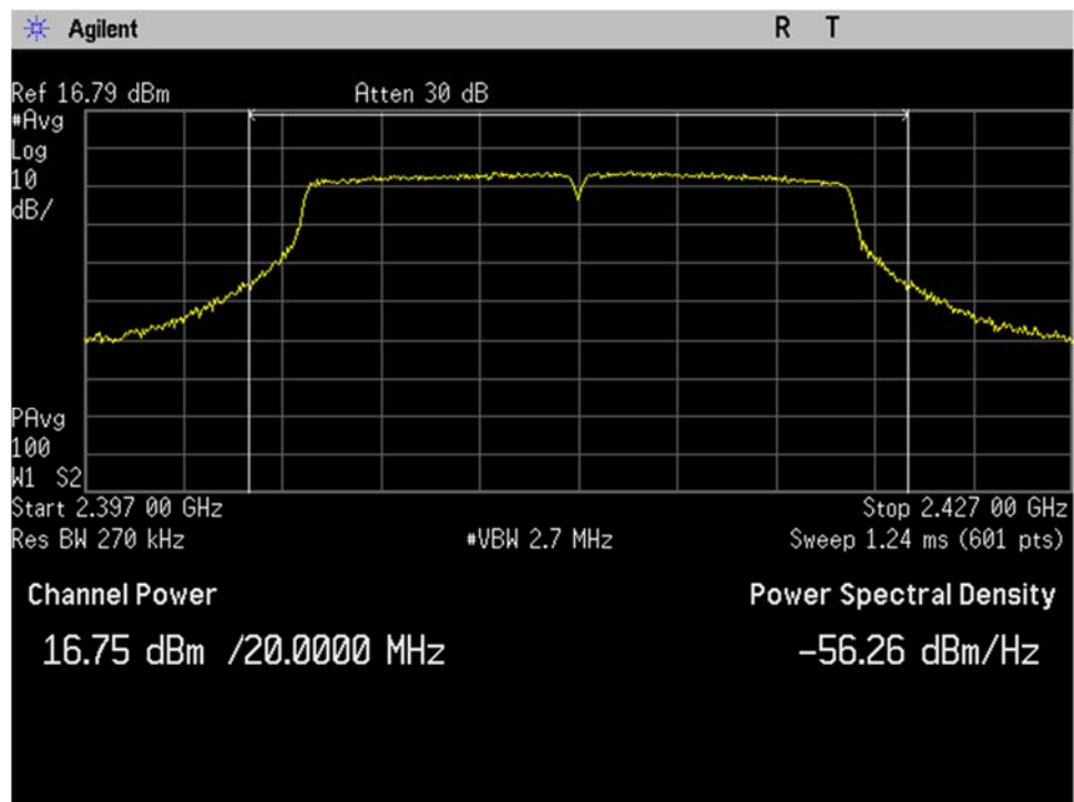
WIFI_Low Ch_2412MHz_20MHz BW_g-mode_Output Power_Port 1
