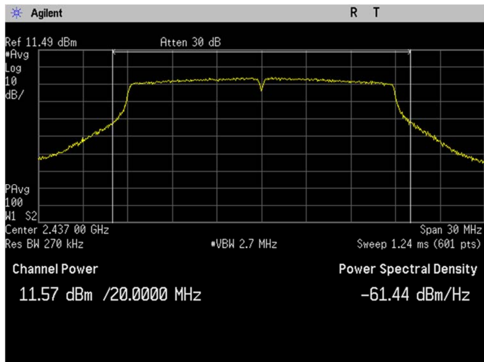
WIFI_Mid Ch_2437MHz_20MHz BW_n-mode_Output Power_Port 2
