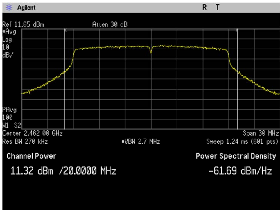
WIFI_High Ch_2462MHz_20MHz BW_n-mode_Output Power_Port 2
