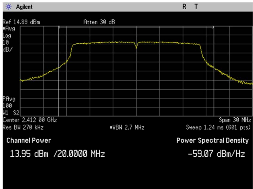
WIFI_Low Ch_2412MHz_20MHz BW_g-mode_Output Power_Port 2
