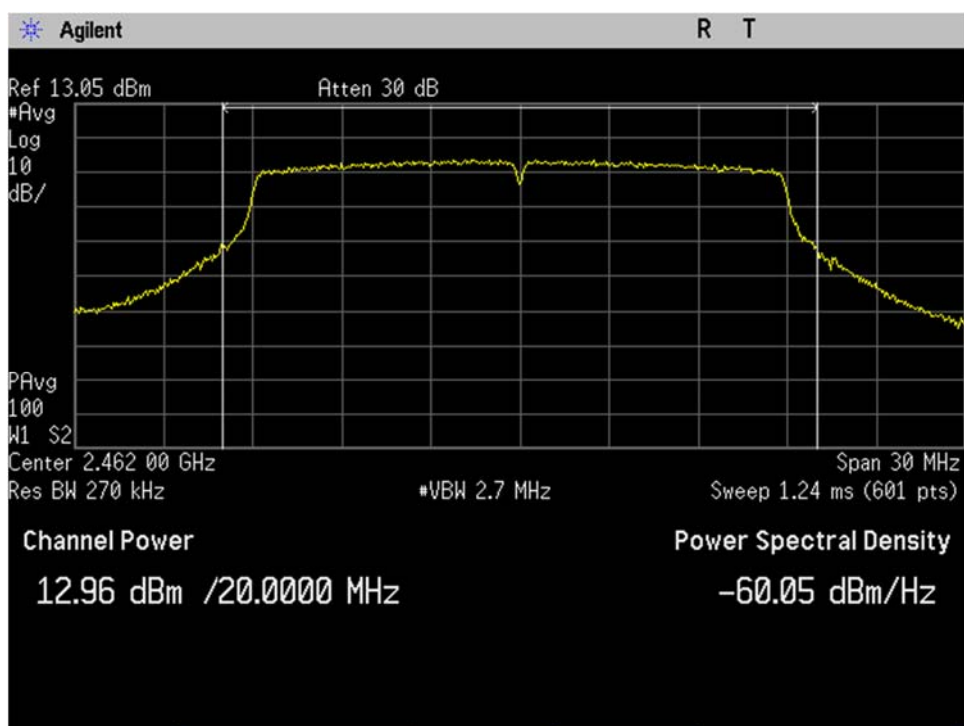
WIFI_High Ch_2462MHz_20MHz BW_n-mode_Output Power_Port 1
