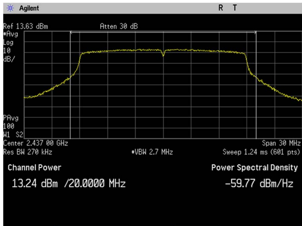
WIFI_Mid Ch_2437MHz_20MHz BW_n-mode_Output Power_Port 1
