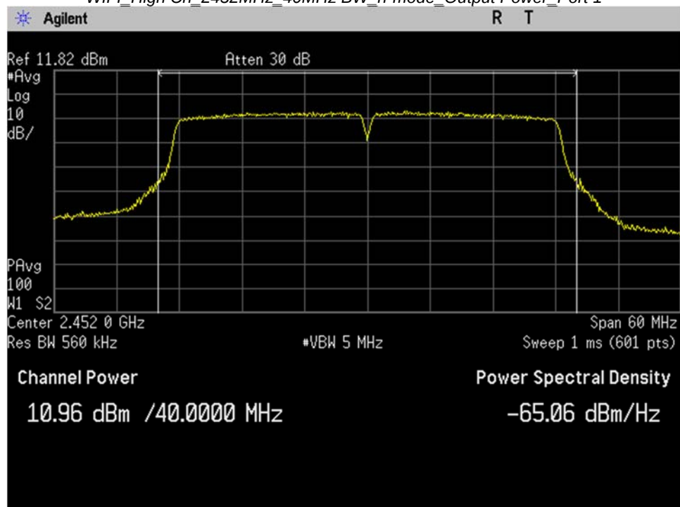
WIFI_High Ch_2452MHz_40MHz BW_n-mode_Output Power_Port 1
