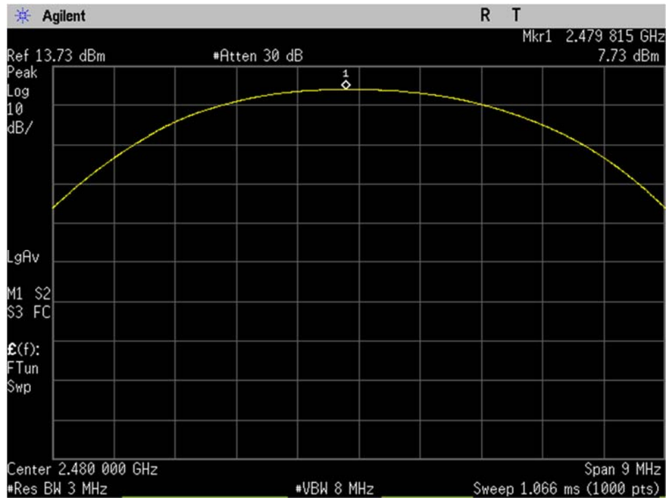
BLE_High Ch_2480MHz_1MBit_Output Power_Port 1
