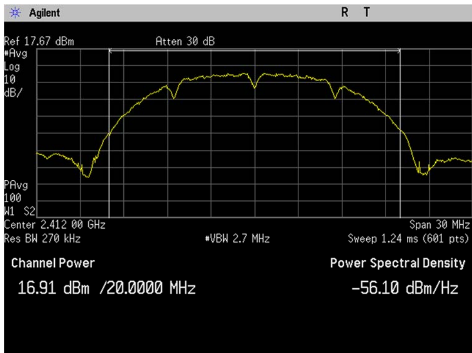
WIFI_Low Ch_2412MHz_20MHz BW_b-mode_Output Power_Port 2
