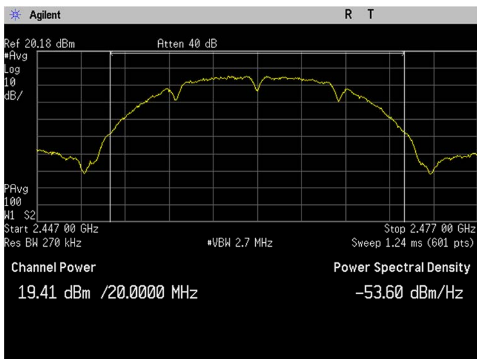
WIFI_High Ch_2462MHz_20MHz BW_b-mode_Output Power_Port 1
