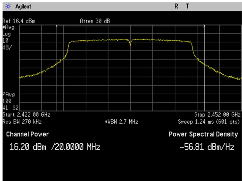
WIFI_Mid Ch_2437MHz_20MHz BW_g-mode_Output Power_Port 1
