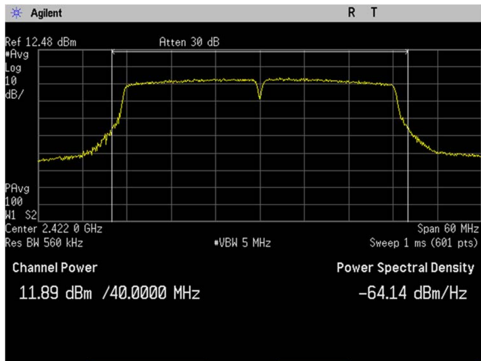
WIFI_Low Ch_2422MHz_40MHz BW_n-mode_Output Power_Port 1
