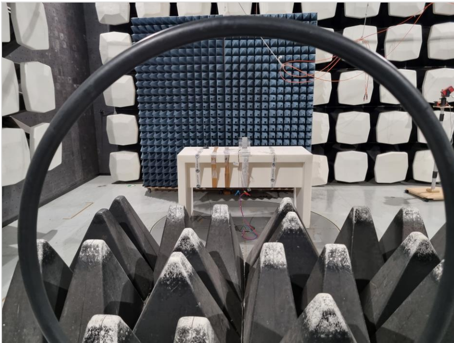
Photograph 1: EUT test setup in the semi anechoic chamber, measurement <30 MHz, overview
