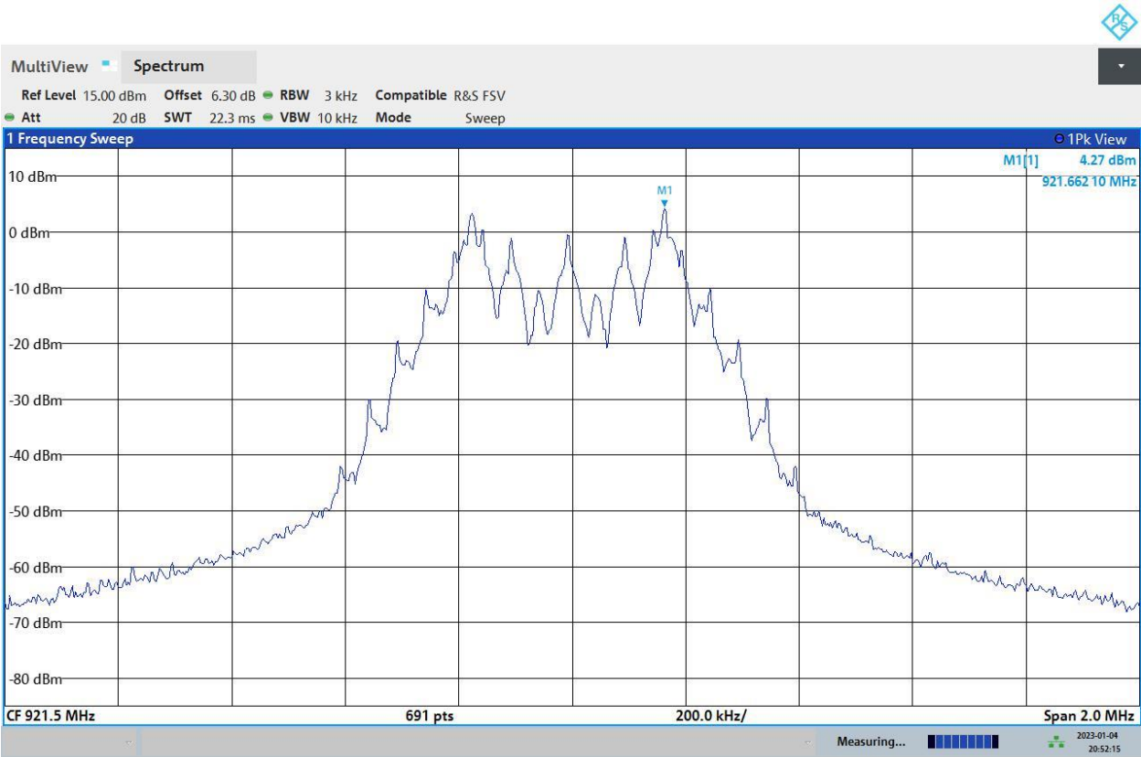
Figure 4: D004_PK-PSD
