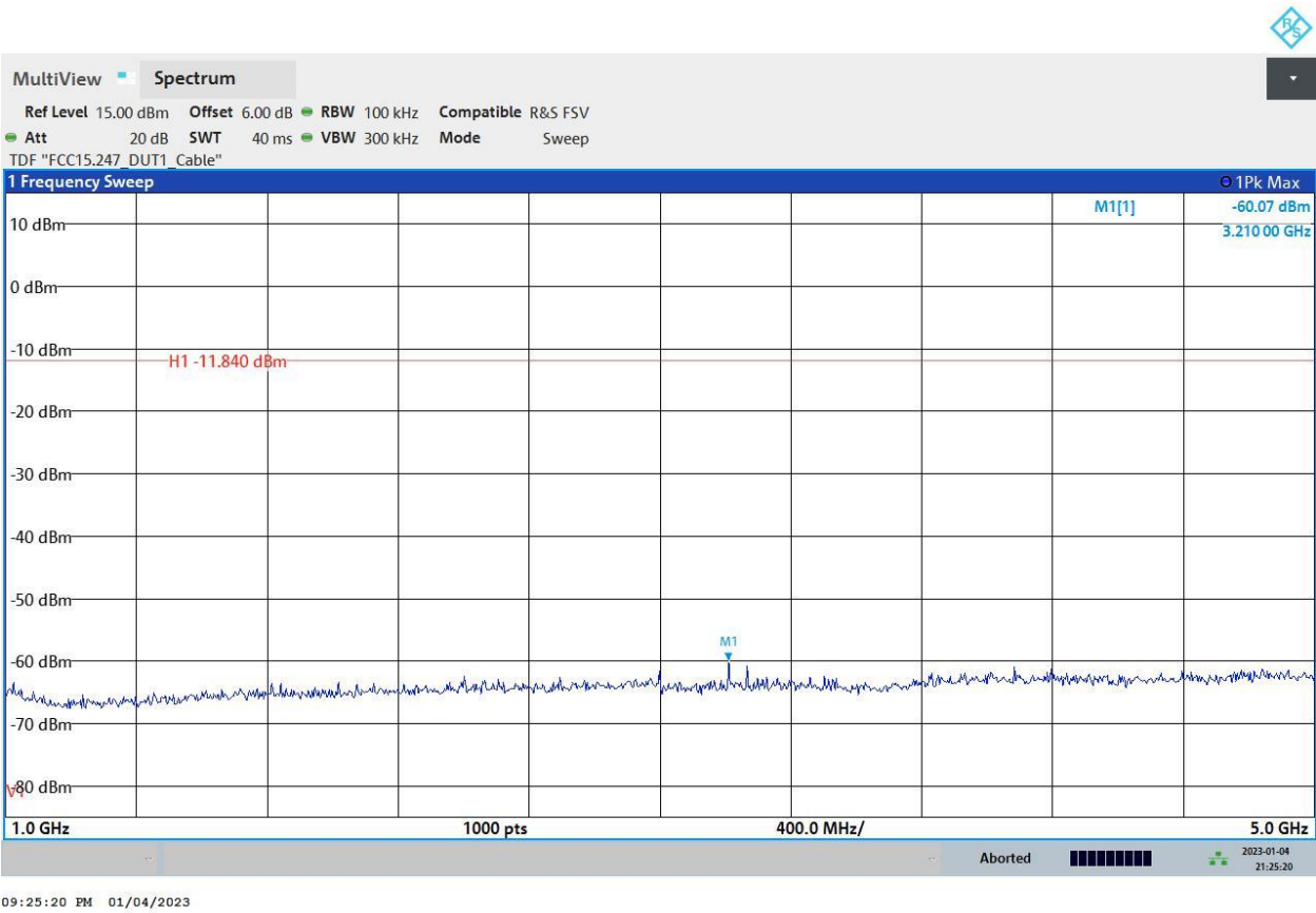
Figure 8: D005_04_sweep_3
