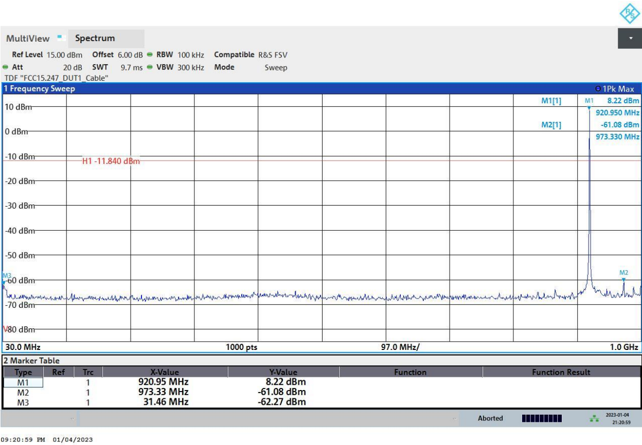
Figure 7: D005_03_sweep_2
