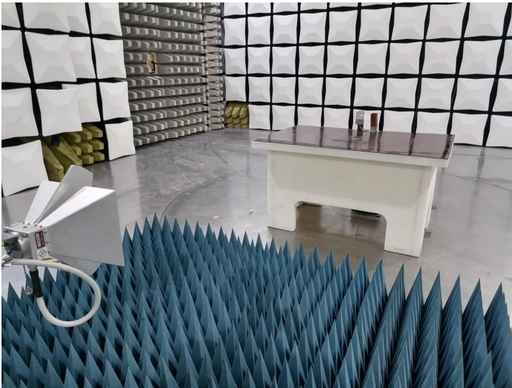
Fig. Mea.: 5 : Radiated Emission Picture1 4.01
