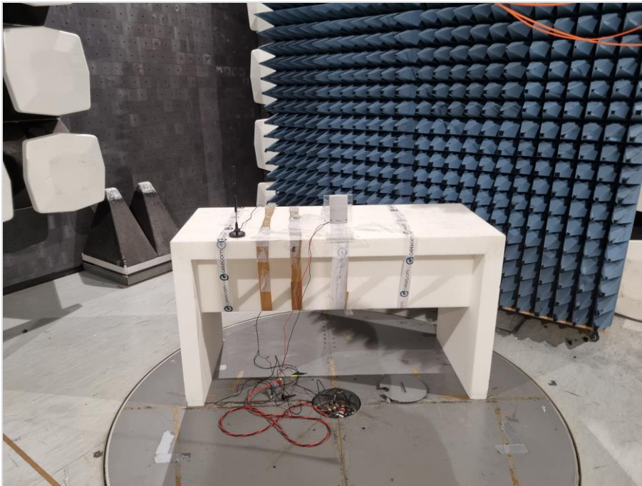
Photograph 3: EUT test setup in the semi anechoic chamber, measurement <1 GHz, close up view, EUT_standing
