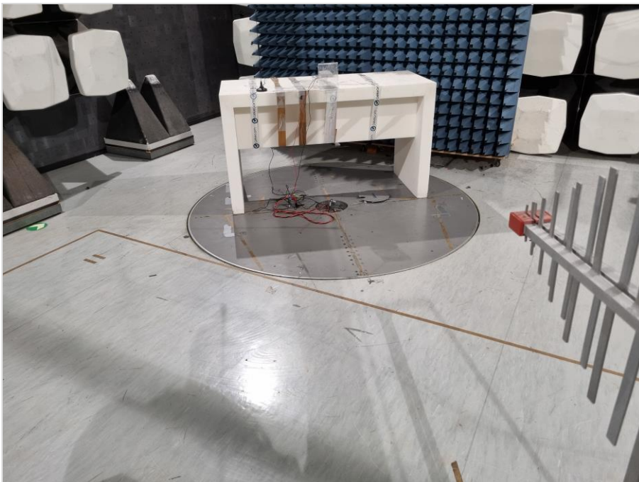
Photograph 4: EUT test setup in the semi anechoic chamber, measurement <1 GHz, overview, EUT_lying
