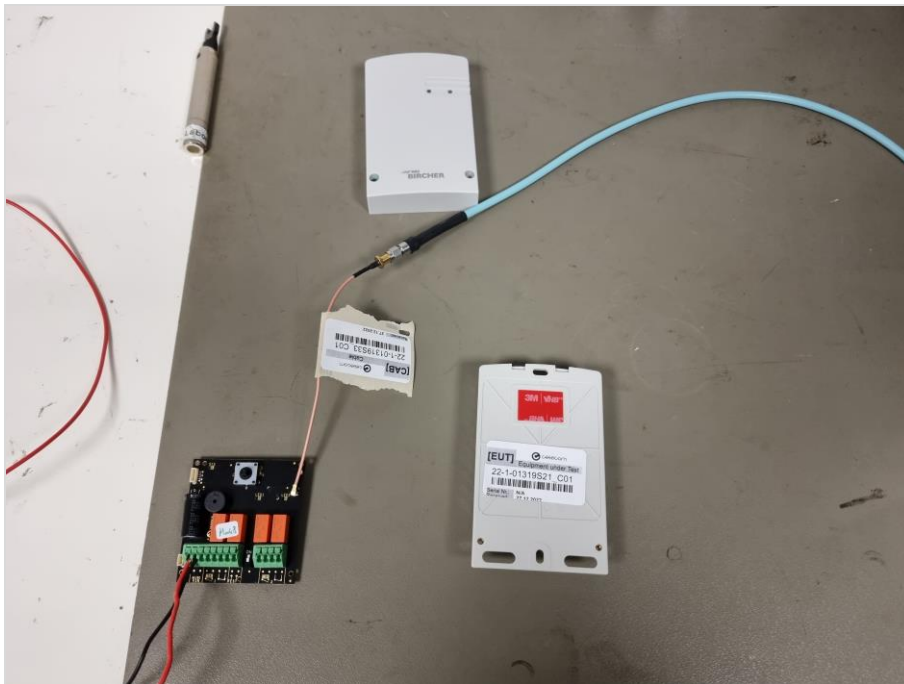
Photograph 7: EUT test setup for conducted measurement, close up view
