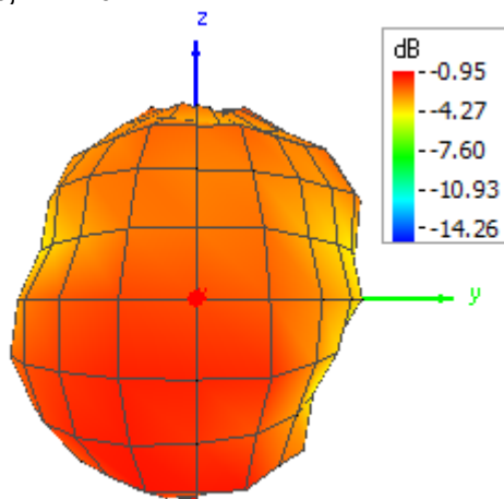
Theta = 90, Phi = 0
