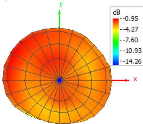
Theta = 0, Phi = 0
