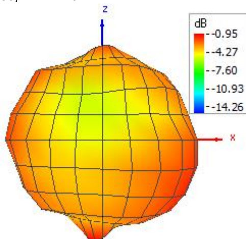
Theta = 90, Phi = 270
