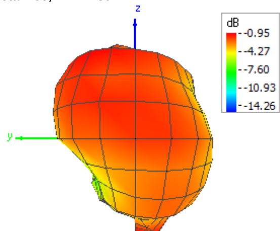
Theta = 90, Phi = 180
