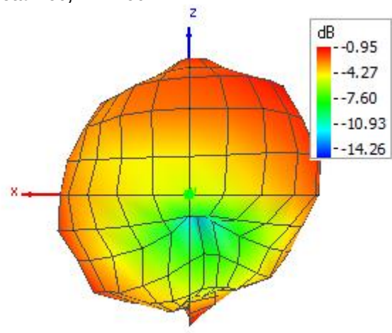
Theta = 90, Phi = 90
