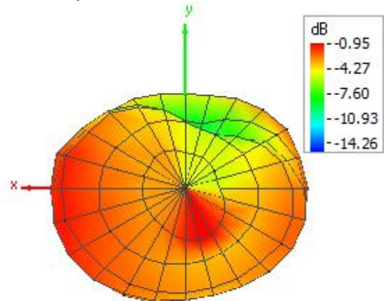
Theta = 180, Phi = 0
