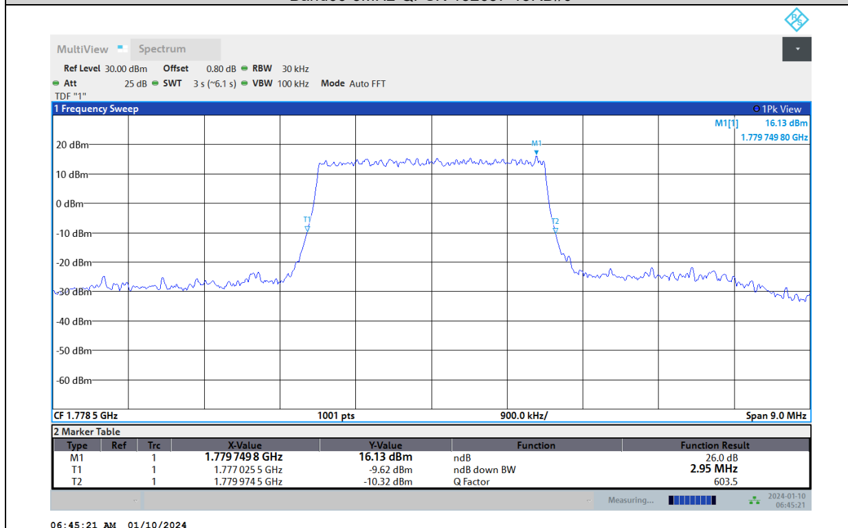
Band66-3MHz-16QAM-131987-15RB#0
