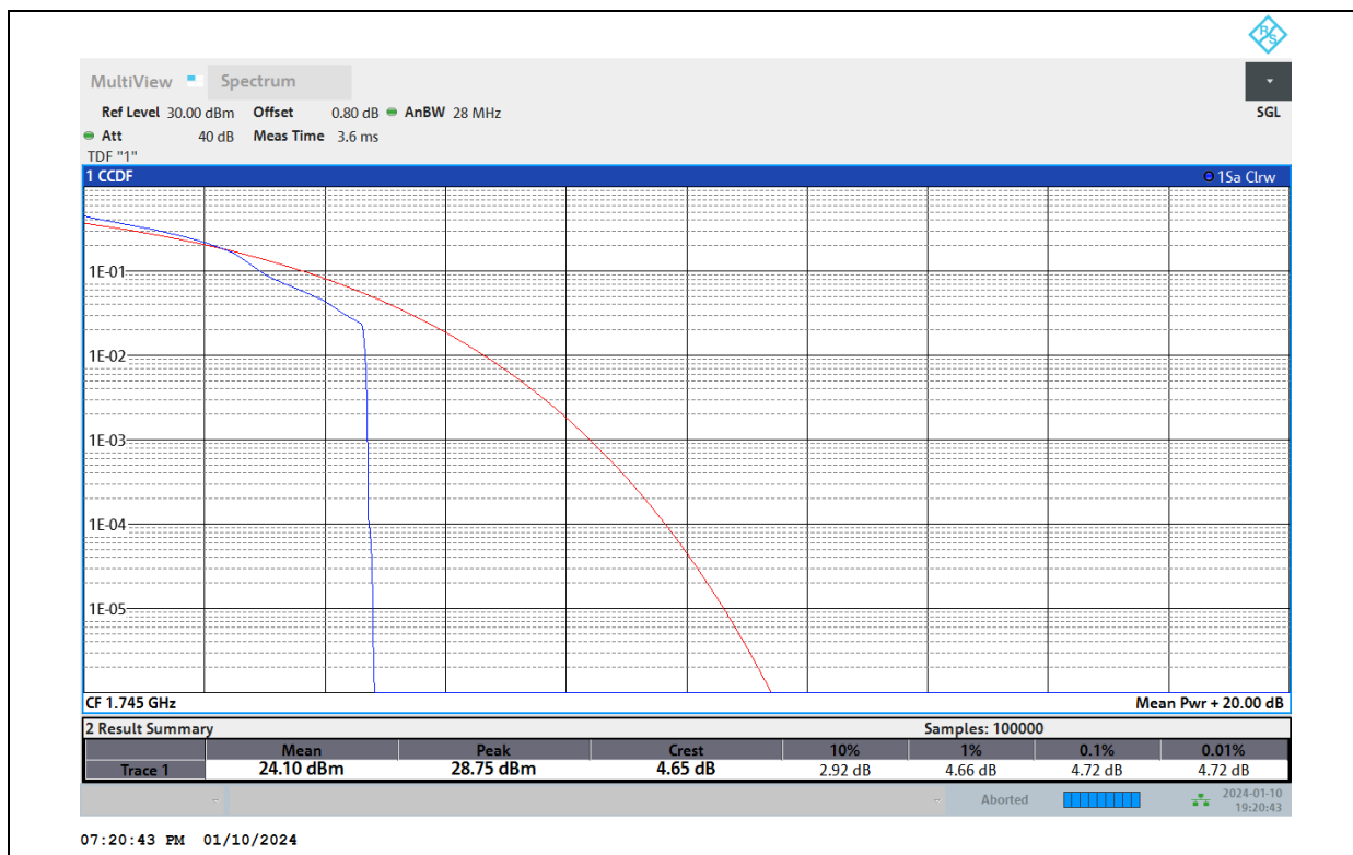
Band66-20MHz-16QAM-132322-100RB#0
