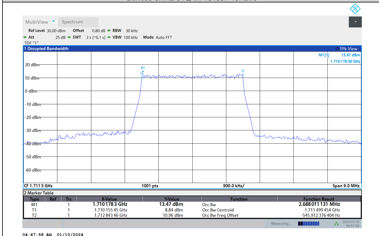
Band66-3MHz-64QAM-132322-15RB#0
