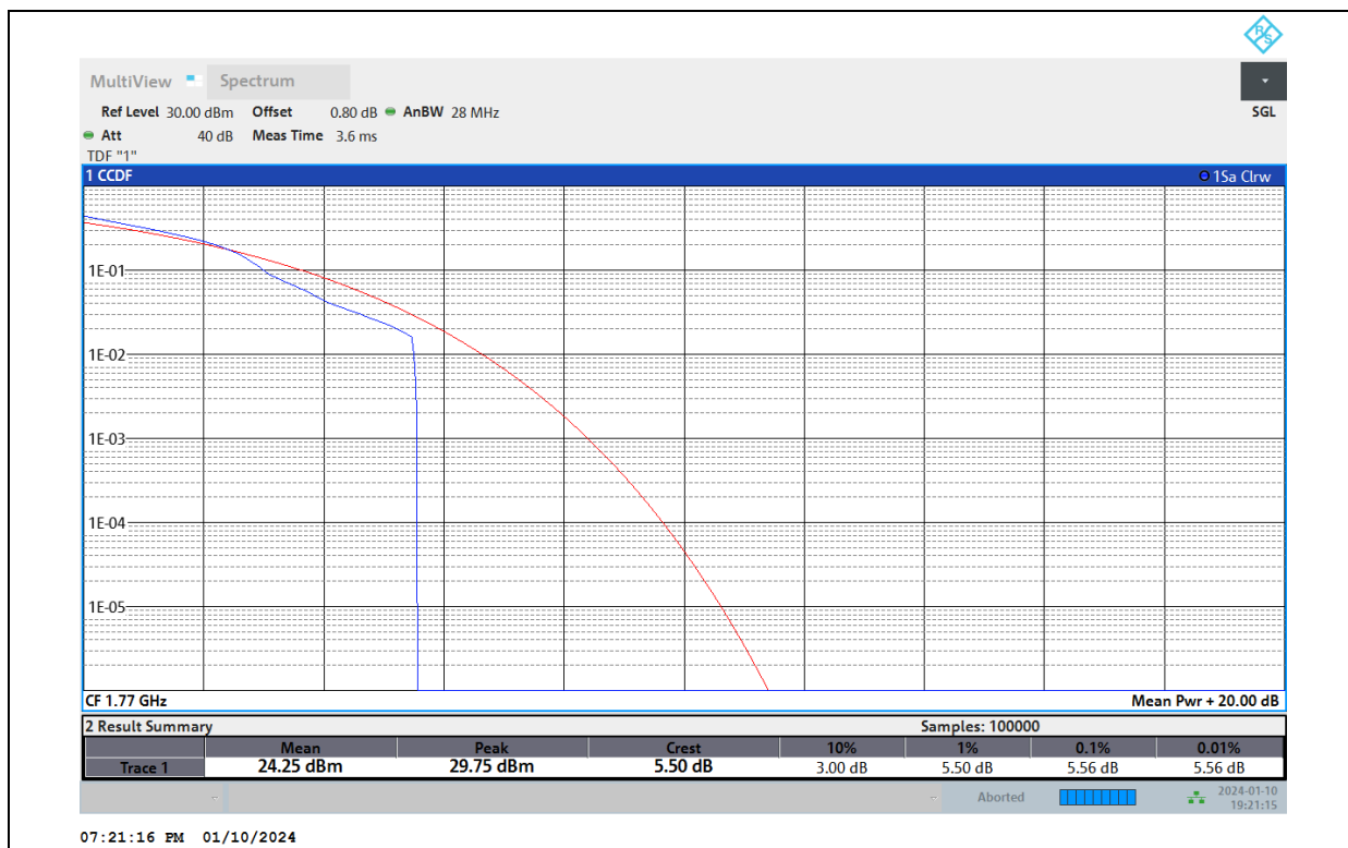
Band66-20MHz-16QAM-132572-100RB#0
