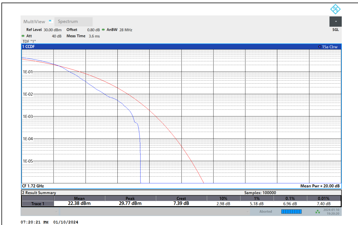
Band66-20MHz-64QAM-132072-100RB#0
