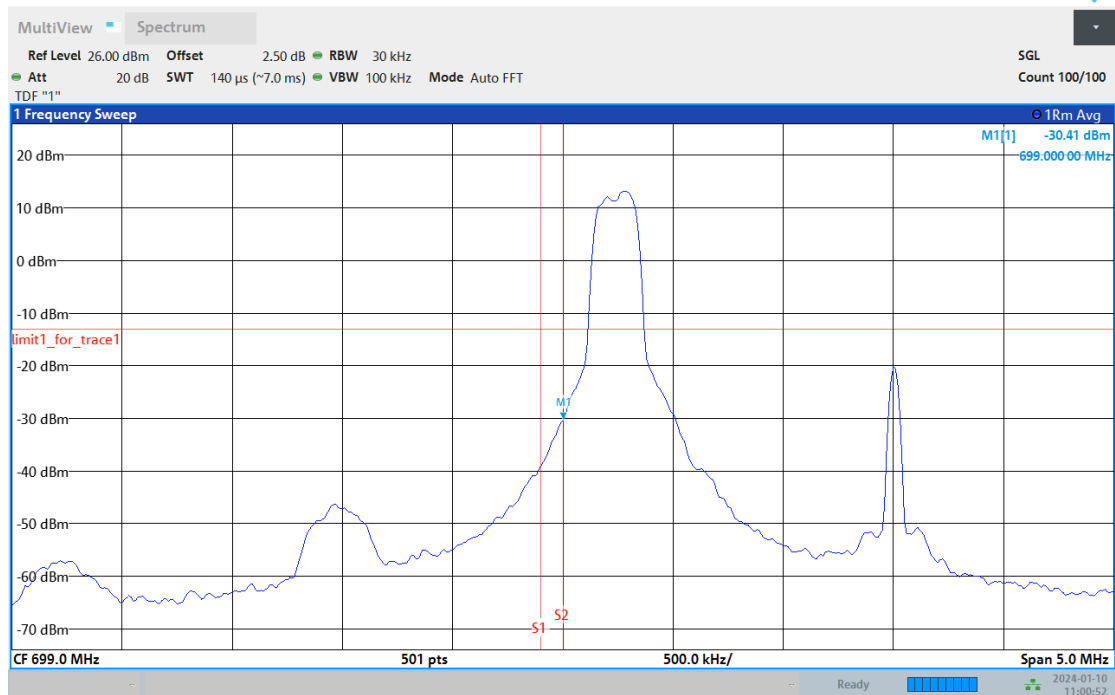
Band12-3MHz-64QAM-23025-15RB#0
