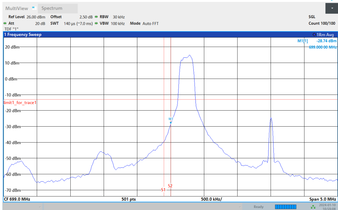
Band12-3MHz-16QAM-23025-15RB#0
