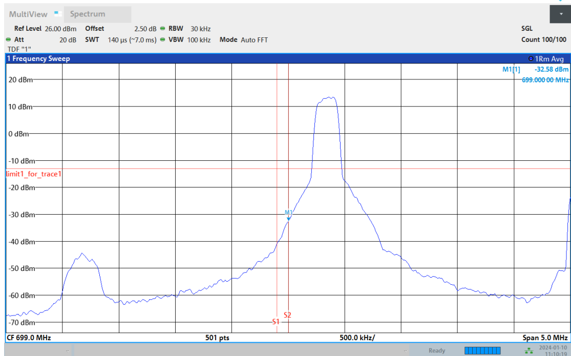
Band12-5MHz-16QAM-23035-25RB#0
