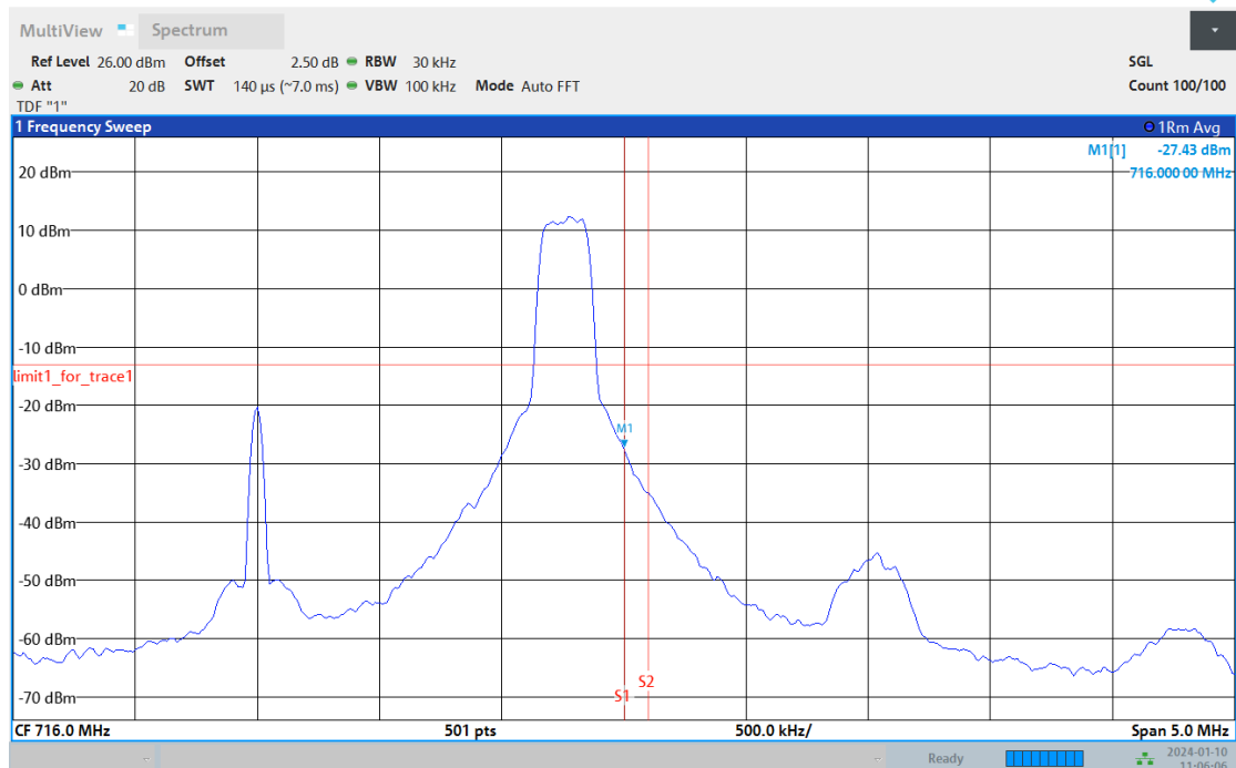
Band12-3MHz-64QAM-23165-15RB#0
