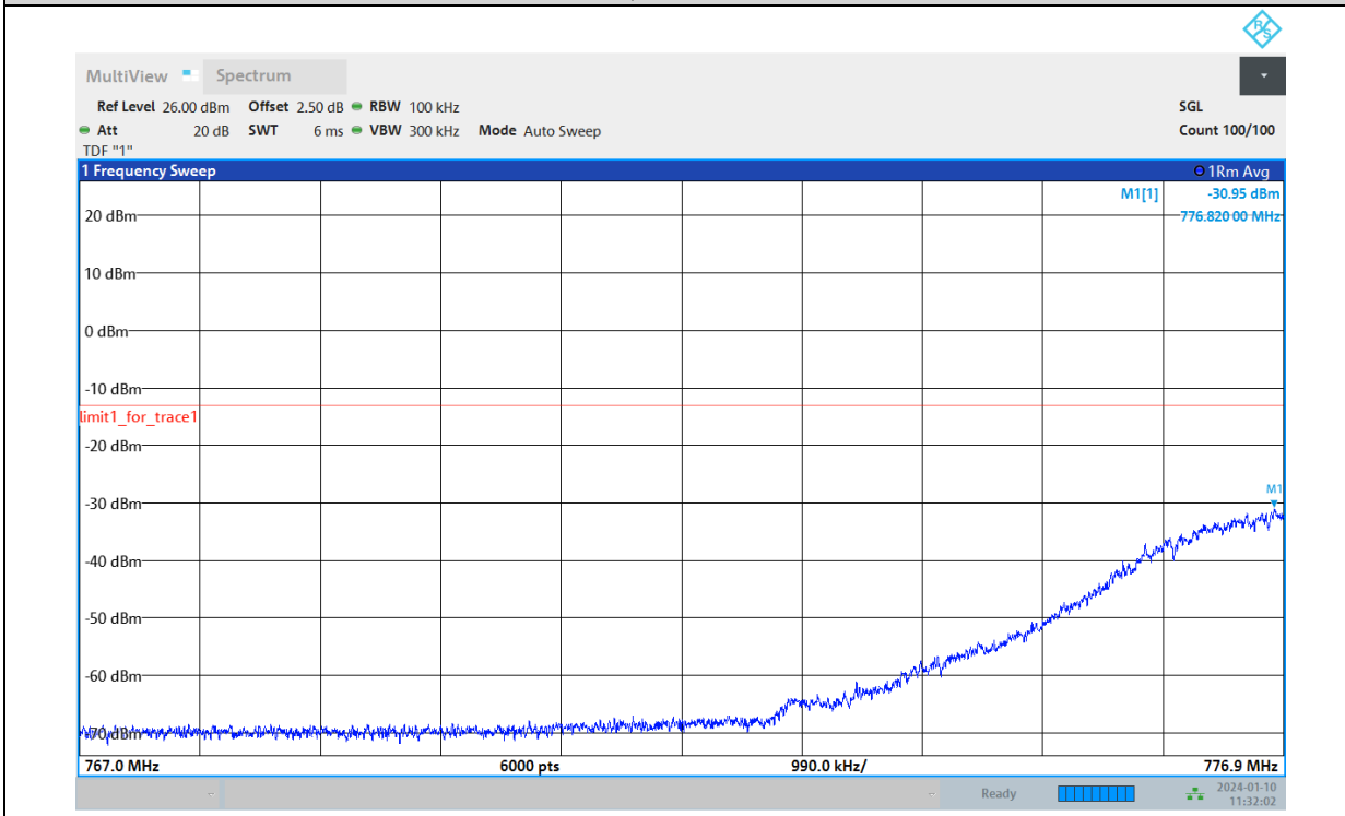
Band13-5MHz-QPSK-23205-25RB#0-P2
