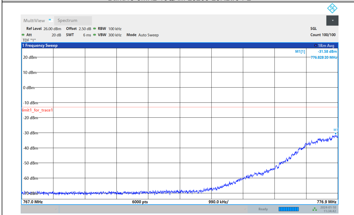
Band13-5MHz-16QAM-23205-25RB#0-P2
