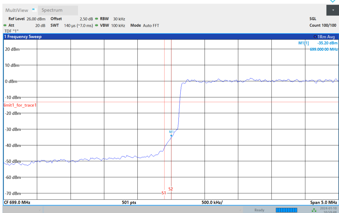
Band12-3MHz-16QAM-23165-1RB#14
