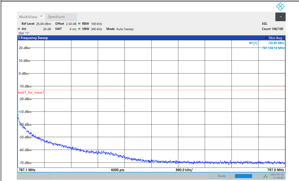
Band13-5MHz-QPSK-23255-1RB#24-P2
