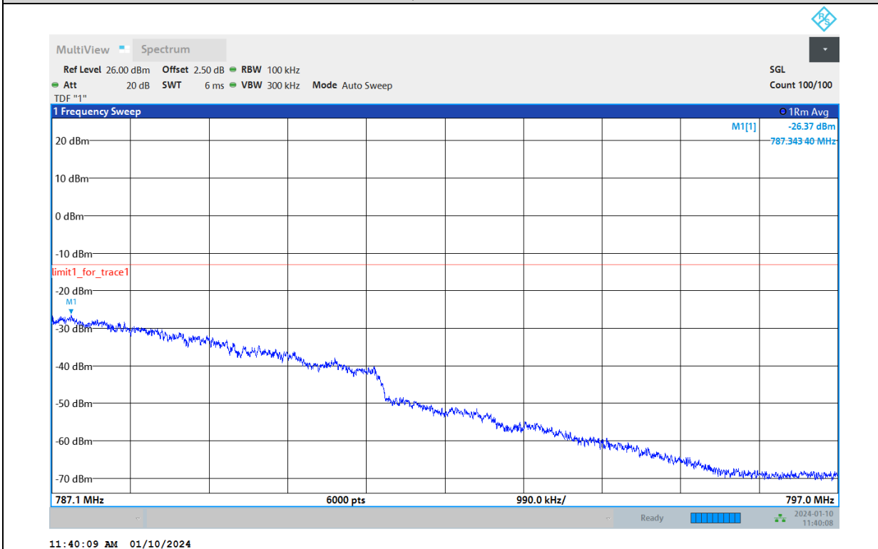
Band13-5MHz-16QAM-23255-1RB#24-P1
