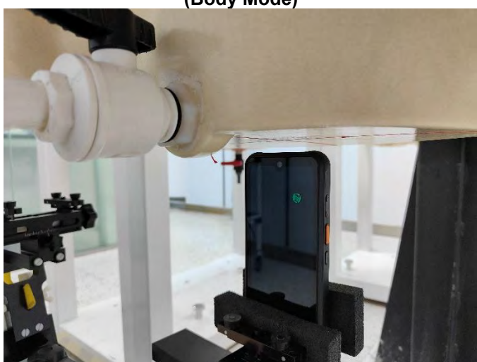
Top Side of EUT with 1 cm Gap (Body Mode)
