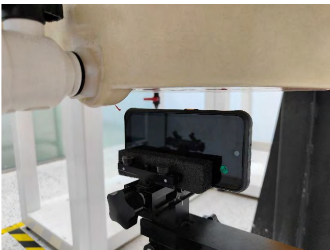
Left Side of EUT with 2.4 cm Gap (Body Mode)
