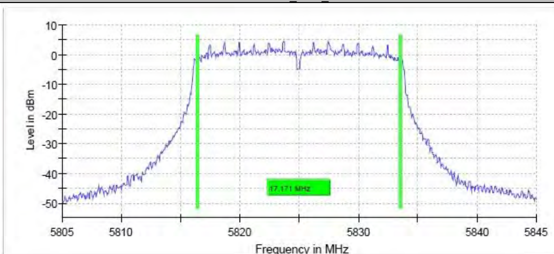
11AC20-MIMO_Ant6_5825
