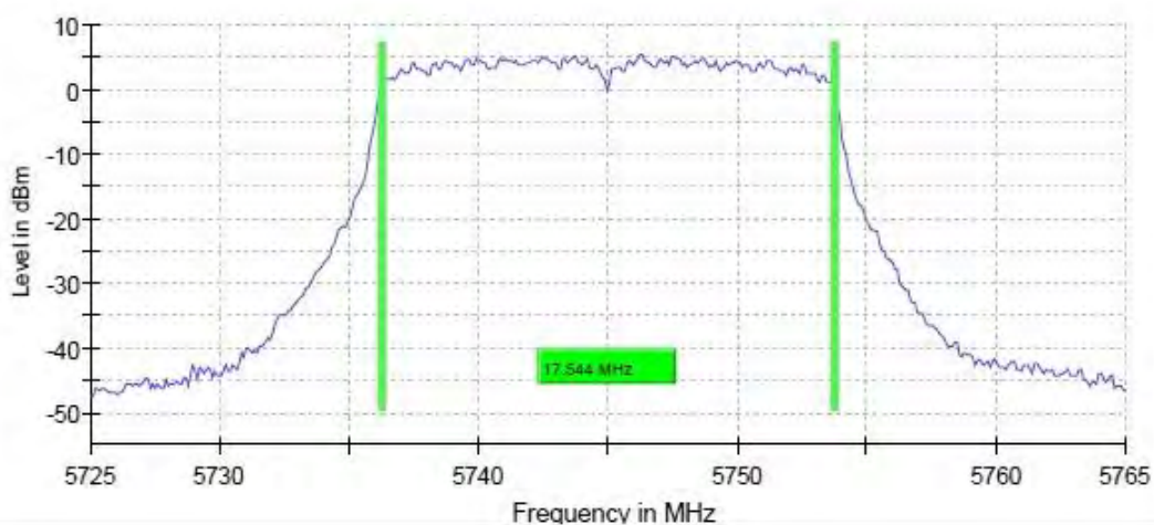
11AC20_Ant6_5745
