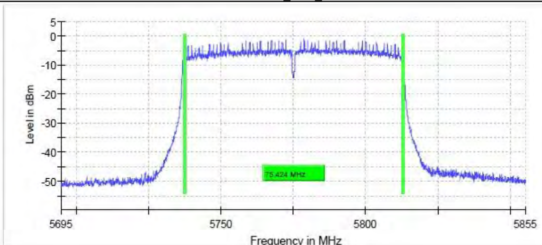
11AC80-MIMO Ant6 5775
