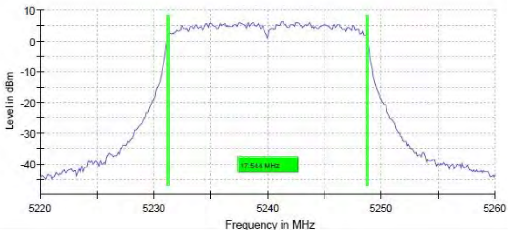
11AC20_Ant6_5240
