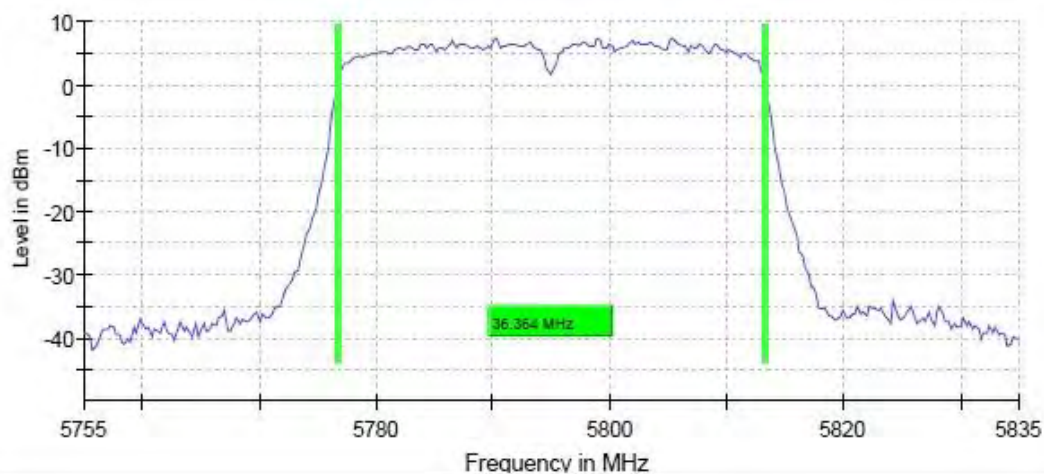
11AC40_Ant6_5795
