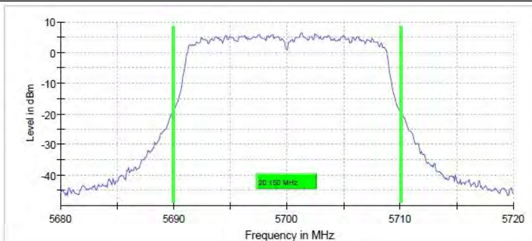
11AC20_Ant6_5700
