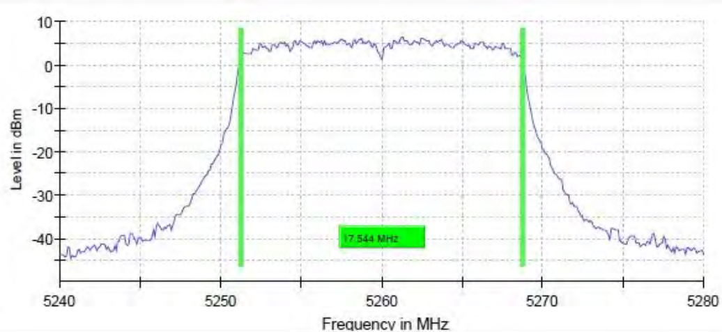
11AC20_Ant6_5260
