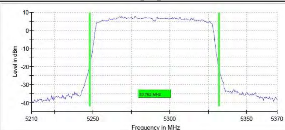
11AC80_Ant6_5290
