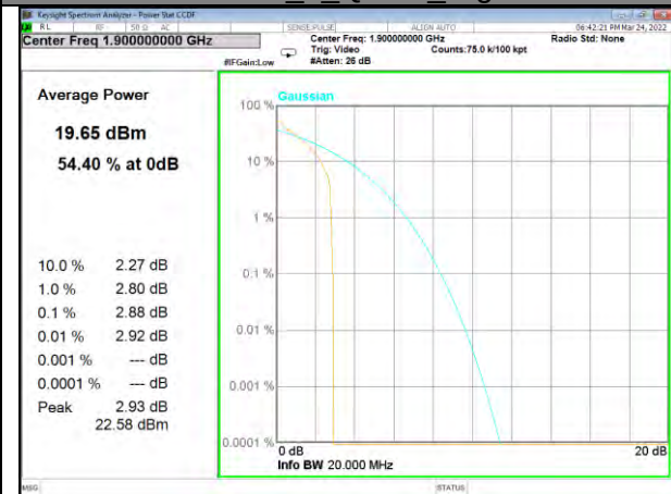
Band 2_1_Q16_High
