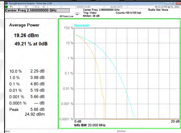
Band 7_100_Q16_High
