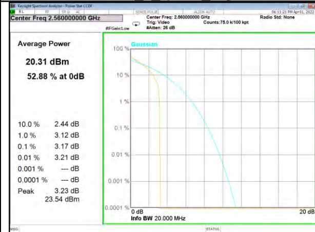
Band 7_1_Q16_High
