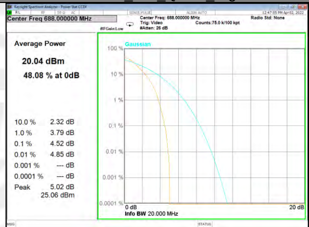
Band 71_100_Q16_High
