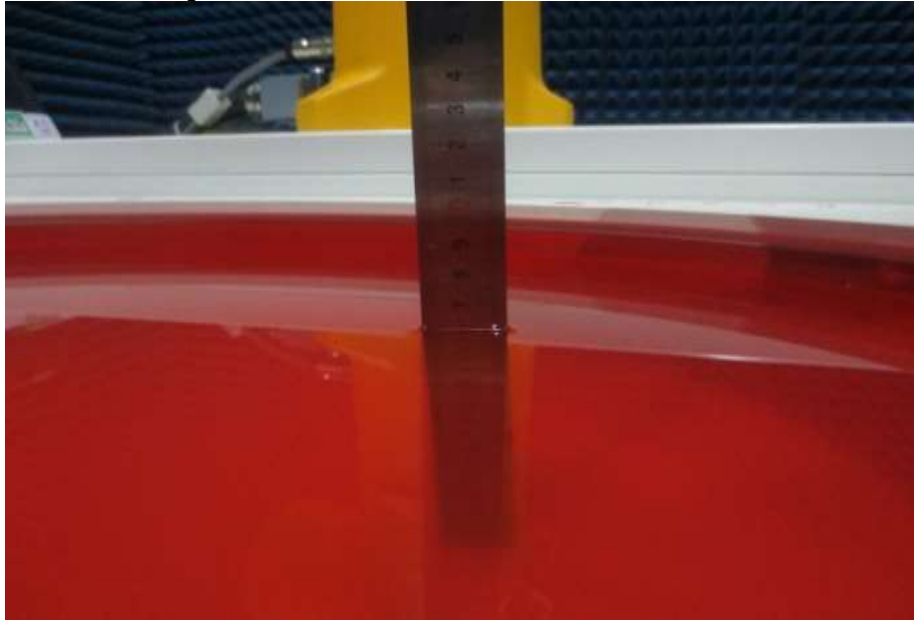
Fig. 9.2 Photo of Liquid Height for Body SAR of ELI V5.0 (850MHz) (depth>15cm)
