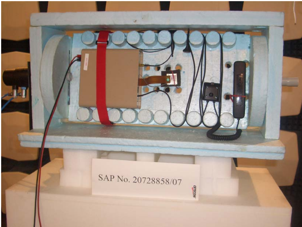
Photograph 6: Measurements in the anechoic chamber, test set-up
