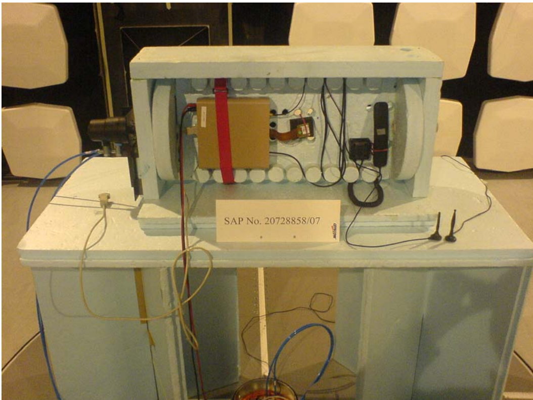
Photograph 5: Measurements in the anechoic chamber, test set-up (front view of test set-up)
