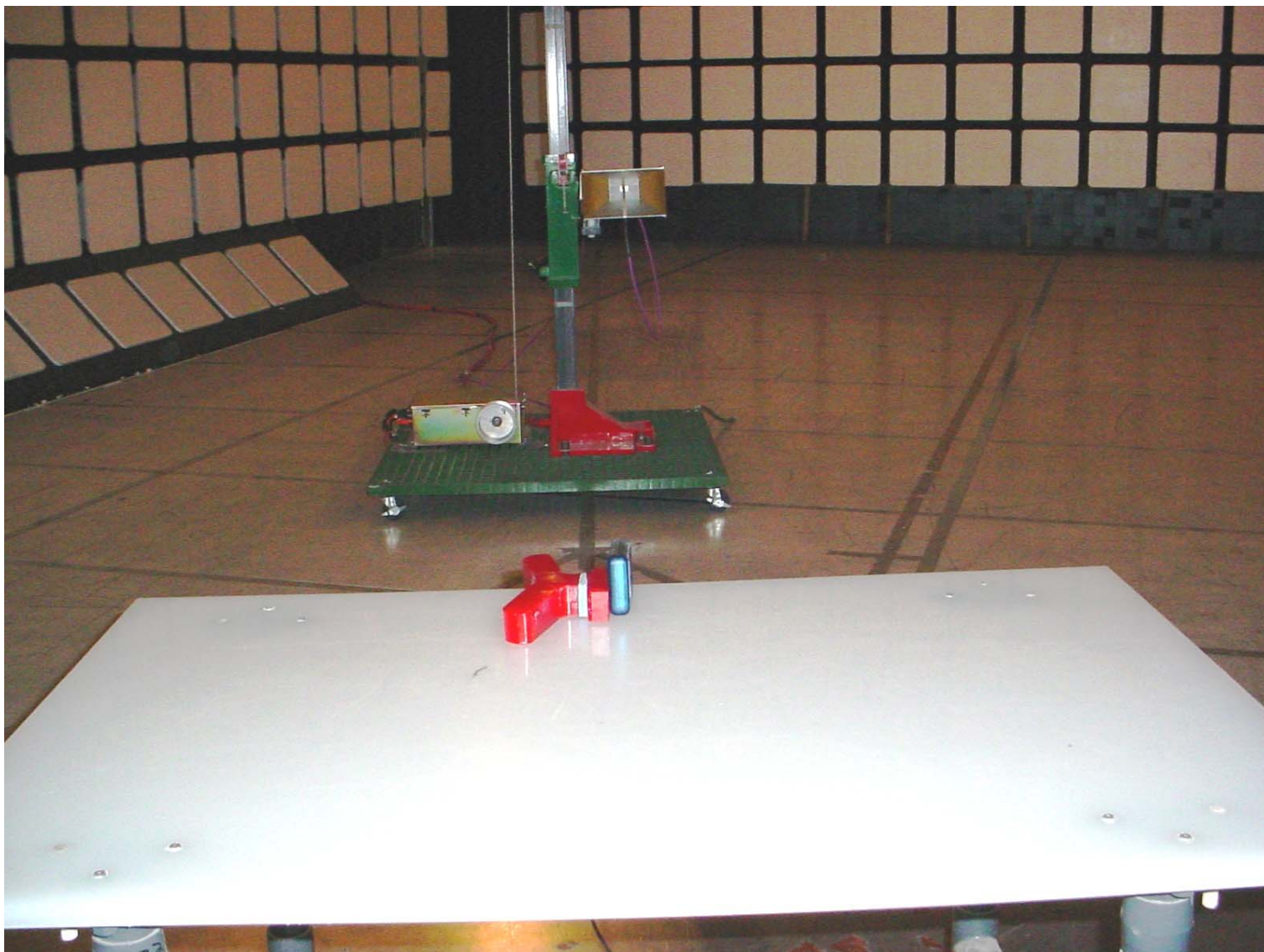
Photo #3: Radiated Emissions, Orthogonal Position #2
