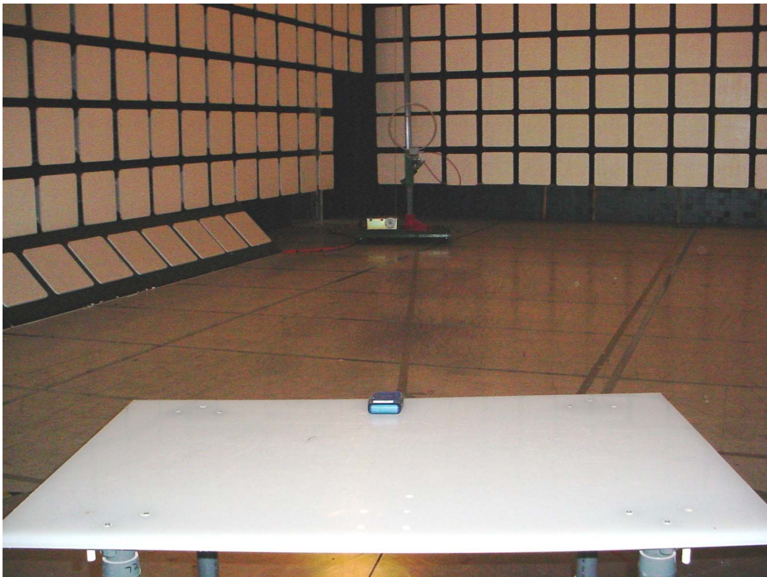
Photo #4: Radiated Emissions, Orthogonal Position #3
