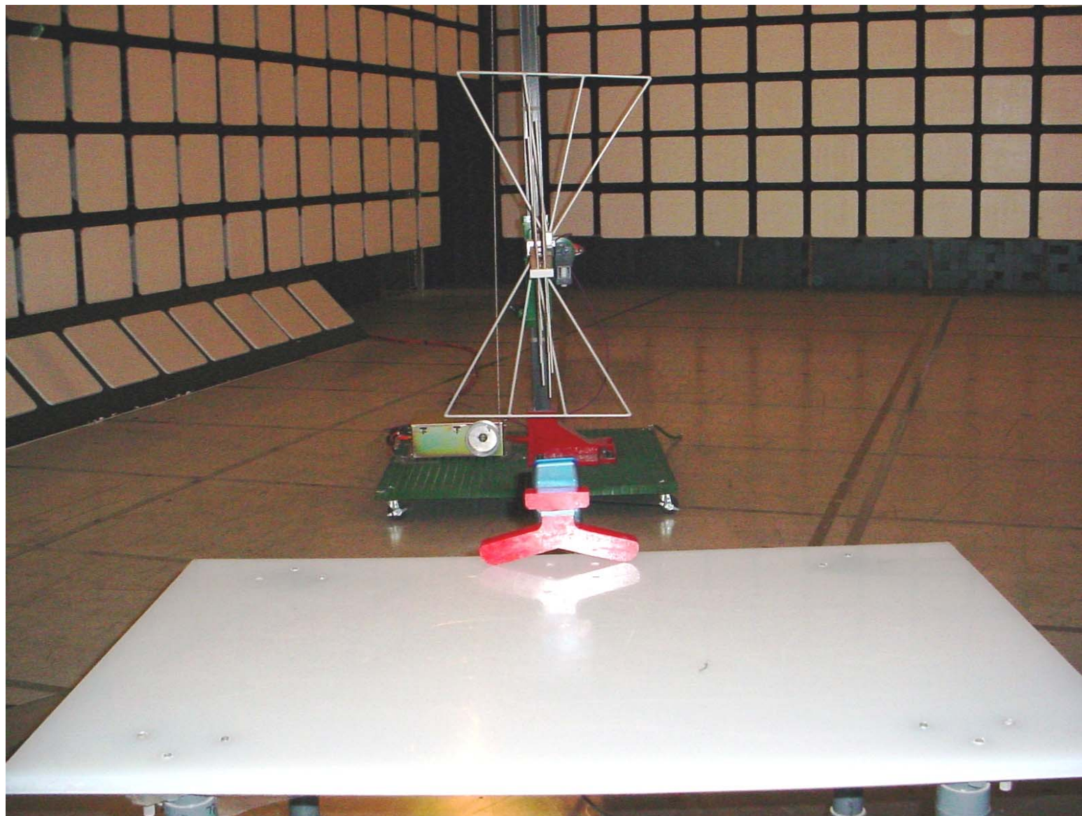
Photo #2: Radiated Emissions, Orthogonal Position #1
