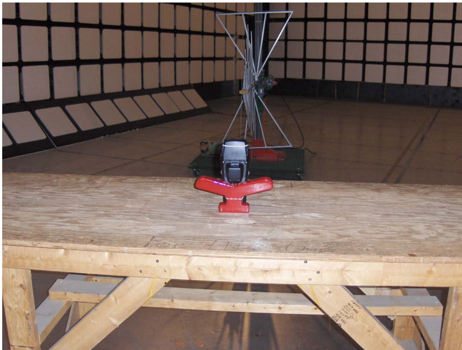
Photo #3: Radiated Emissions, Orthogonal Position #3
