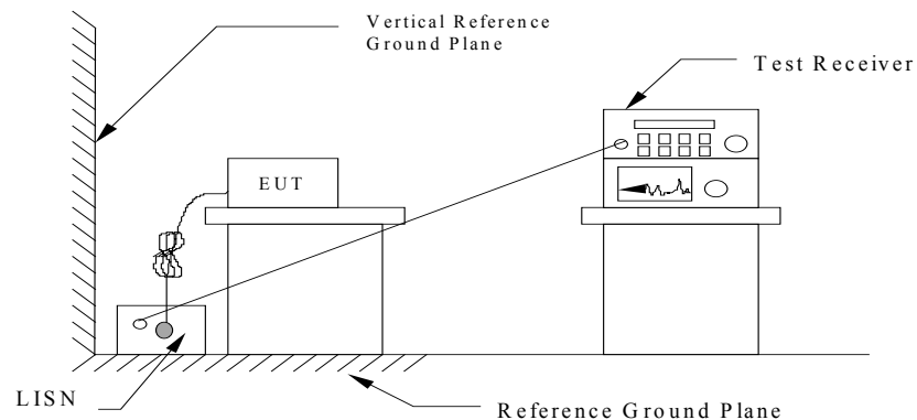
Figure 3 : Conducted emissions measurement configuration
