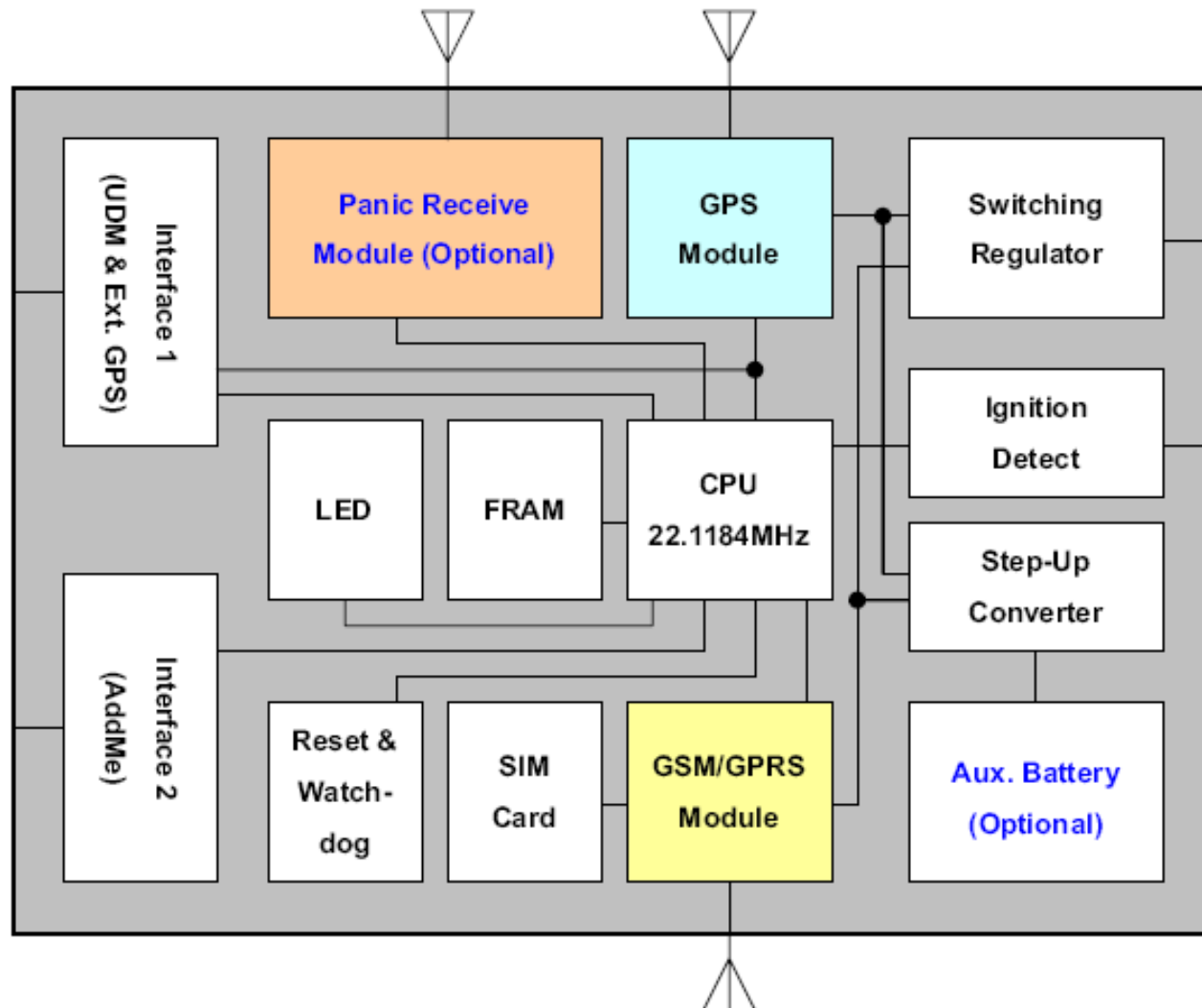
Speedy Block Diagram
