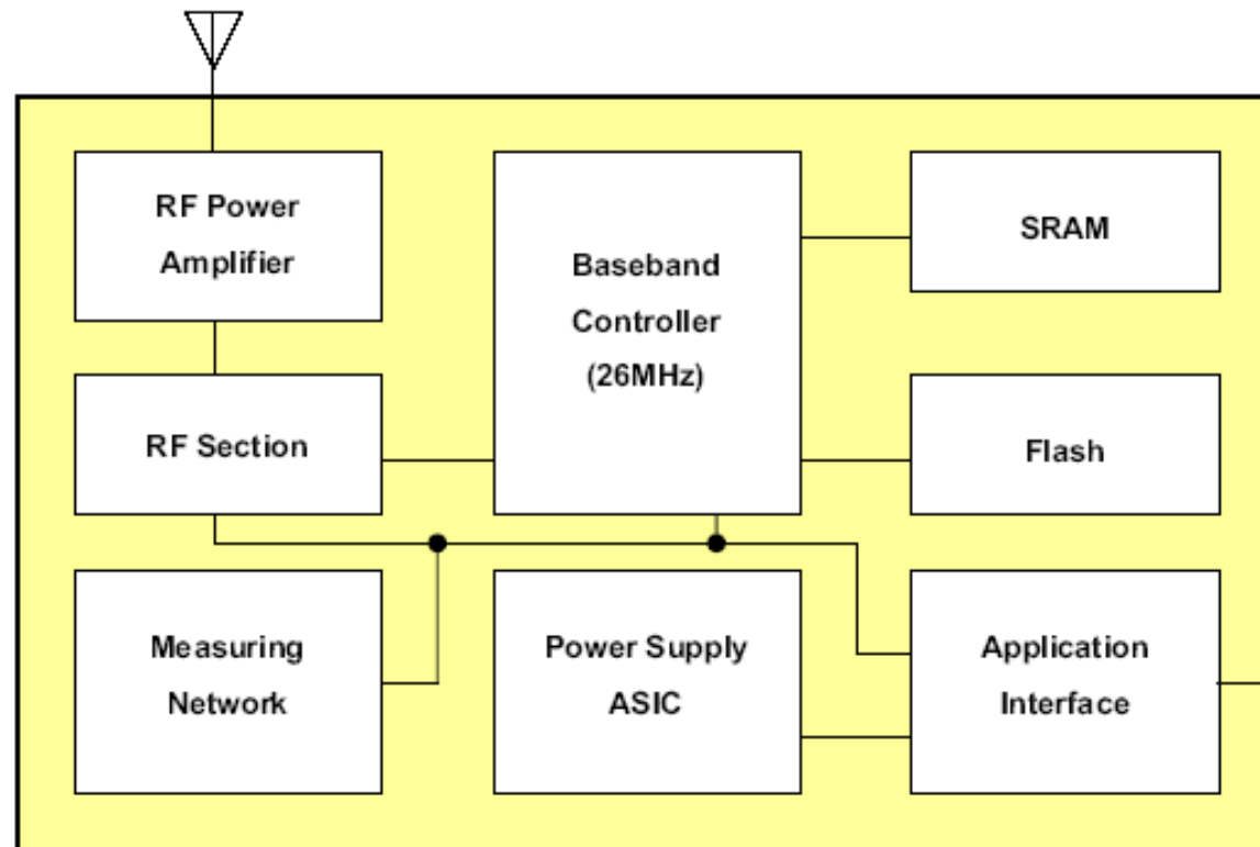
GSM/GPRS Module Block Diagram
