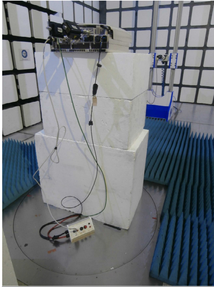
Radiated Emissions 18 GHz to 22 GHz
