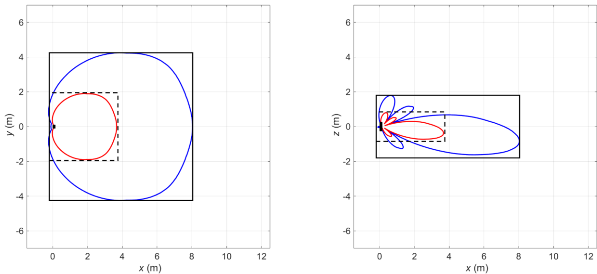
Figure 5 Compliance boundaries for general public (black solid line) and occupational (black dashed line) exposure for the USA and markets where the FCC exposure limits apply. The blue solid lines correspond to compliance distance results for general public exposure obtained using the spherical models. The solid red lines indicate the corresponding compliance distance results for occupational exposure. The EUT is shown from above (left) and from the side (right) with its backplane located at x = 0 m. Mode: B77D (NR). Total time-averaged power delivered to the antenna: 75.5 W.
