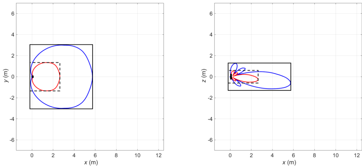
Figure 3 Compliance boundaries for general public (black solid line) and occupational (black dashed line) exposure for the USA and markets where the FCC exposure limits apply. The blue solid lines correspond to compliance distance results for general public exposure obtained using the spherical models. The solid red lines indicate the corresponding compliance distance results for occupational exposure. The EUT is shown from above (left) and from the side (right) with its backplane located at x = 0 m. Mode: B77D (NR). Total time-averaged power delivered to the antenna: 37.8 W.
