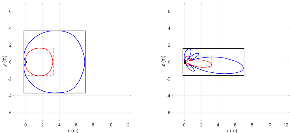
Figure 4 Compliance boundaries for general public (black solid line) and occupational (black dashed line) exposure for the USA and markets where the FCC exposure limits apply. The blue solid lines correspond to compliance distance results for general public exposure obtained using the spherical models. The solid red lines indicate the corresponding compliance distance results for occupational exposure. The EUT is shown from above (left) and from the side (right) with its backplane located at x = 0 m. Mode: B77D (NR). Total time-averaged power delivered to the antenna: 56.7 W.
