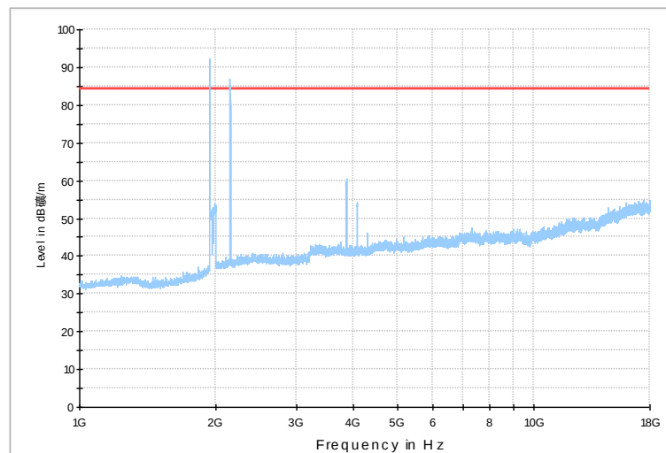
RSE_Erison_1-18G_FCC
