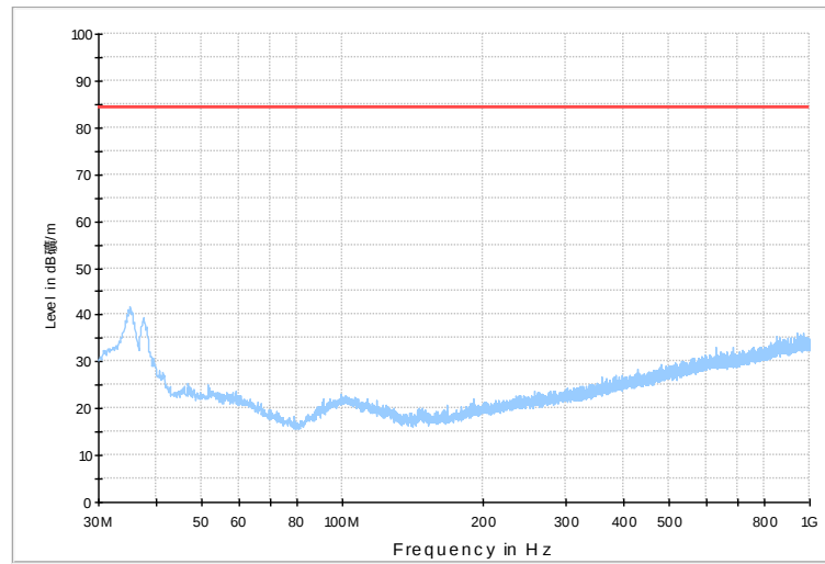
RSE_Erison_30M-1G_FCC
