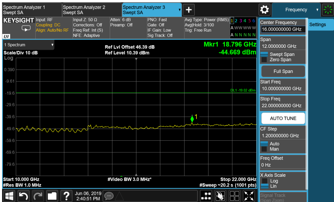
Configuration WCDMA+NB-IoT-MC-2 (1WCDMA 64QAM+2SA QPSK)
