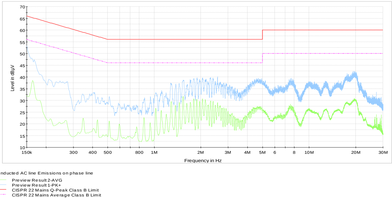
Plot 8.3-1: Conducted emissions on phase line
