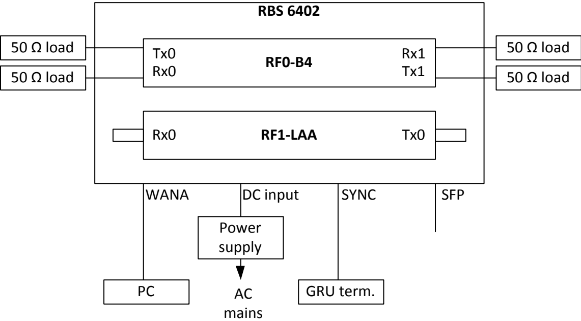
Figure 3.6-1: Setup diagram
