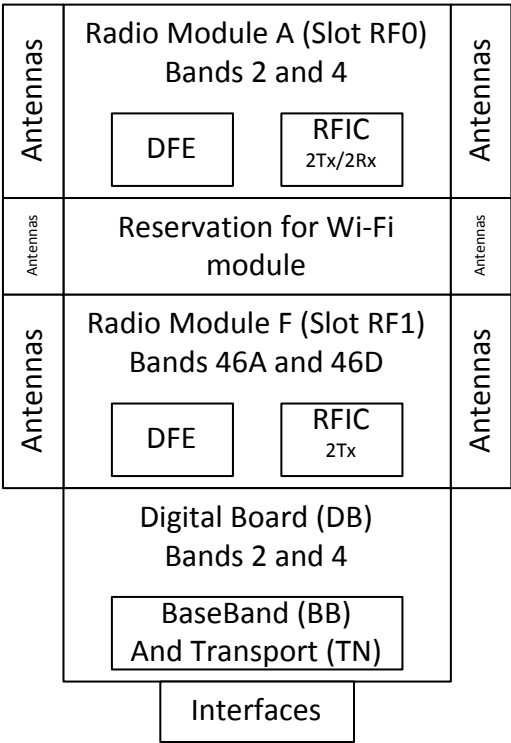
Figure 3.4-1: RBS 6402 block diagram (KRD 901 060/83), Wi-Fi module was not assembled in the tests
