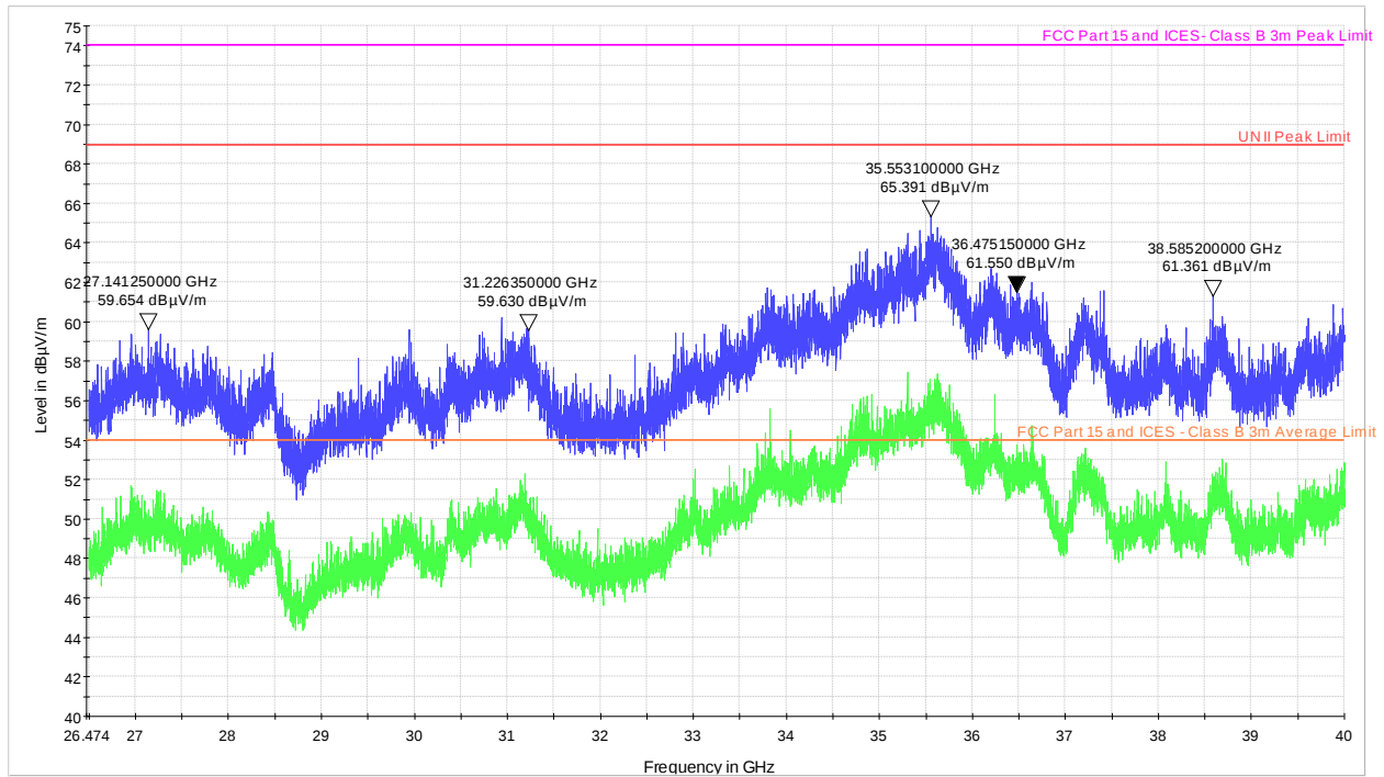
Figure 8.2-11: Radiated spurious emissions within 26.5–40 GHz, mid channel
