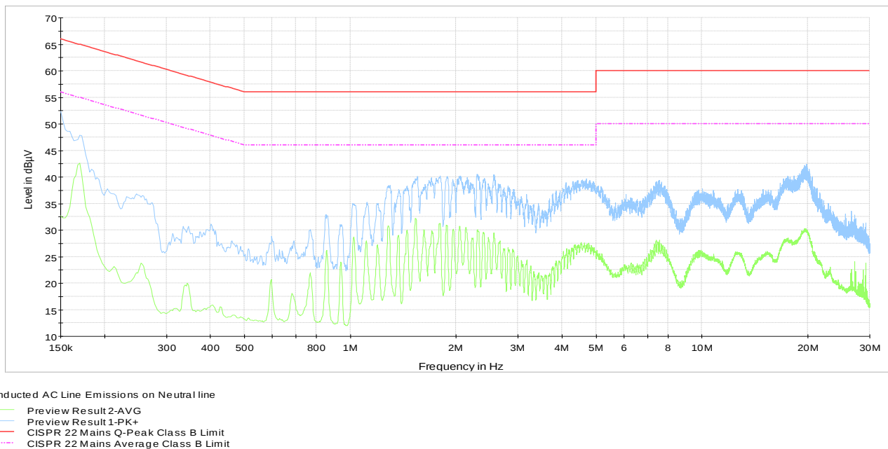
Plot 8.3-2: Conducted emissions on neutral line
